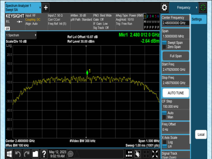
2DH5-Ant1-2480-0~Reference
