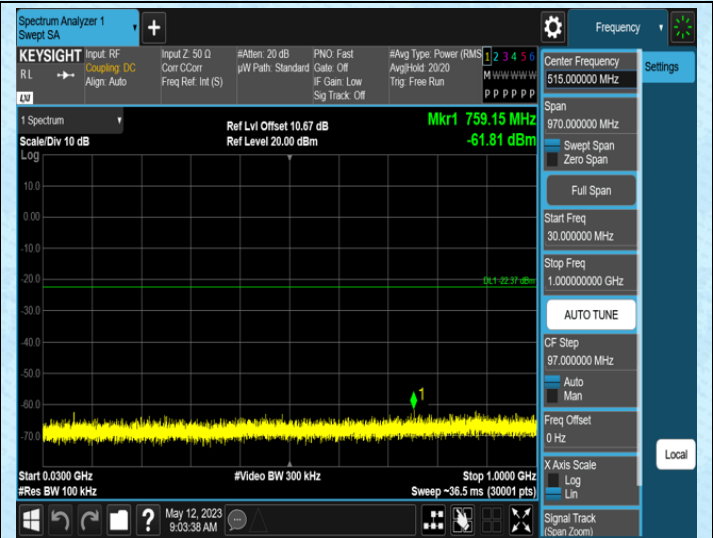
3DH5-Ant1-2402-30~1000
