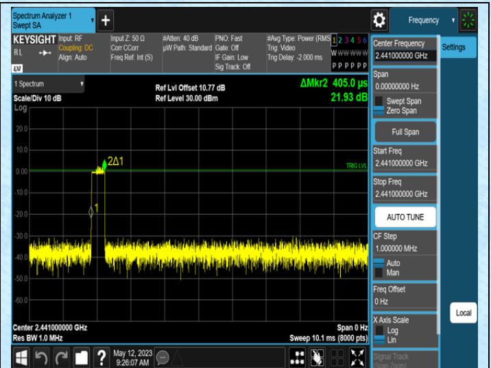
3DH1-Ant1-Hop
