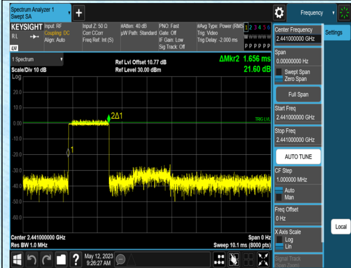
3DH3-Ant1-Hop
