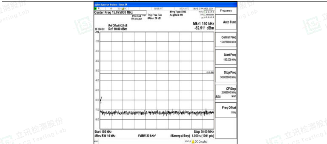
Band2-15MHz-16QAM-18675-1RB#0-0.15~30-PASS
