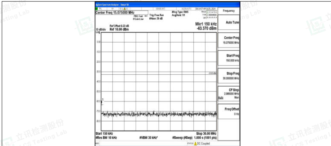
Band2-10MHz-QPSK-19150-1RB#0-0.15~30-PASS
