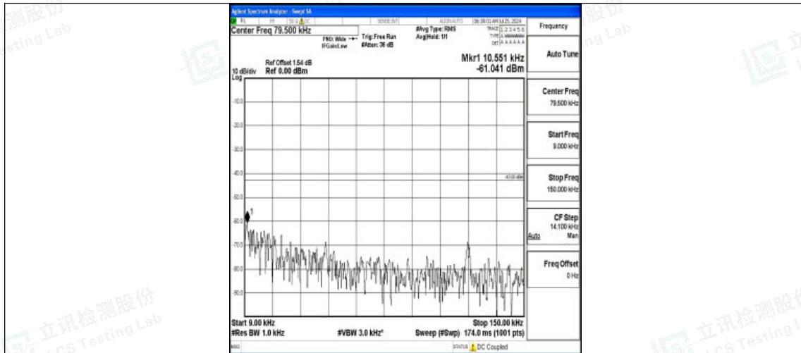
Band2-15MHz-QPSK-18675-1RB#0-0.009~0.15-PASS
