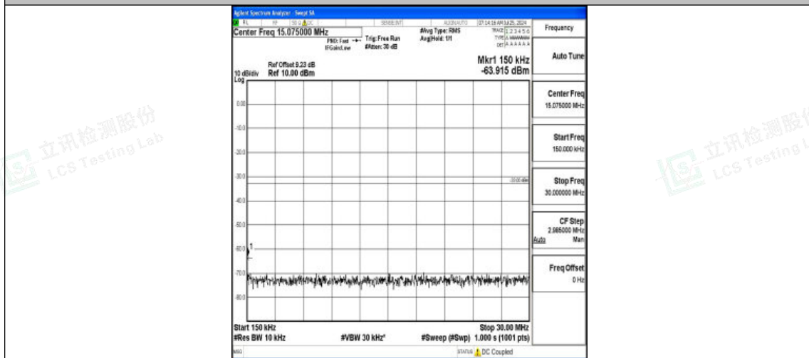
Band2-20MHz-QPSK-18900-1RB#0-0.15~30-PASS
