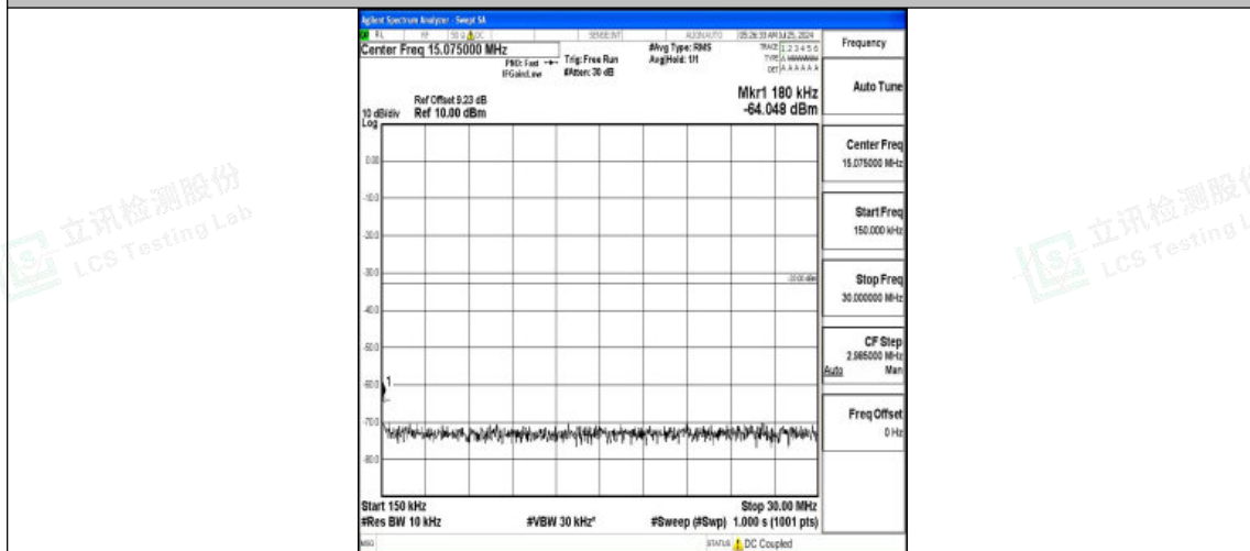
Band2-3MHz-QPSK-18900-1RB#0-0.15~30-PASS
