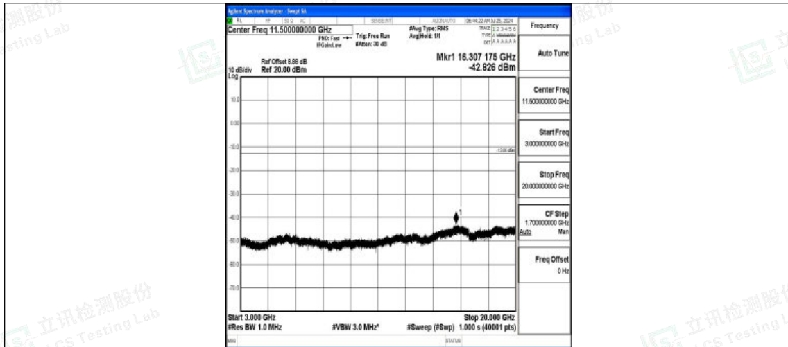
Band2-15MHz-QPSK-19125-1RB#0-3000~20000-PASS
