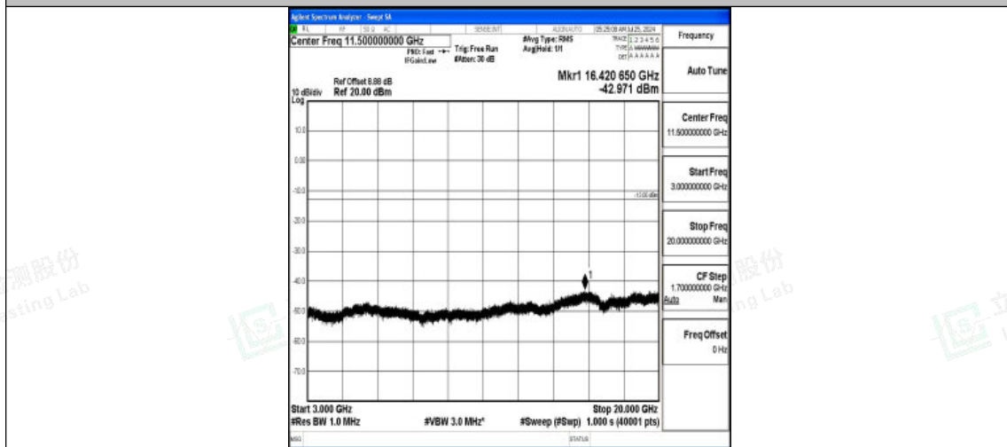
Band2-3MHz-QPSK-18615-1RB#0-3000~20000-PASS
