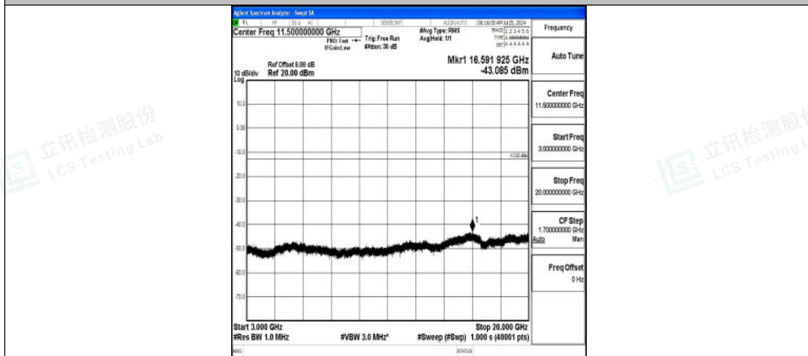
Band2-10MHz-16QAM-19150-1RB#0-3000~20000-PASS
