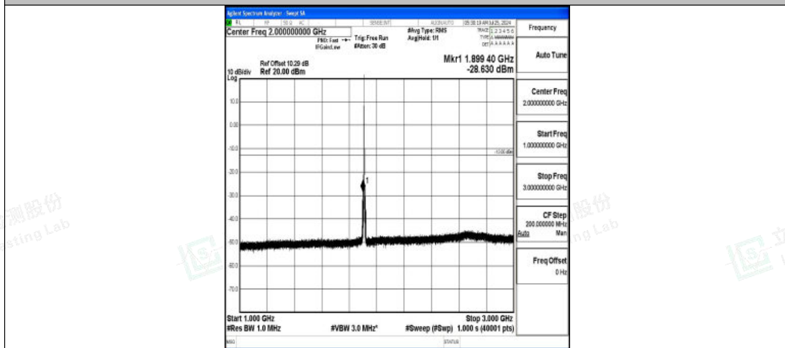
Band2-3MHz-16QAM-19185-1RB#0-1000~3000-PASS
