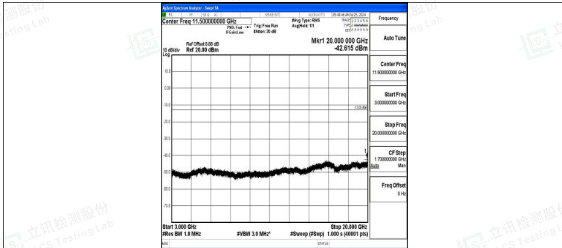
Band2-5MHz-16QAM-18625-1RB#0-3000~20000-PASS
