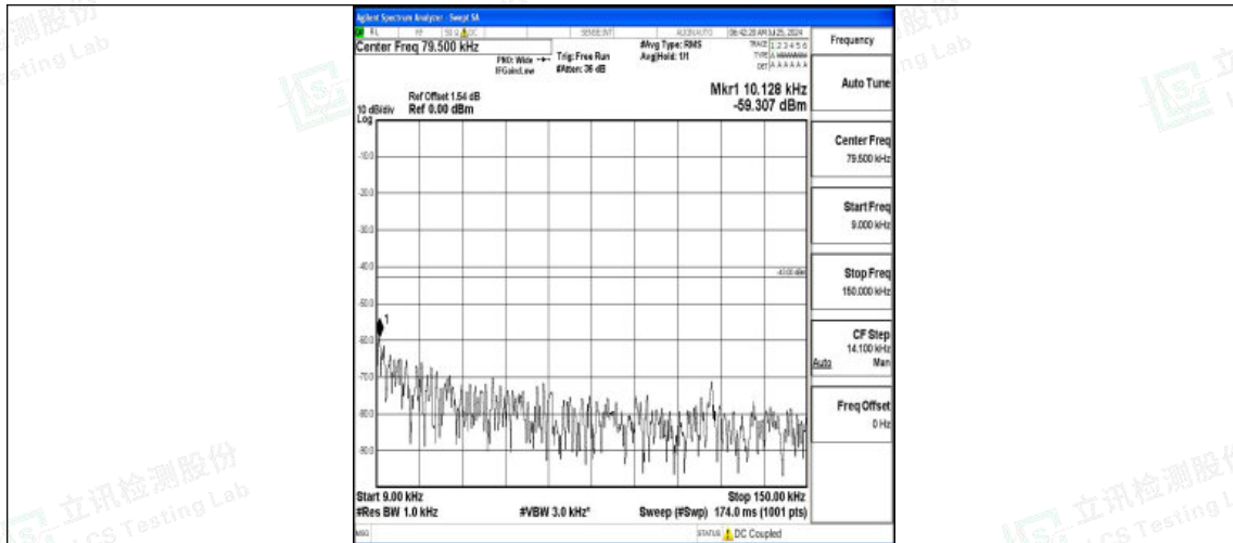
Band2-15MHz-16QAM-18900-1RB#0-0.009~0.15-PASS
