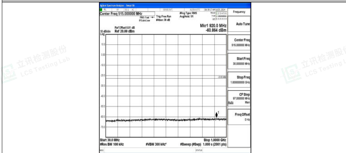
Band2-15MHz-QPSK-18675-1RB#0-30~1000-PASS
