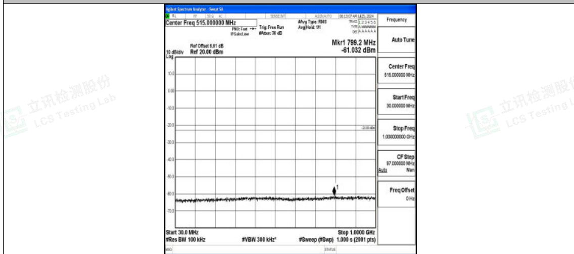
Band2-10MHz-16QAM-18900-1RB#0-30~1000-PASS
