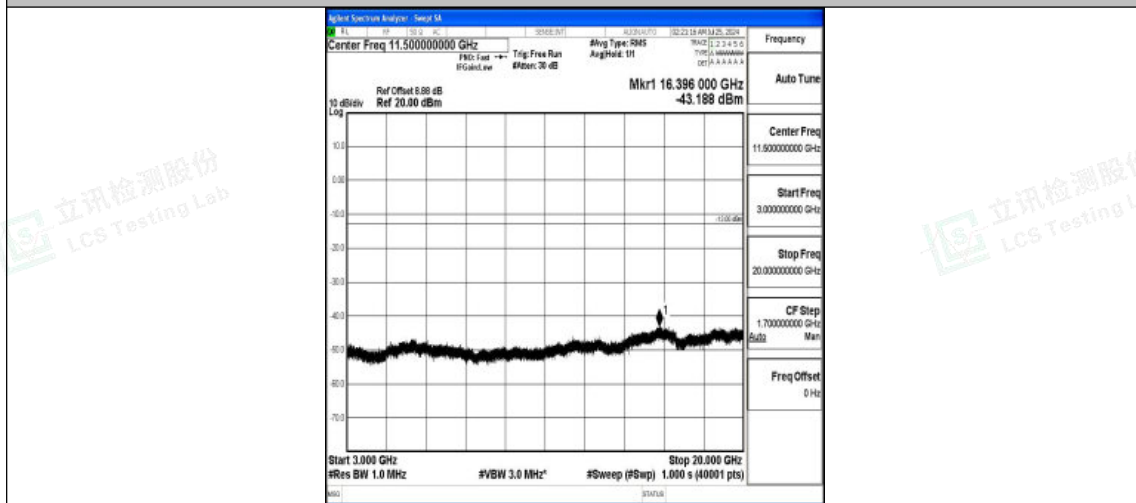
Band2-1.4MHz-16QAM-19193-1RB#0-3000~20000-PASS
