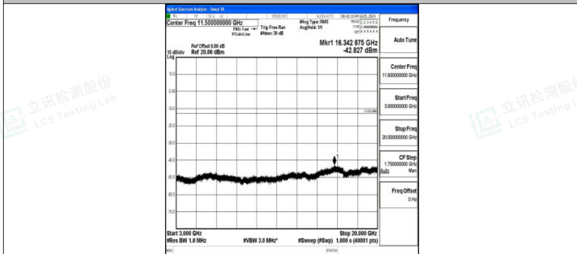
Band2-15MHz-QPSK-18900-1RB#0-3000~20000-PASS
