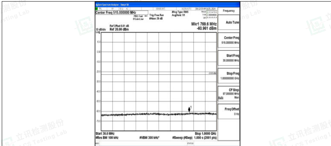
Band2-10MHz-QPSK-18900-1RB#0-30~1000-PASS
