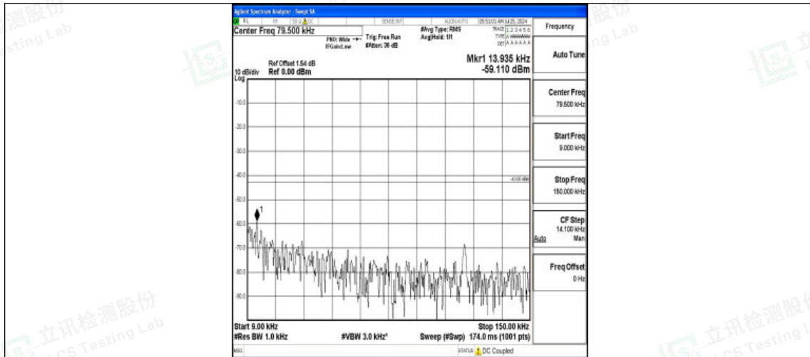
Band2-5MHz-16QAM-18900-1RB#0-0.009~0.15-PASS
