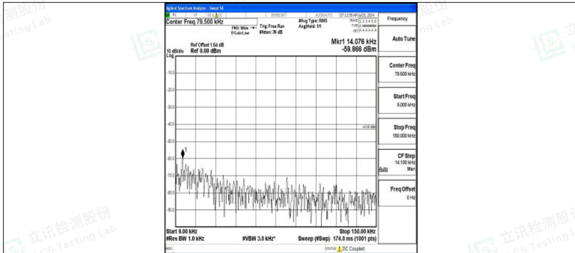
Band2-20MHz-QPSK-18700-1RB#0-0.009~0.15-PASS
