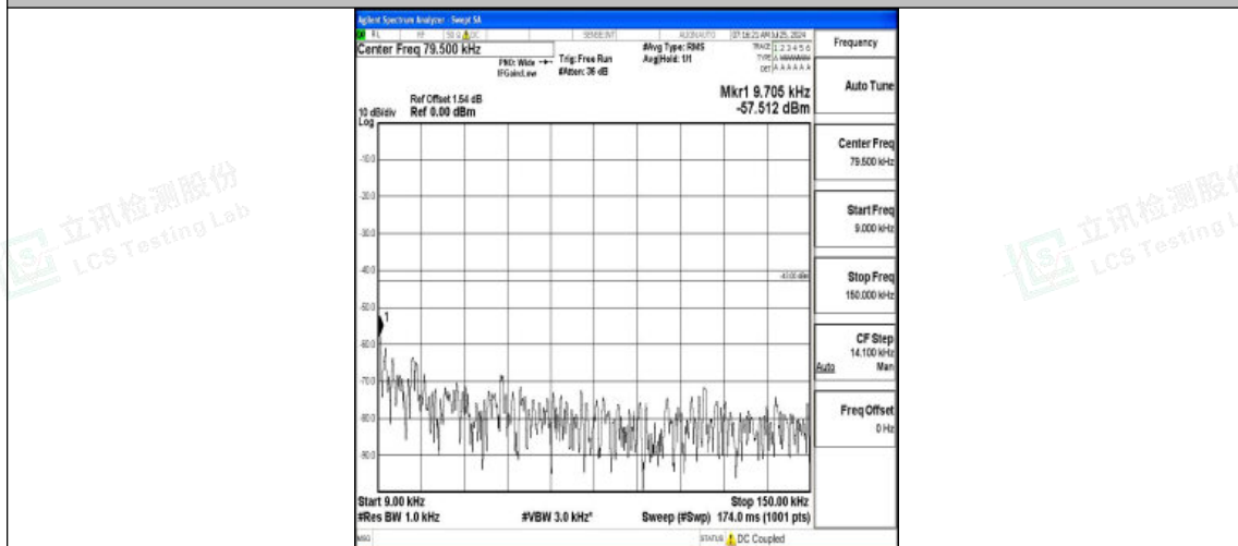
Band2-20MHz-QPSK-19100-1RB#0-0.009~0.15-PASS
