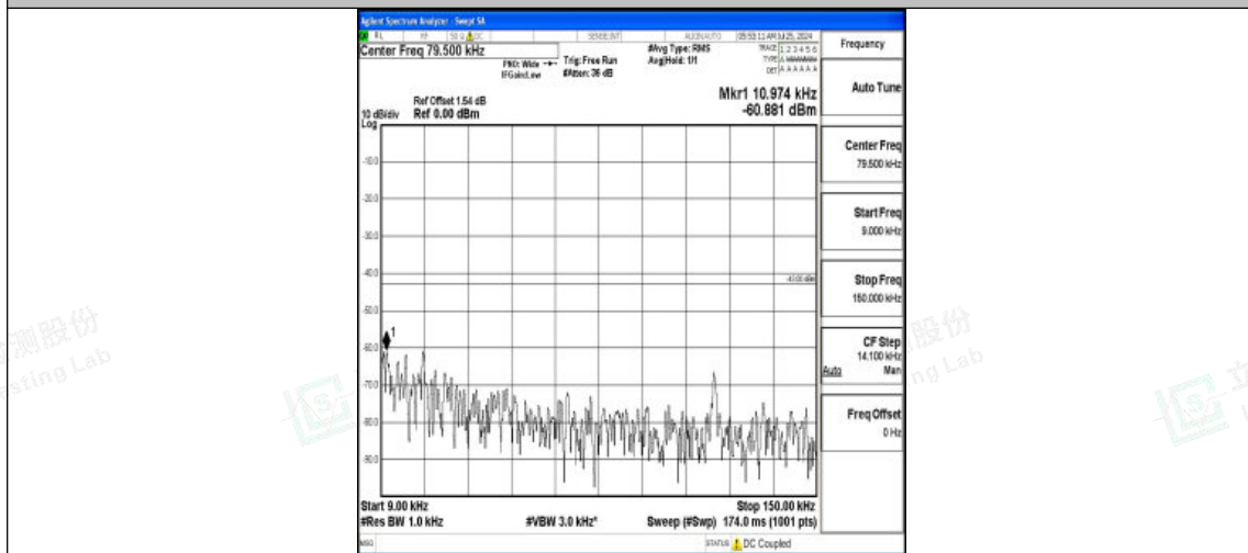
Band2-5MHz-16QAM-19175-1RB#0-0.009~0.15-PASS
