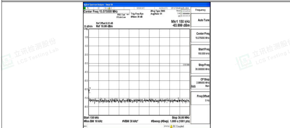
Band2-20MHz-16QAM-19100-1RB#0-0.15~30-PASS
