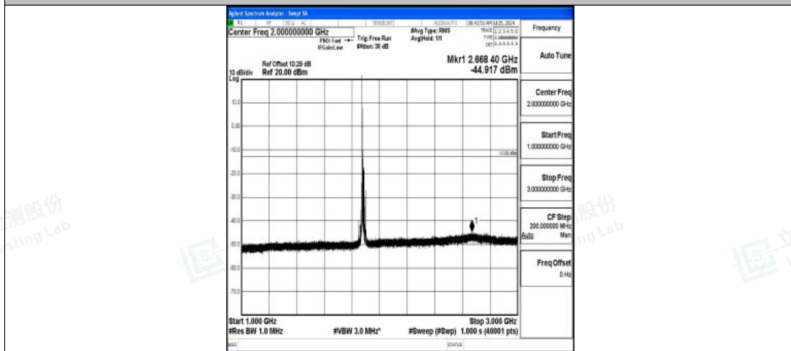
Band2-15MHz-QPSK-18900-1RB#0-1000~3000-PASS
