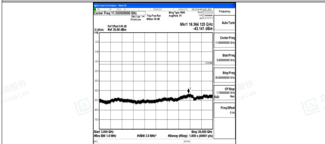
Band2-10MHz-16QAM-18900-1RB#0-3000~20000-PASS
