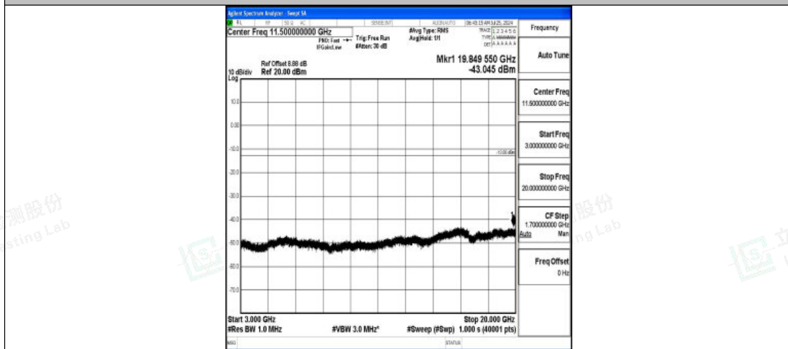
Band2-15MHz-16QAM-18900-1RB#0-3000~20000-PASS
