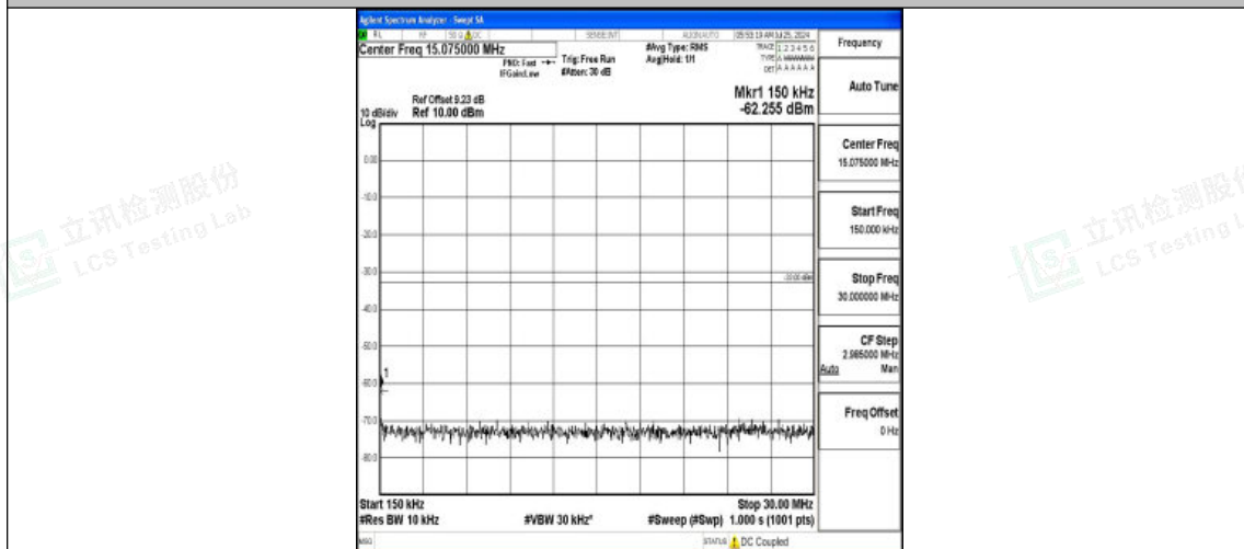
Band2-5MHz-16QAM-19175-1RB#0-0.15~30-PASS
