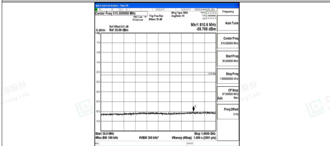
Band2-5MHz-QPSK-19175-1RB#0-30~1000-PASS
