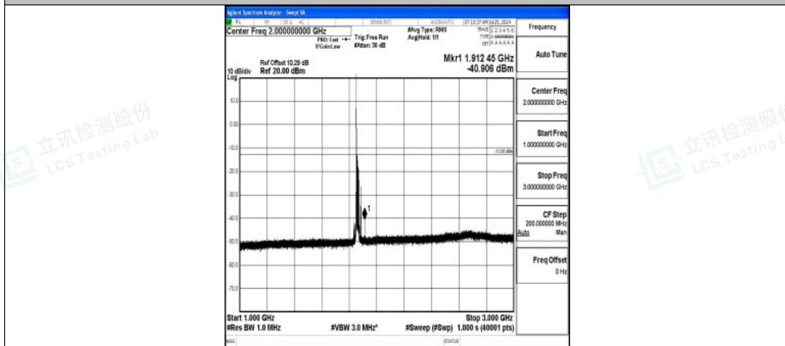
Band2-20MHz-16QAM-18700-1RB#0-1000~3000-PASS
