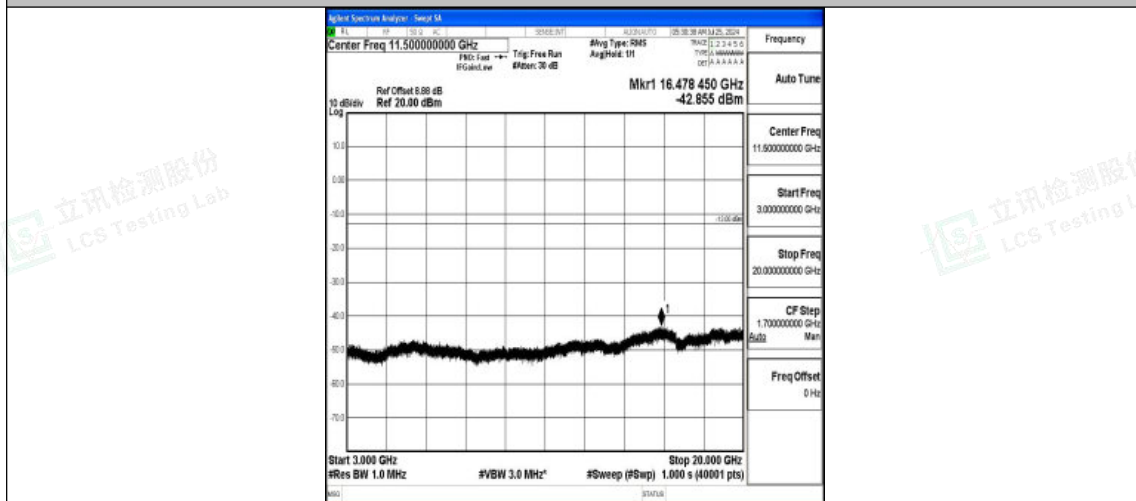
Band2-3MHz-16QAM-19185-1RB#0-3000~20000-PASS
