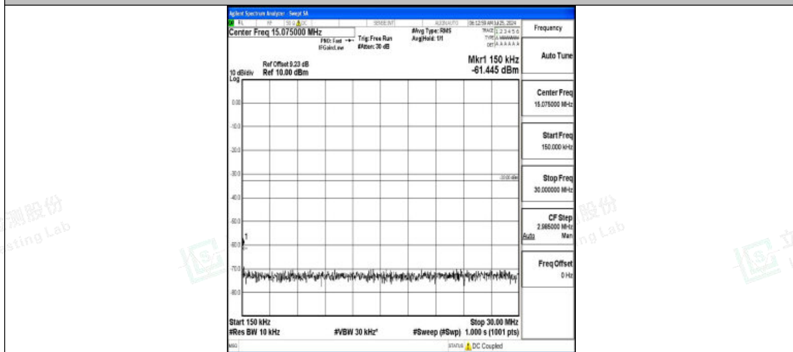
Band2-10MHz-16QAM-18900-1RB#0-0.15~30-PASS
