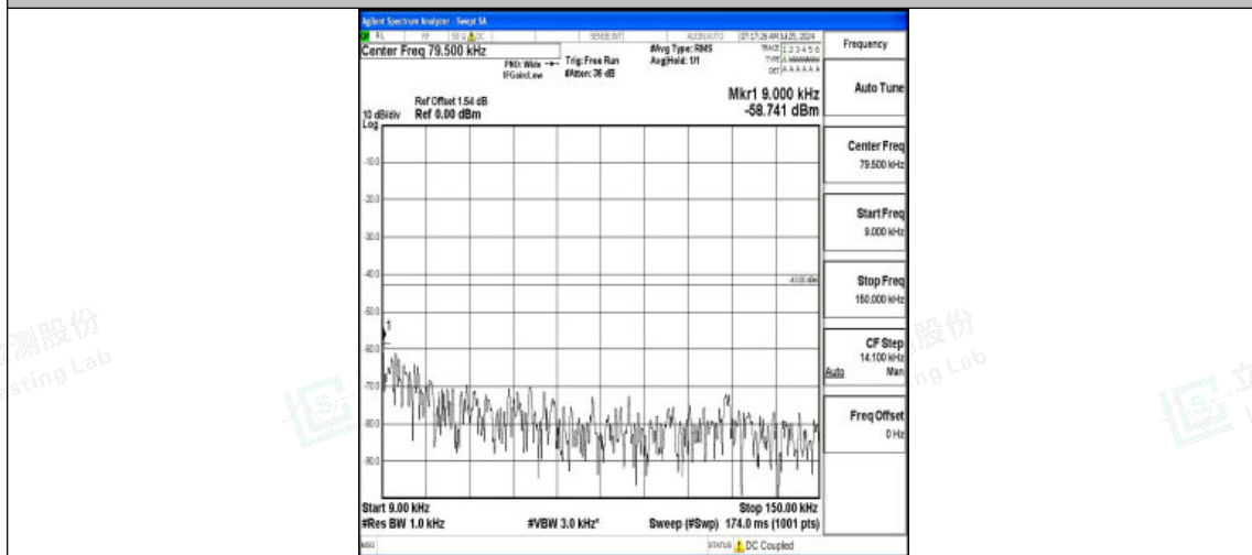
Band2-20MHz-16QAM-19100-1RB#0-0.009~0.15-PASS
