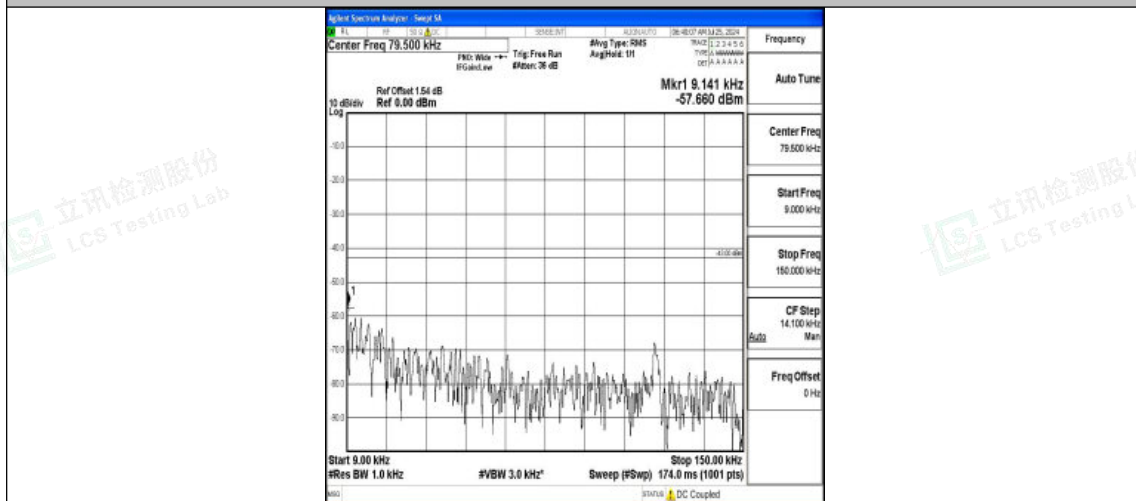
Band2-15MHz-16QAM-18675-1RB#0-0.009~0.15-PASS
