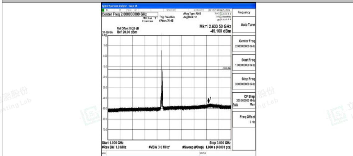
Band2-10MHz-QPSK-18900-1RB#0-1000~3000-PASS
