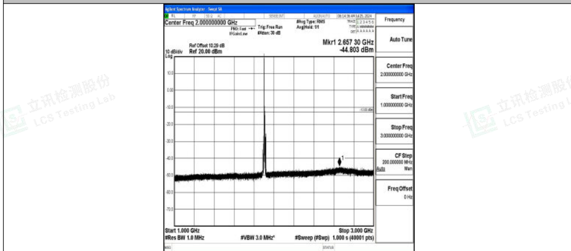
Band2-10MHz-QPSK-19150-1RB#0-1000~3000-PASS
