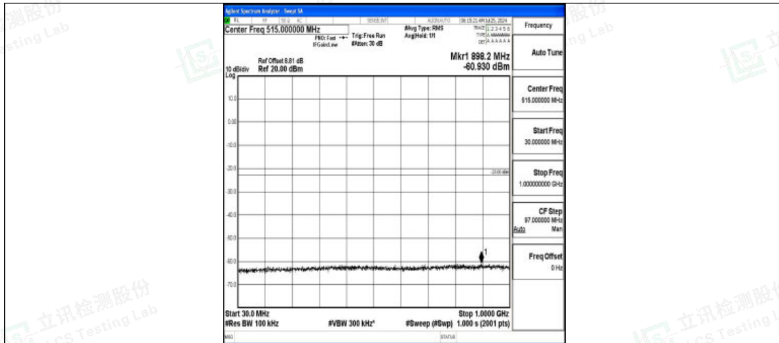
Band2-10MHz-16QAM-19150-1RB#0-30~1000-PASS
