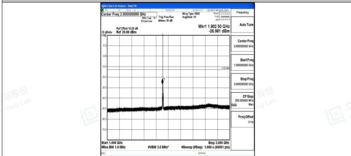
Band2-1.4MHz-16QAM-19193-1RB#0-1000~3000-PASS
