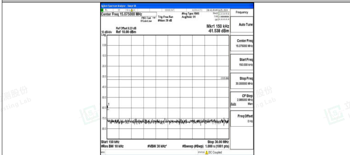
Band2-15MHz-16QAM-18900-1RB#0-0.15~30-PASS
