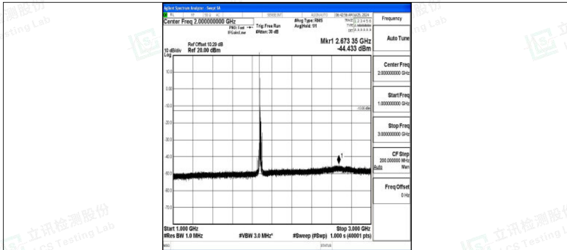
Band2-15MHz-16QAM-18900-1RB#0-1000~3000-PASS
