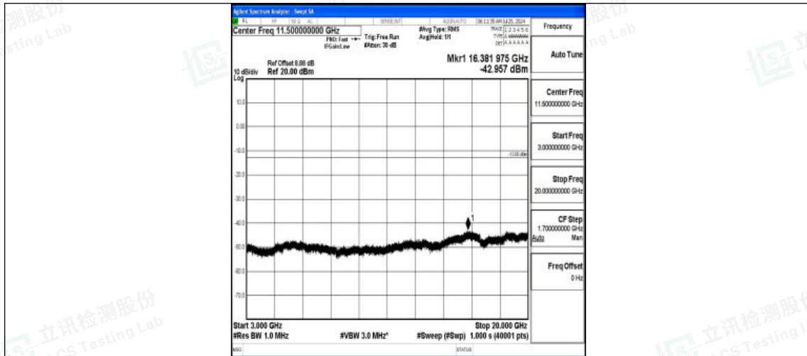
Band2-10MHz-16QAM-18650-1RB#0-3000~20000-PASS
