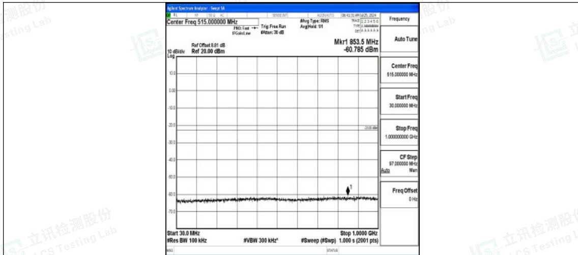
Band2-15MHz-QPSK-18900-1RB#0-30~1000-PASS
