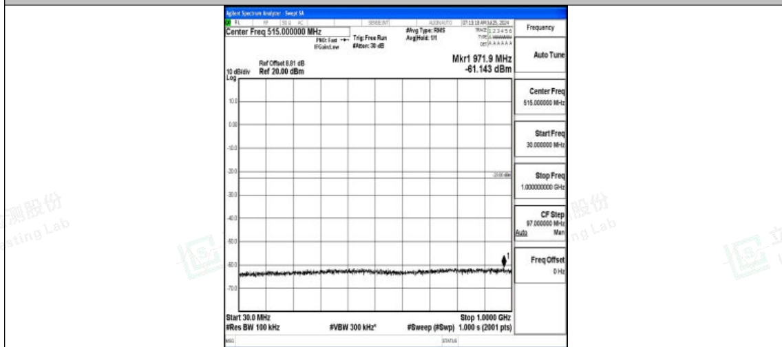
Band2-20MHz-16QAM-18700-1RB#0-30~1000-PASS
