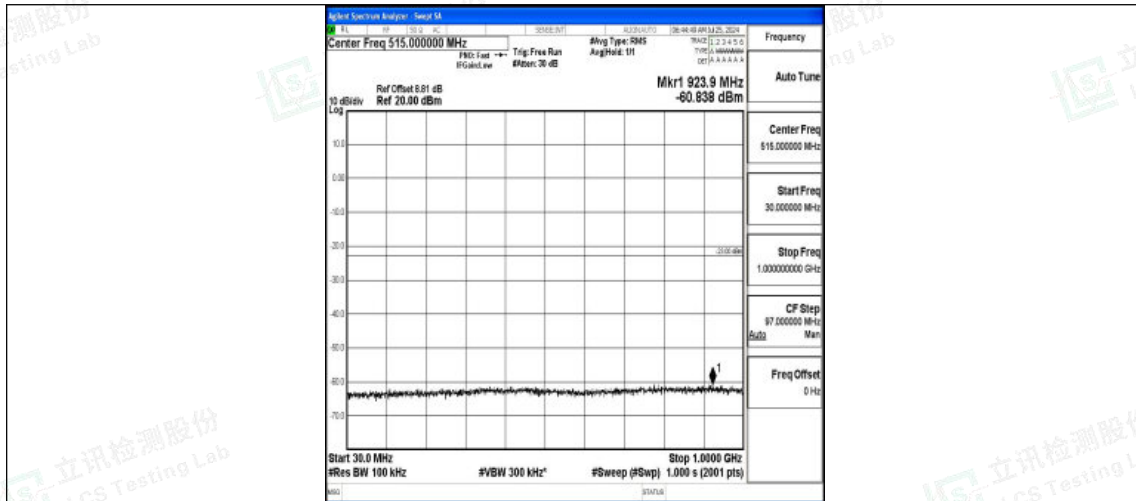
Band2-15MHz-16QAM-19125-1RB#0-30~1000-PASS
