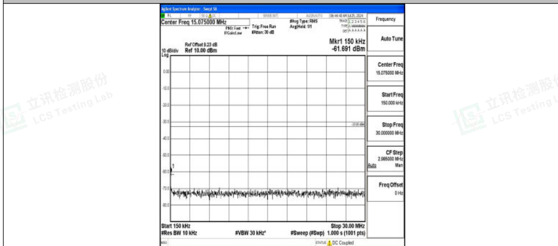
Band2-15MHz-16QAM-19125-1RB#0-0.15~30-PASS
