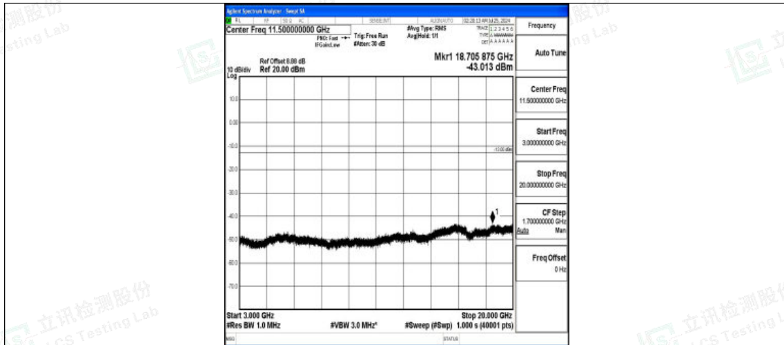
Band2-1.4MHz-QPSK-19193-1RB#0-3000~20000-PASS
