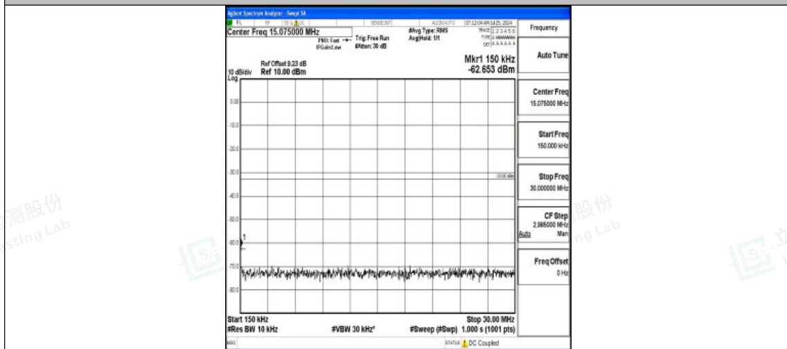
Band2-20MHz-QPSK-18700-1RB#0-0.15~30-PASS
