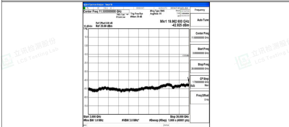
Band2-5MHz-16QAM-19175-1RB#0-3000~20000-PASS
