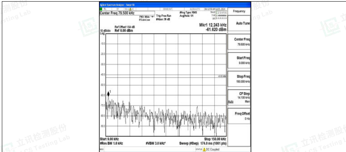
Band2-10MHz-16QAM-18900-1RB#0-0.009~0.15-PASS
