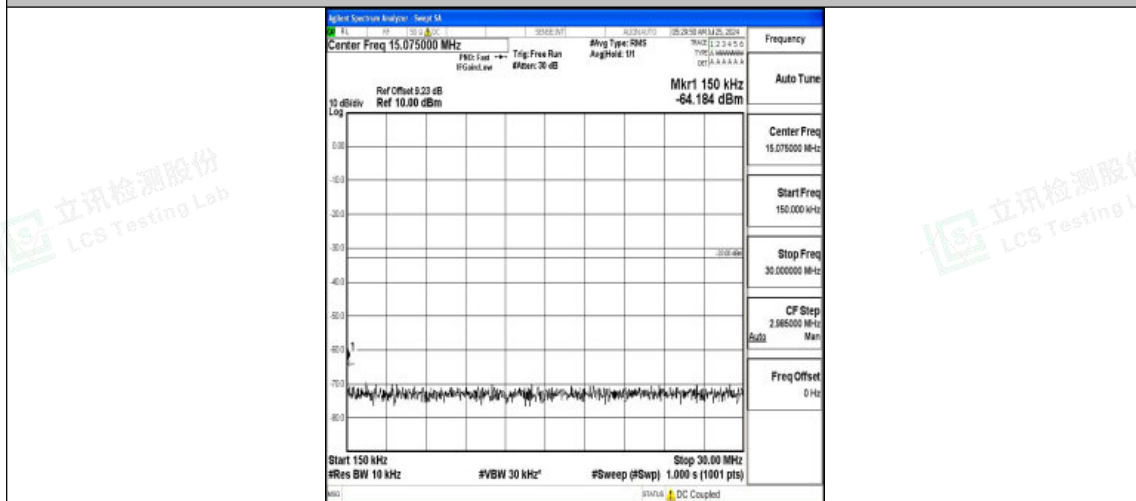
Band2-3MHz-16QAM-19185-1RB#0-0.15~30-PASS
