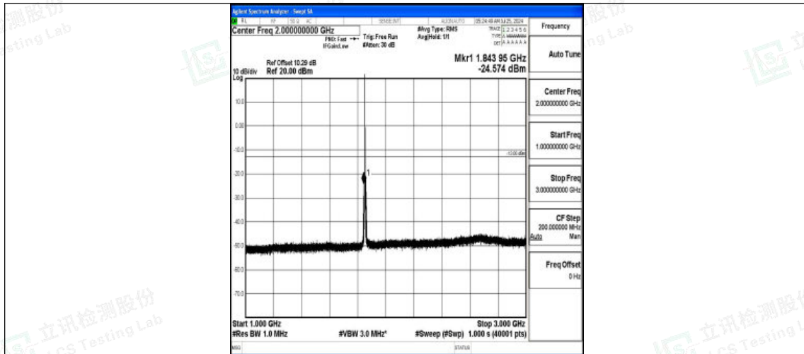
Band2-3MHz-QPSK-18615-1RB#0-1000~3000-PASS
