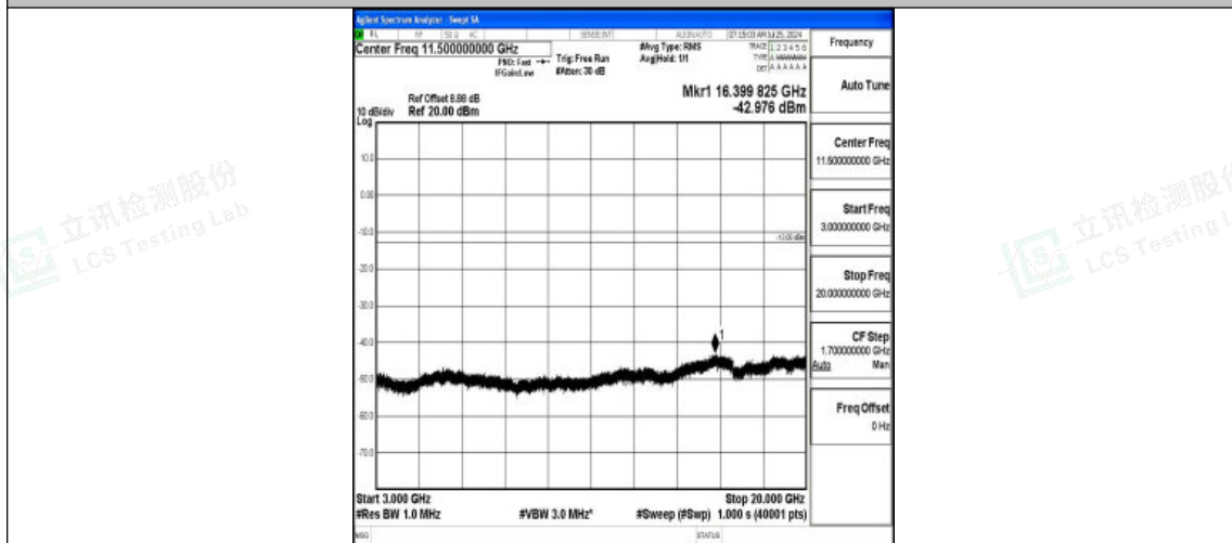
Band2-20MHz-QPSK-18900-1RB#0-3000~20000-PASS
