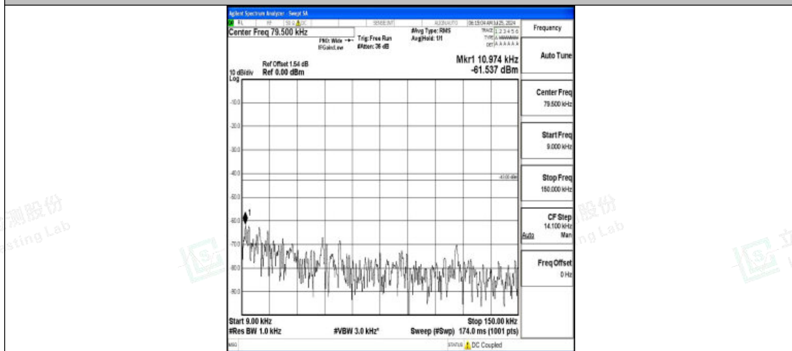
Band2-10MHz-16QAM-19150-1RB#0-0.009~0.15-PASS
