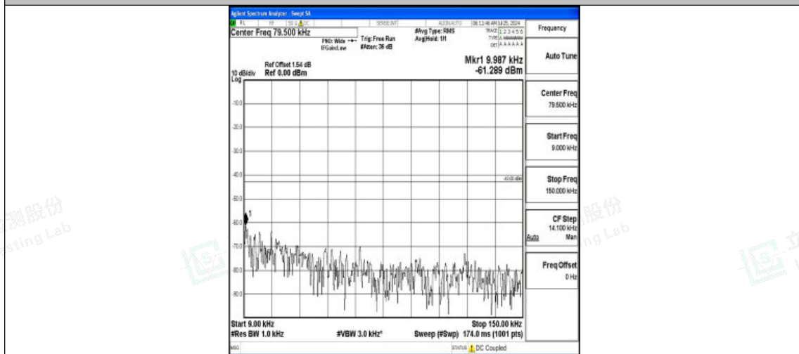
Band2-10MHz-QPSK-18900-1RB#0-0.009~0.15-PASS
