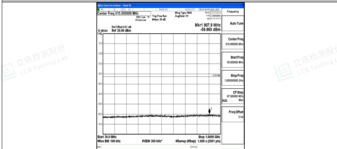
Band2-3MHz-QPSK-18615-1RB#0-30~1000-PASS
