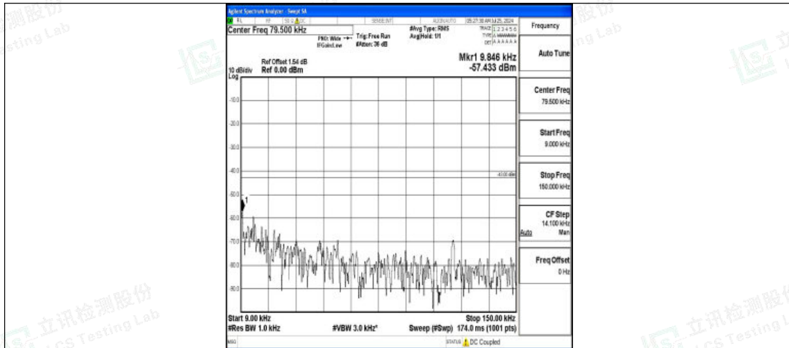
Band2-3MHz-16QAM-18900-1RB#0-0.009~0.15-PASS
