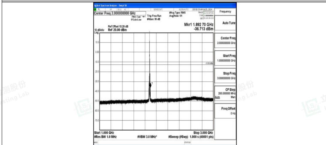
Band2-5MHz-QPSK-18900-1RB#0-1000~3000-PASS
