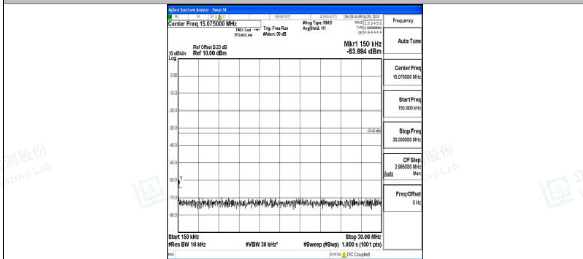
Band2-10MHz-QPSK-18650-1RB#0-0.15~30-PASS
