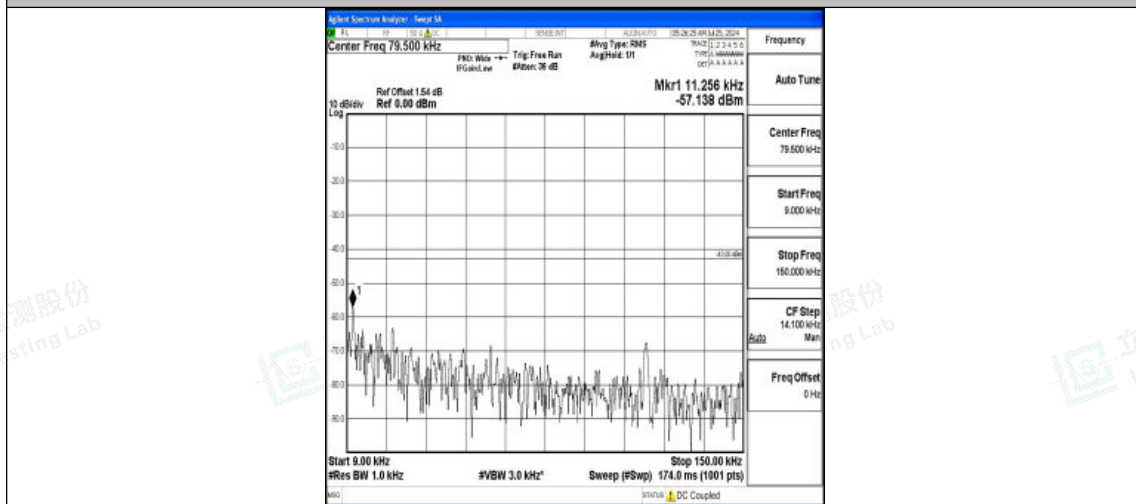
Band2-3MHz-QPSK-18900-1RB#0-0.009~0.15-PASS
