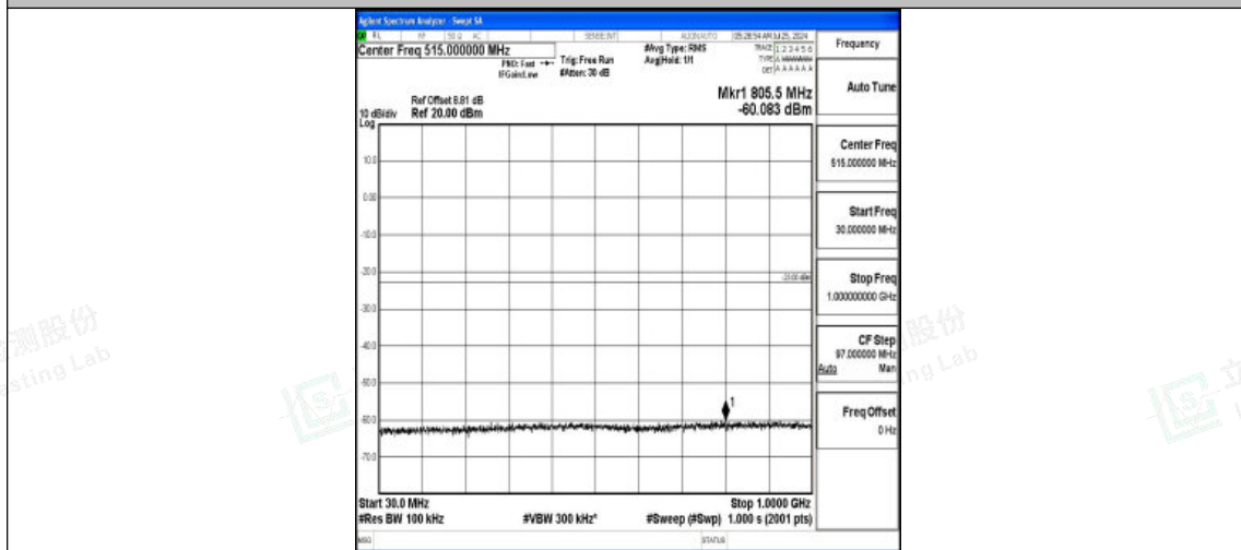
Band2-3MHz-QPSK-19185-1RB#0-30~1000-PASS
