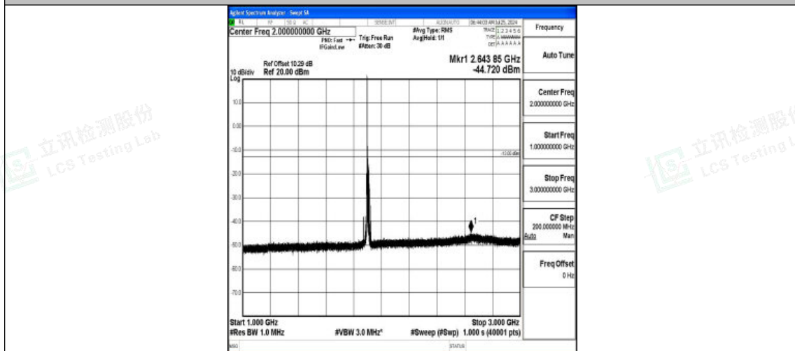
Band2-15MHz-QPSK-19125-1RB#0-1000~3000-PASS
