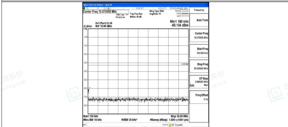
Band2-20MHz-16QAM-18900-1RB#0-0.15~30-PASS
