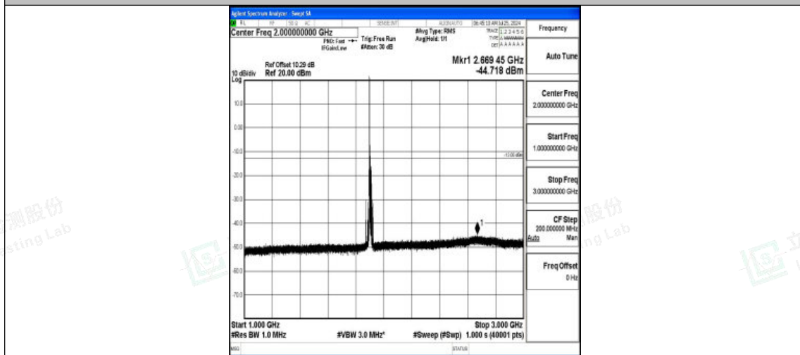
Band2-15MHz-16QAM-19125-1RB#0-1000~3000-PASS
