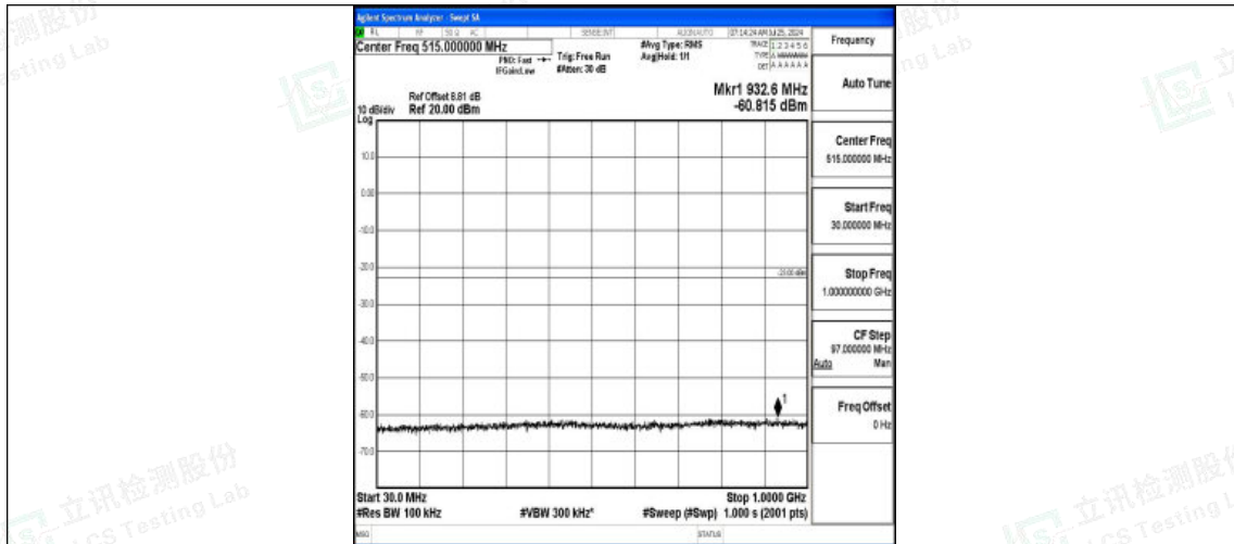
Band2-20MHz-QPSK-18900-1RB#0-30~1000-PASS
