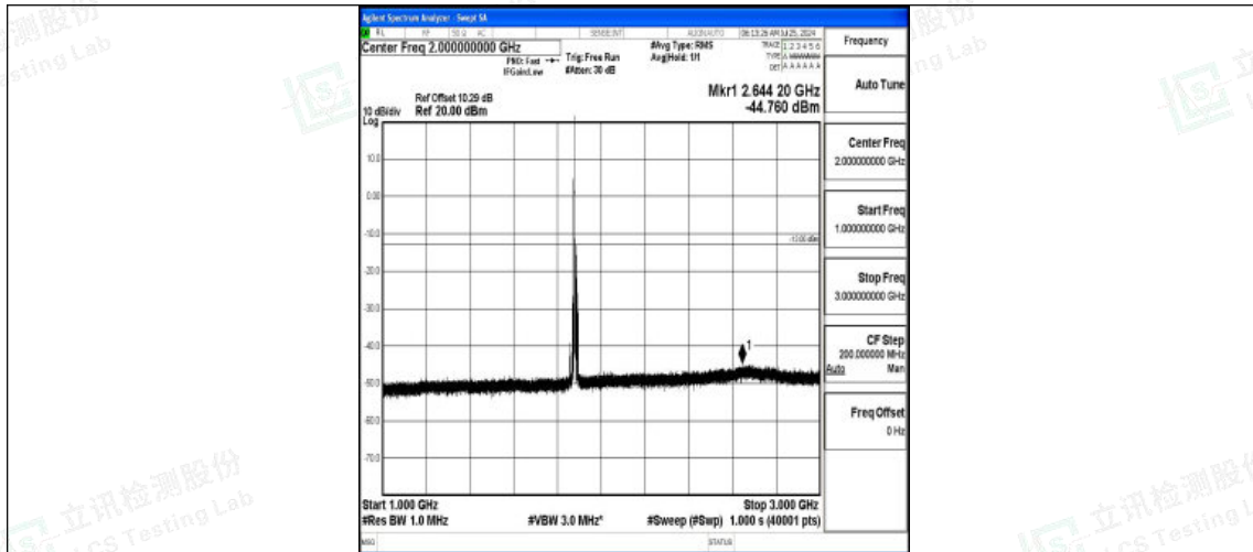
Band2-10MHz-16QAM-18900-1RB#0-1000~3000-PASS
