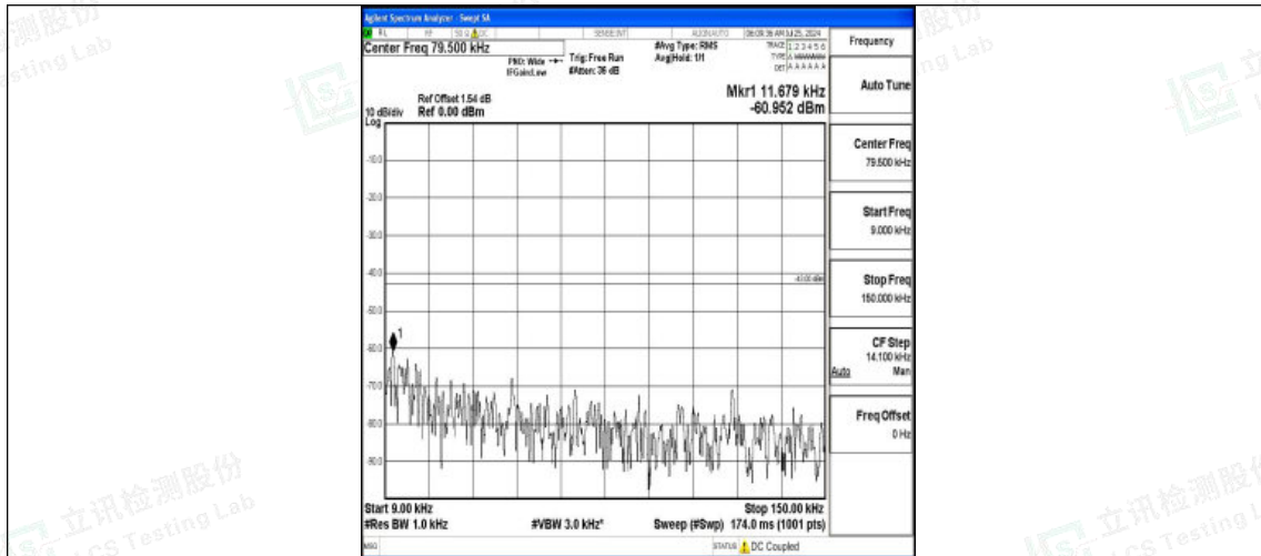
Band2-10MHz-QPSK-18650-1RB#0-0.009~0.15-PASS
