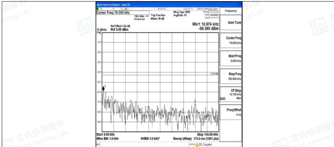
Band2-3MHz-QPSK-18615-1RB#0-0.009~0.15-PASS
