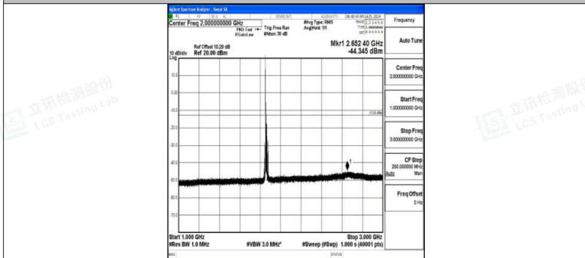
Band2-15MHz-16QAM-18675-1RB#0-1000~3000-PASS
