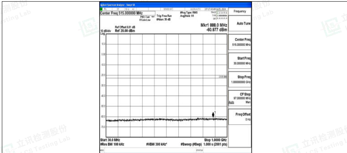
Band2-20MHz-16QAM-19100-1RB#0-30~1000-PASS
