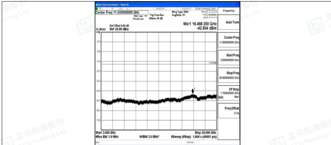
Band2-3MHz-16QAM-18615-1RB#0-3000~20000-PASS
