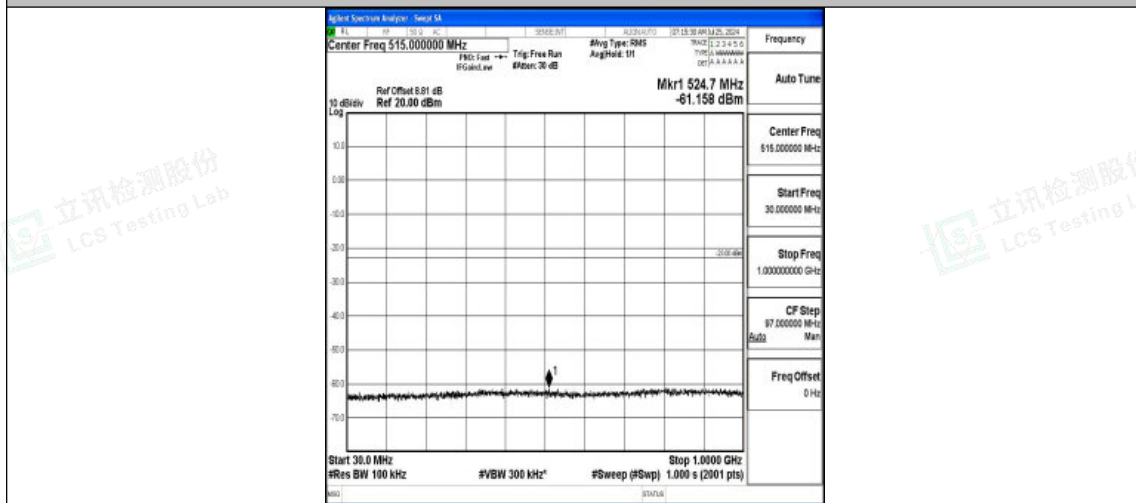
Band2-20MHz-16QAM-18900-1RB#0-30~1000-PASS
