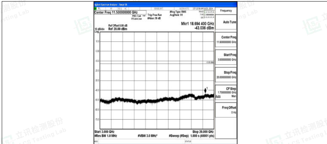
Band2-20MHz-16QAM-18700-1RB#0-3000~20000-PASS
