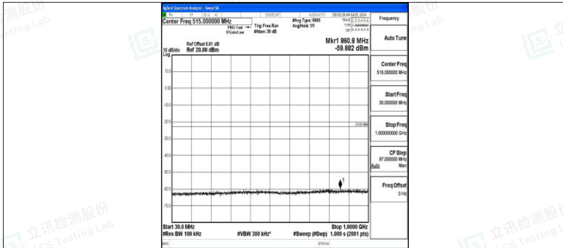
Band2-5MHz-16QAM-19175-1RB#0-30~1000-PASS
