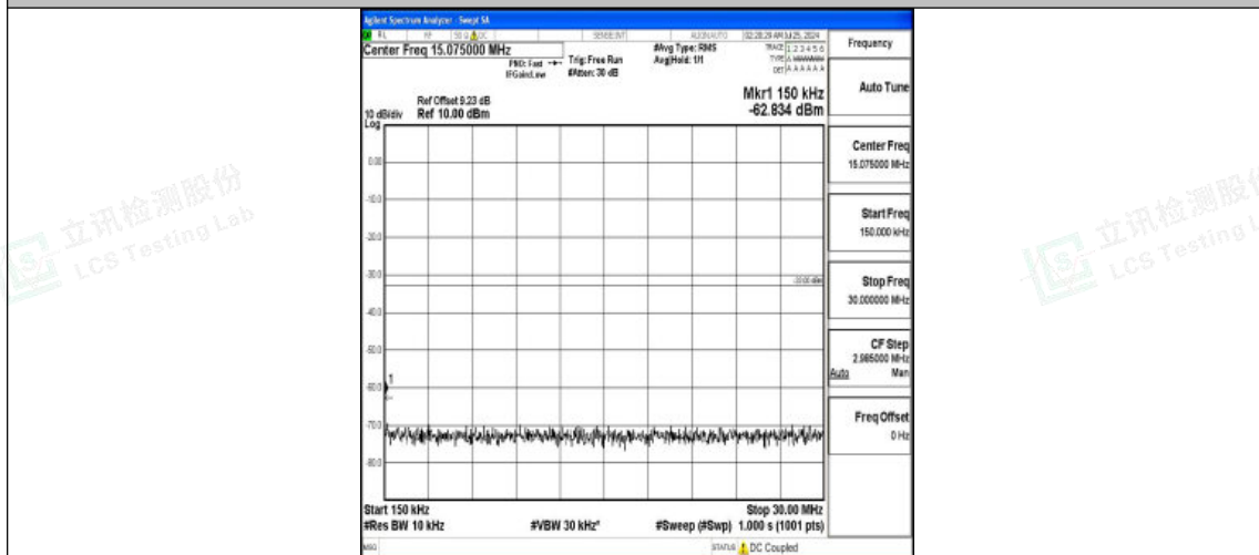
Band2-1.4MHz-16QAM-19193-1RB#0-0.15~30-PASS
