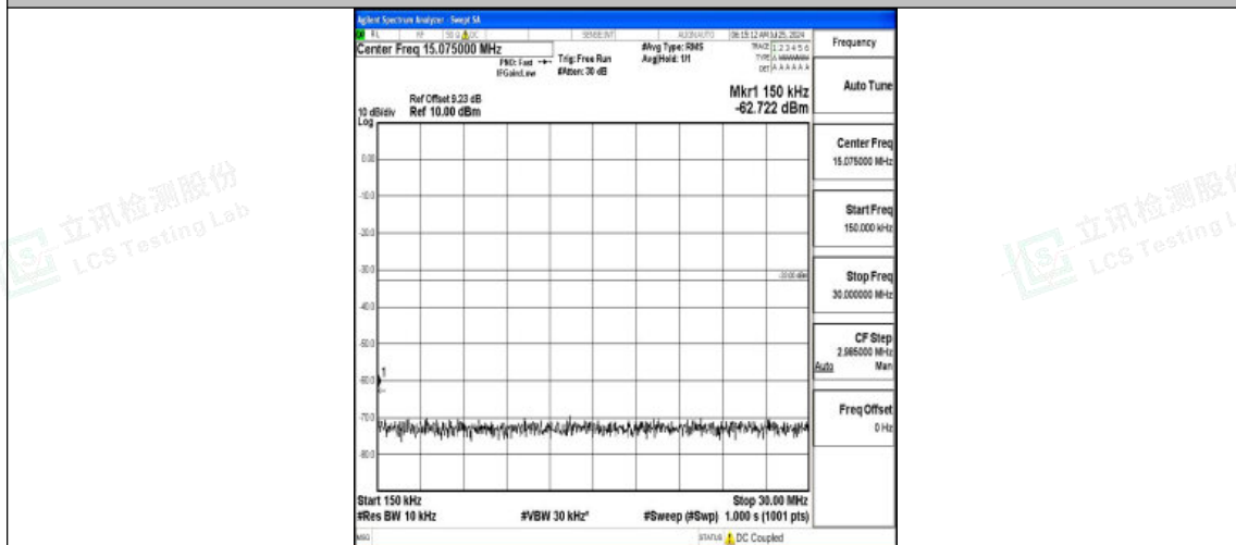
Band2-10MHz-16QAM-19150-1RB#0-0.15~30-PASS
