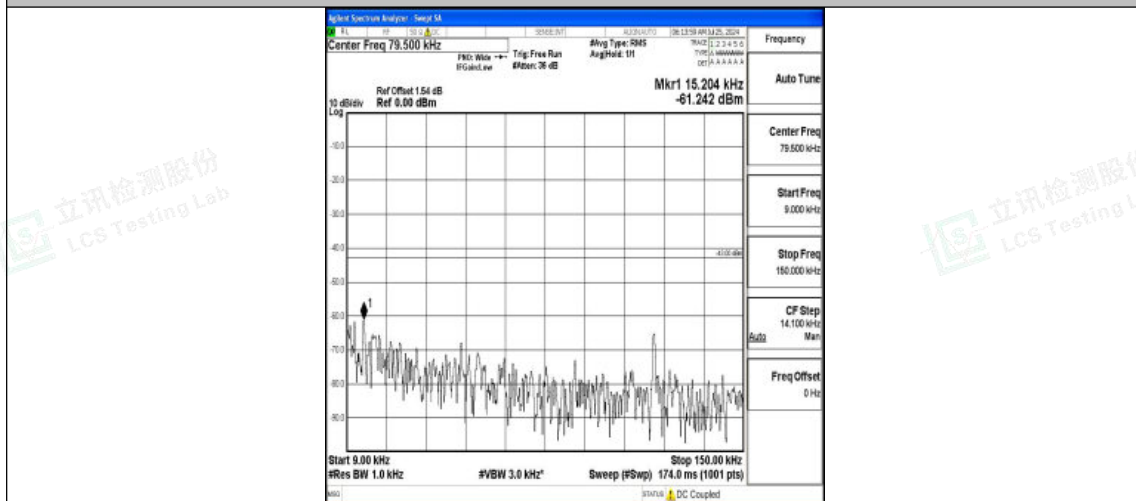
Band2-10MHz-QPSK-19150-1RB#0-0.009~0.15-PASS
