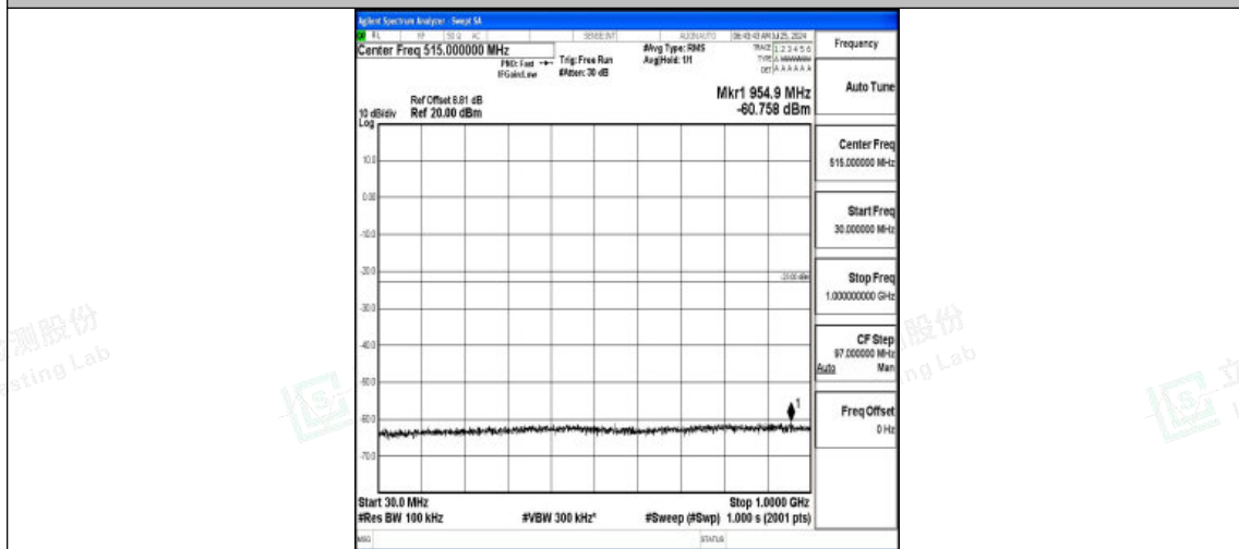
Band2-15MHz-QPSK-19125-1RB#0-30~1000-PASS
