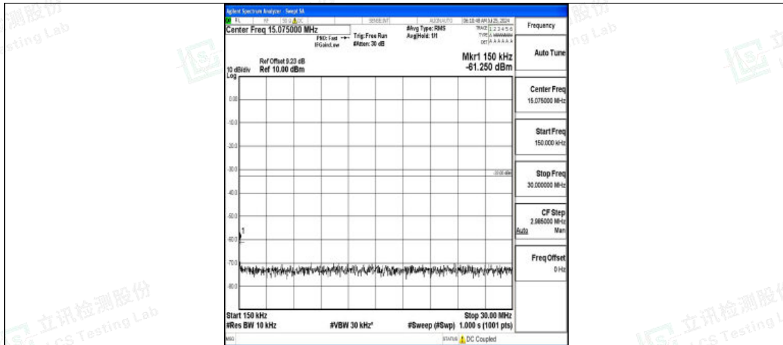
Band2-10MHz-16QAM-18650-1RB#0-0.15~30-PASS
