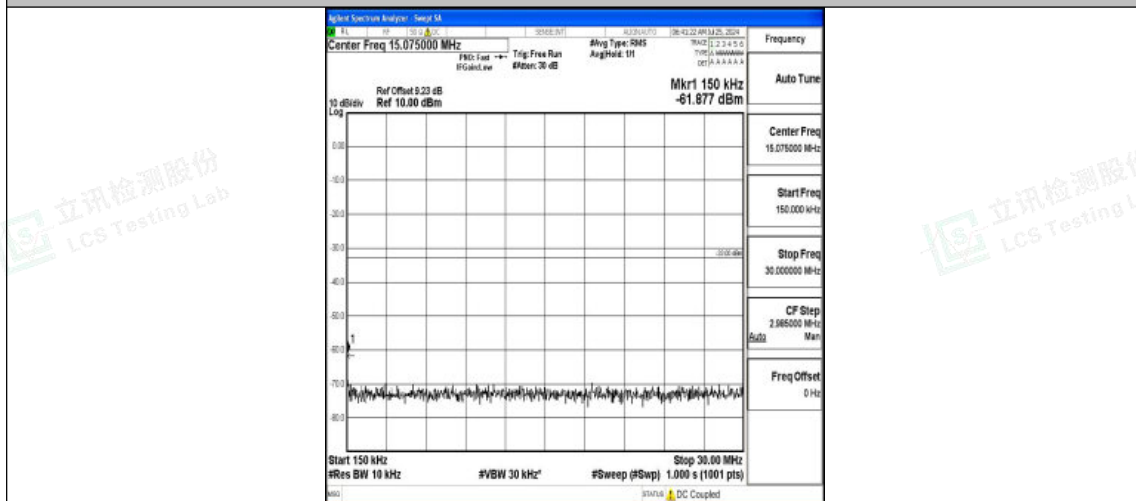
Band2-15MHz-QPSK-18900-1RB#0-0.15~30-PASS
