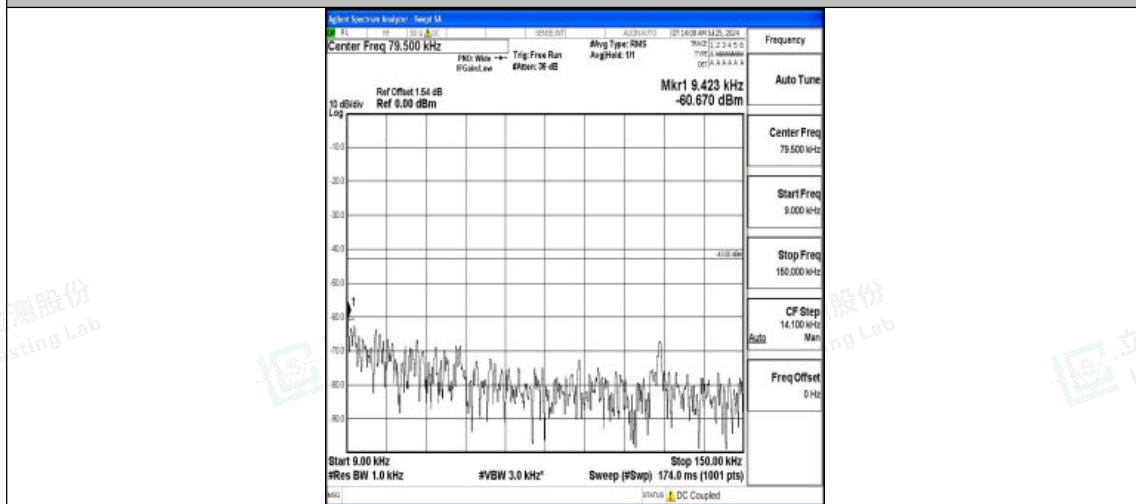
Band2-20MHz-QPSK-18900-1RB#0-0.009~0.15-PASS
