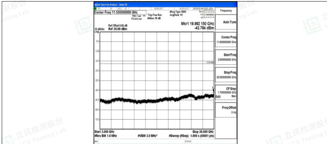
Band2-5MHz-QPSK-19175-1RB#0-3000~20000-PASS
