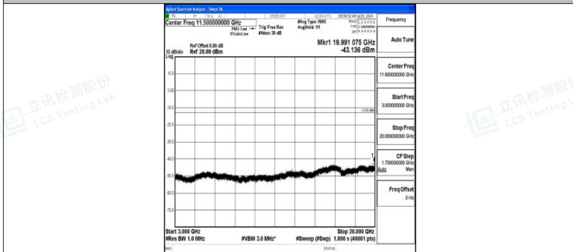
Band2-5MHz-QPSK-18900-1RB#0-3000~20000-PASS
