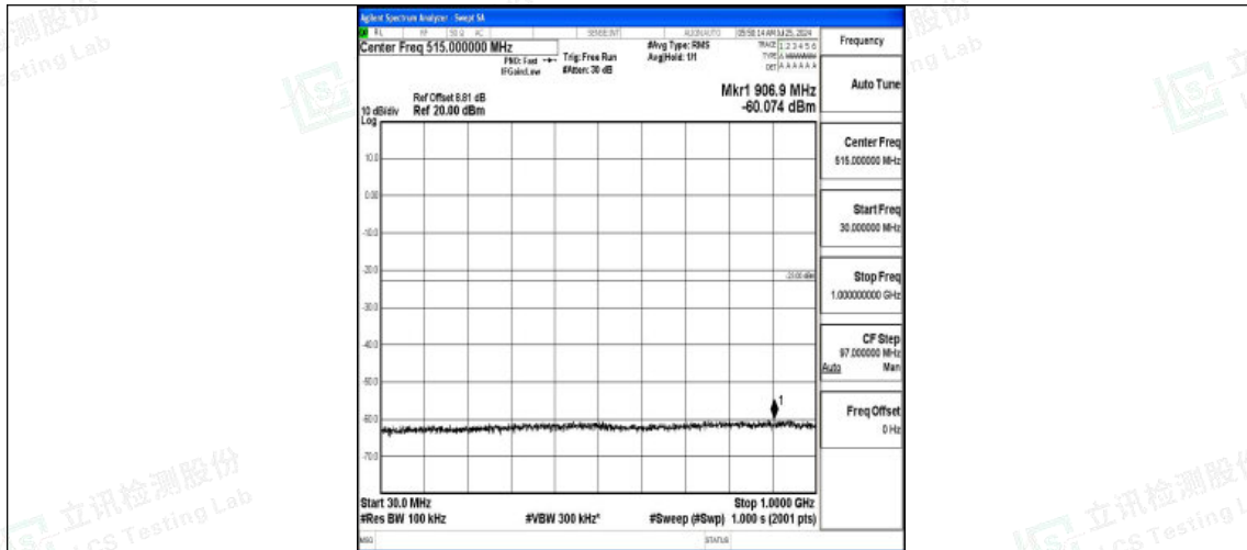
Band2-5MHz-QPSK-18900-1RB#0-30~1000-PASS
