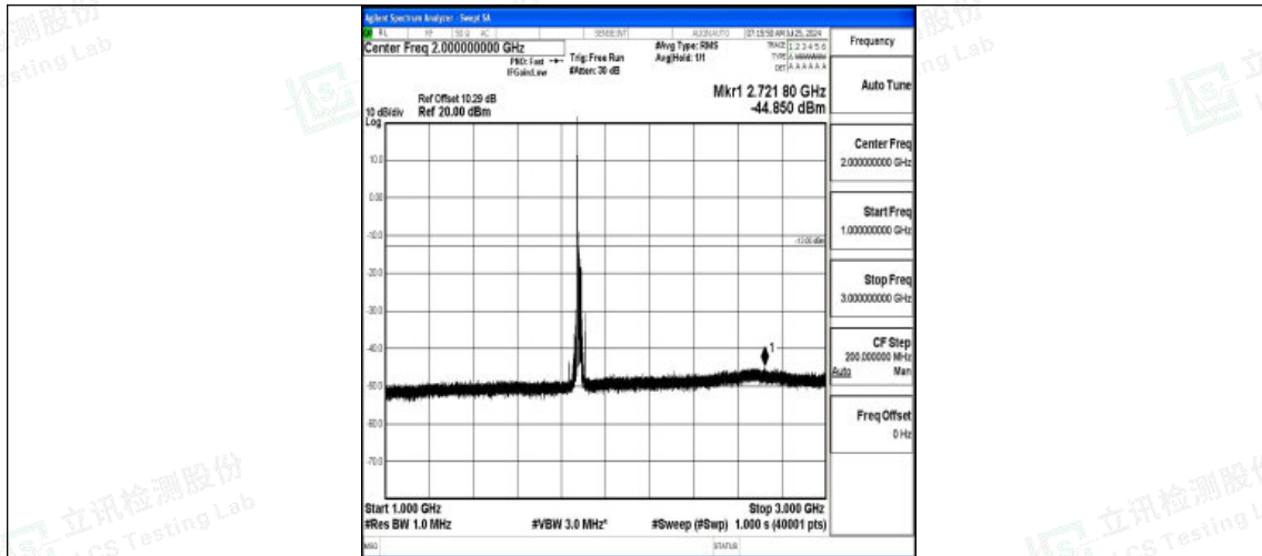
Band2-20MHz-16QAM-18900-1RB#0-1000~3000-PASS
