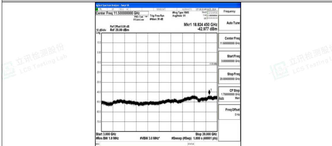
Band2-20MHz-16QAM-19100-1RB#0-3000~20000-PASS
