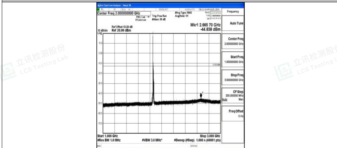
Band2-10MHz-16QAM-18650-1RB#0-1000~3000-PASS
