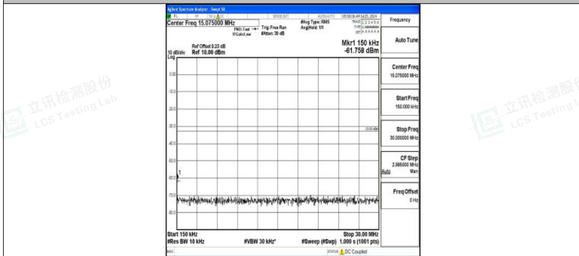
Band2-5MHz-QPSK-18900-1RB#0-0.15~30-PASS
