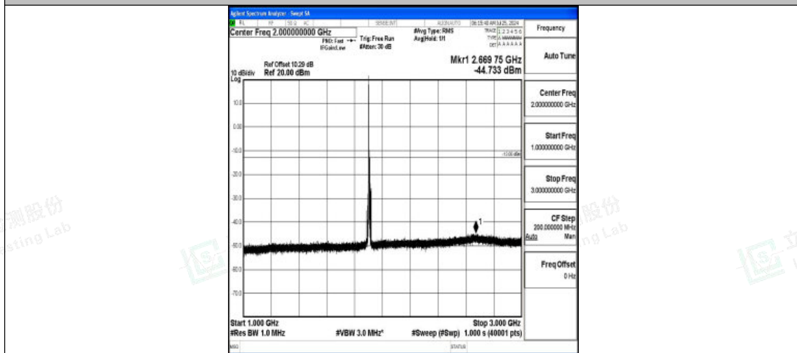
Band2-10MHz-16QAM-19150-1RB#0-1000~3000-PASS
