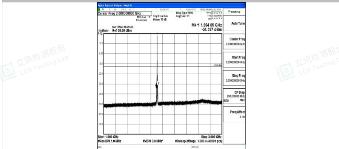
Band2-5MHz-QPSK-19175-1RB#0-1000~3000-PASS
