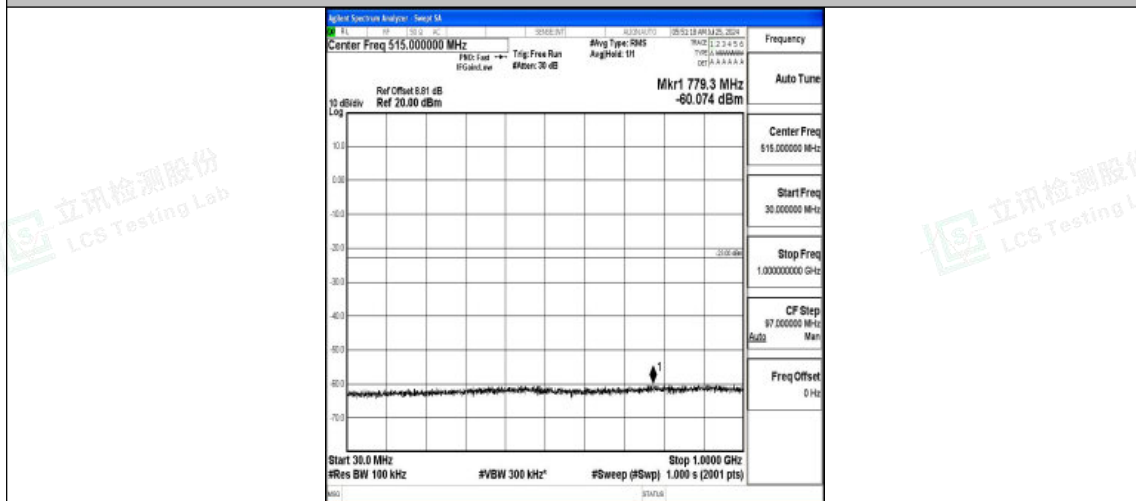
Band2-5MHz-16QAM-18900-1RB#0-30~1000-PASS
