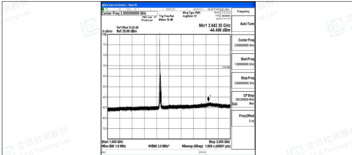
Band2-15MHz-QPSK-18675-1RB#0-1000~3000-PASS
