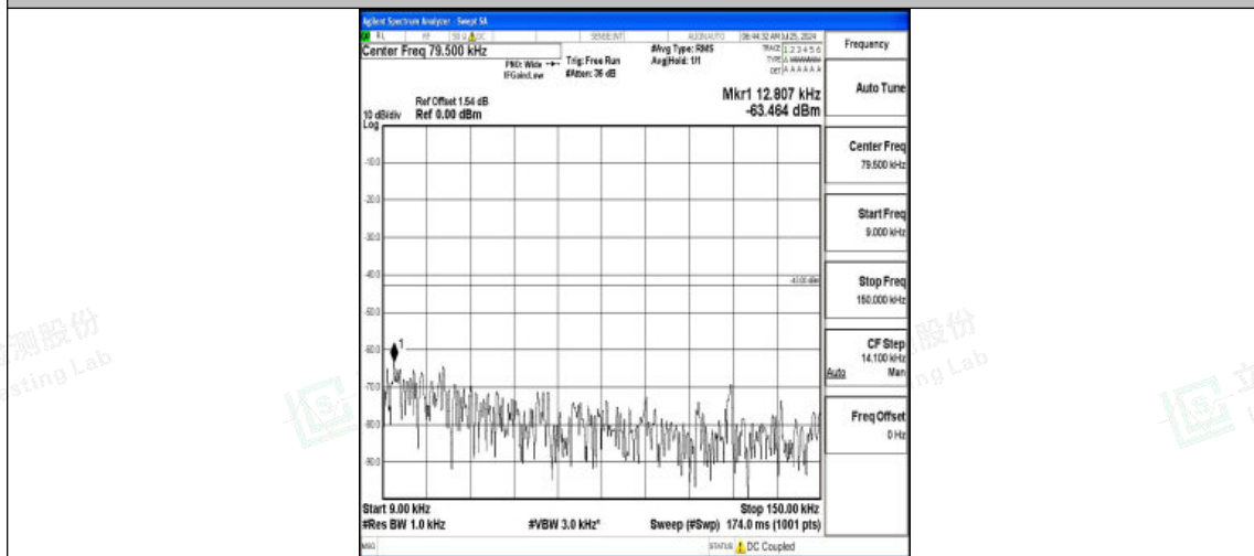
Band2-15MHz-16QAM-19125-1RB#0-0.009~0.15-PASS
