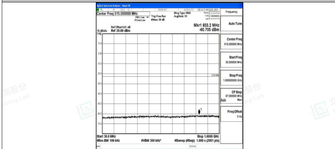
Band2-10MHz-QPSK-19150-1RB#0-30~1000-PASS
