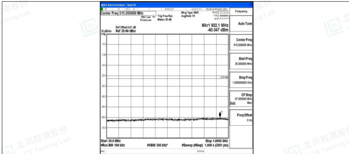
Band2-3MHz-QPSK-18900-1RB#0-30~1000-PASS
