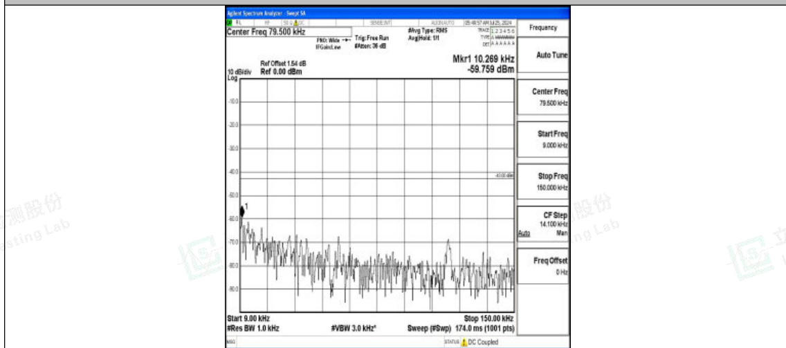
Band2-5MHz-QPSK-18900-1RB#0-0.009~0.15-PASS
