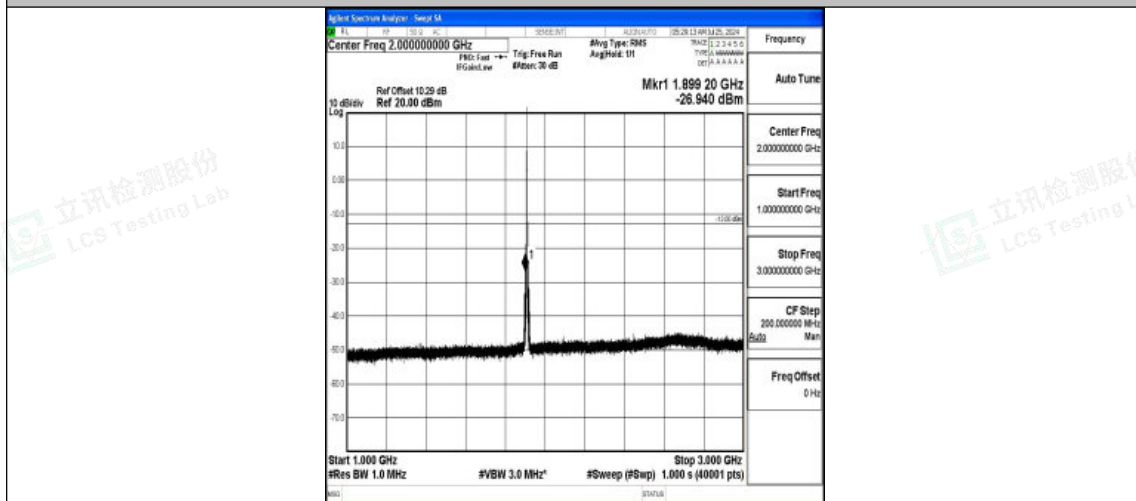
Band2-3MHz-QPSK-19185-1RB#0-1000~3000-PASS
