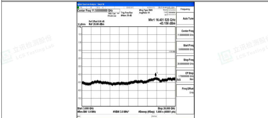
Band2-3MHz-QPSK-18900-1RB#0-3000~20000-PASS
