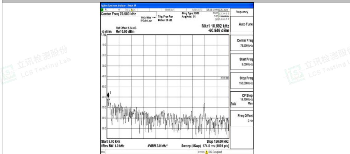
Band2-3MHz-16QAM-18615-1RB#0-0.009~0.15-PASS
