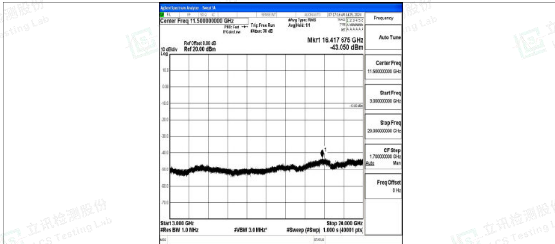
Band2-20MHz-QPSK-19100-1RB#0-3000~20000-PASS
