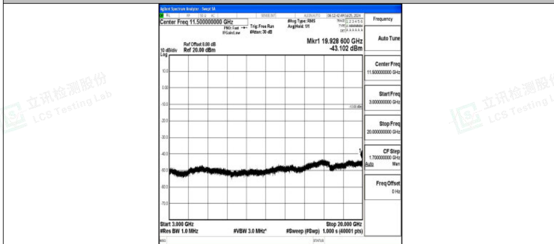
Band2-10MHz-QPSK-18900-1RB#0-3000~20000-PASS
