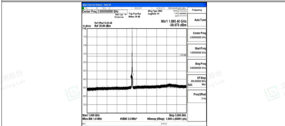
Band2-5MHz-16QAM-19175-1RB#0-1000~3000-PASS
