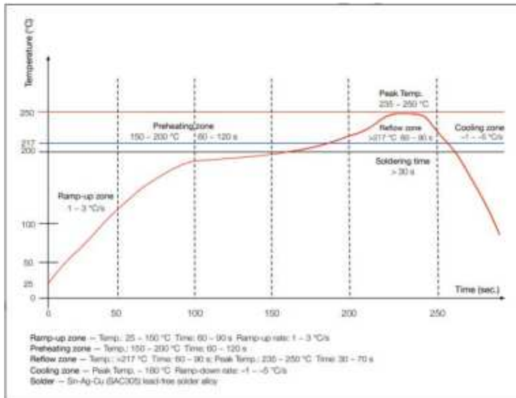
Figure 5 Reflow Profile
