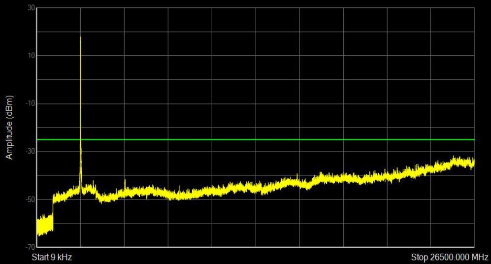
Band41 QPSK BW=20MHz Channel=41490 RB Size=100 Position=#0
