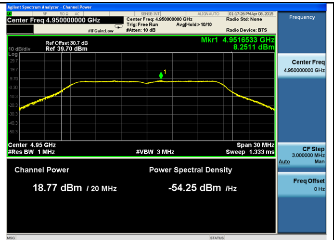
Chain 2 Ave Output Power (20dBi Antenna) - 4950MHz
