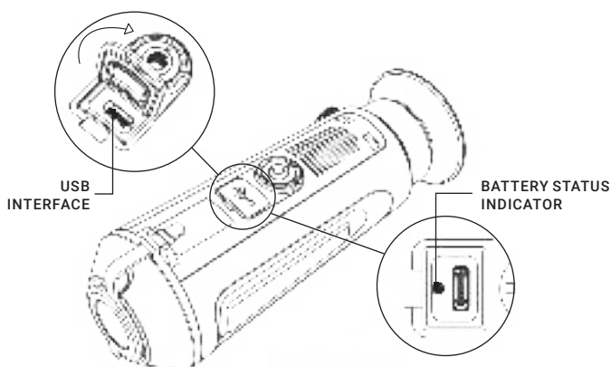
FIGURE 2-1. TAIPAN CHARGING
