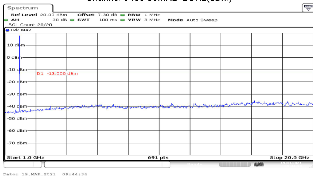
Channel 9400 1GHz~20GHz(dBm)
