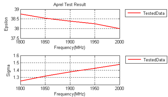
1 900 MHz Head, 2014.06.06
