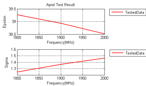
1 900 MHz Head, 2014.06.07
