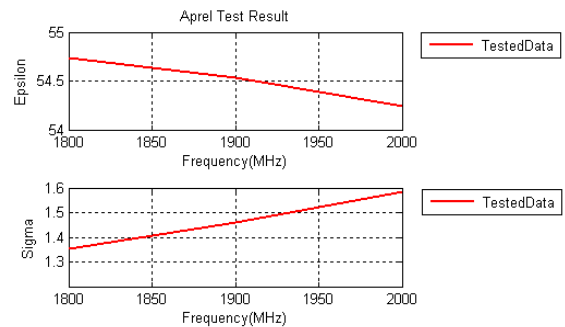
1 900 MHz Body, 2014.06.11
