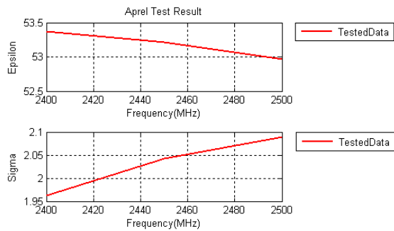
2 450 MHz Body, 2014.06.03
