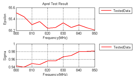
835 MHz Body, 2014.06.18
