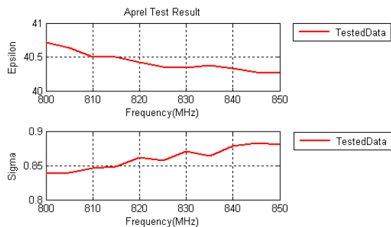
835 MHz Head, 2014.06.13
