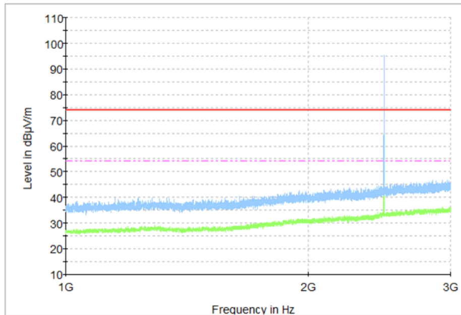
Fig. 53 Radiated Spurious Emission (8DPSK, Ch78, 1 GHz ~3 GHz)
