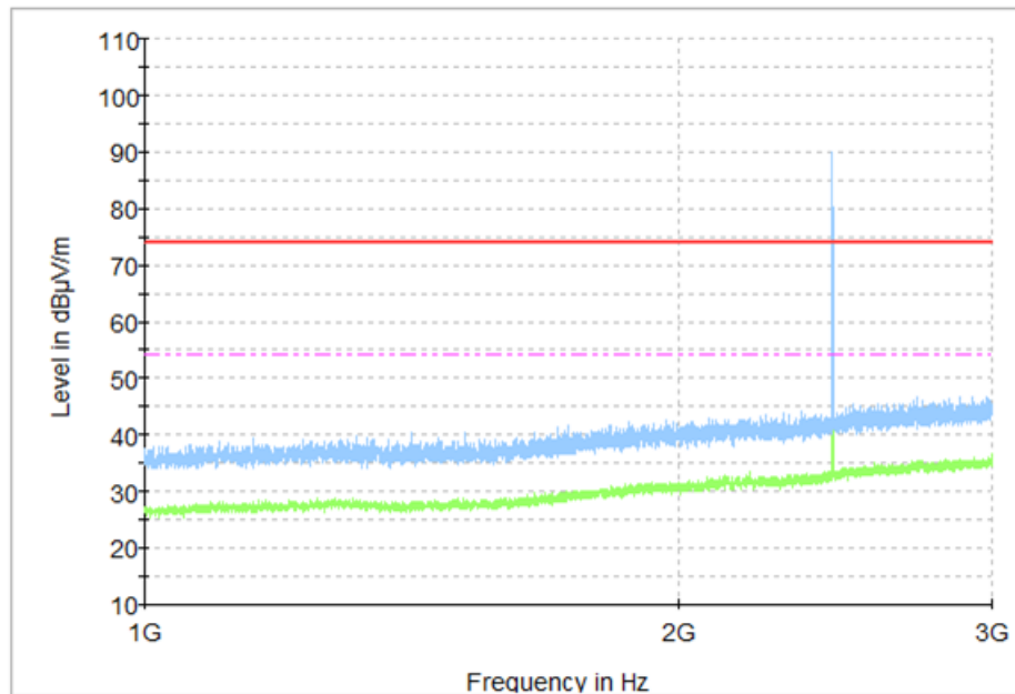
Fig. 35 Radiated Spurious Emission (GFSK, Ch39, 1 GHz ~3 GHz)
