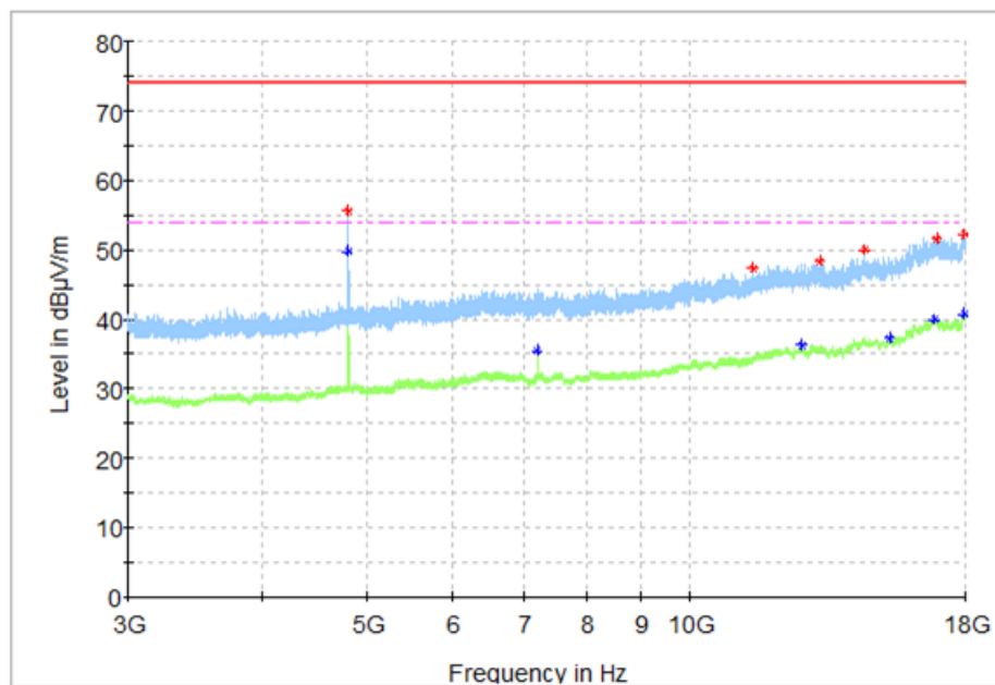
Fig. 42 Radiated Spurious Emission ( \pi/4 DQPSK, Ch0, 3 GHz ~18 GHz)
