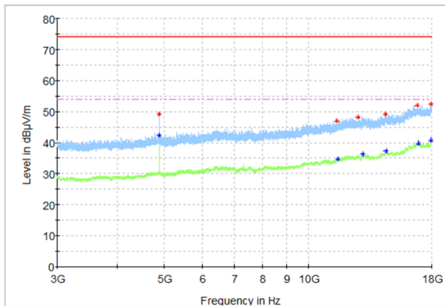
Fig. 44 Radiated Spurious Emission ( \pi/4 DQPSK, Ch39, 3 GHz ~18 GHz)
