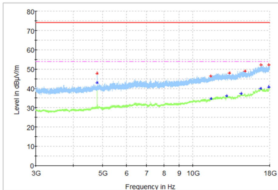
Fig. 50 Radiated Spurious Emission (8DPSK, Ch0, 3 GHz ~18 GHz)
