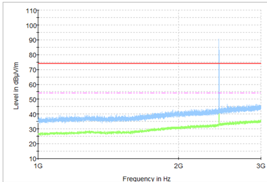
Fig. 51 Radiated Spurious Emission (8DPSK, Ch39, 1 GHz ~3 GHz)
