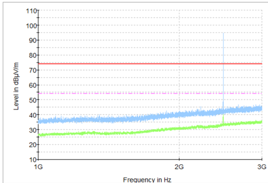
Fig. 37 Radiated Spurious Emission (GFSK, Ch78, 1 GHz ~3 GHz)
