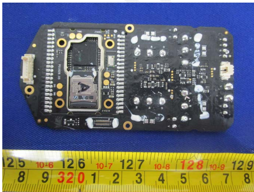
EUT –PCB Bottom Unshielded View
