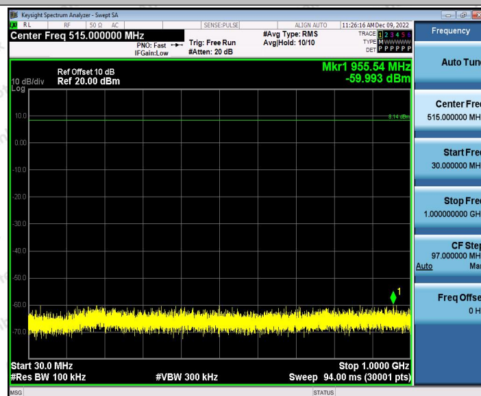
2.4G_Ant2_2441.4_30~1000
