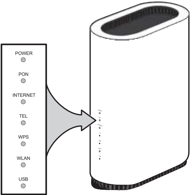
Figure 5-7 G-2426G-B indoor ONT LEDs for NAR variant
