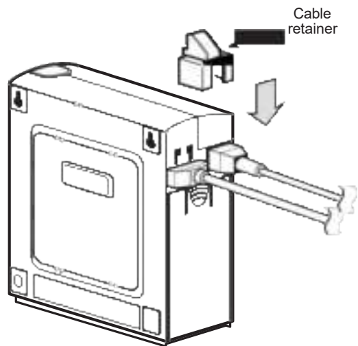
Figure 6-12 Attaching the cable retainer
