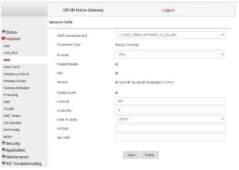
Figure 8-16 WAN page - Route Mode
