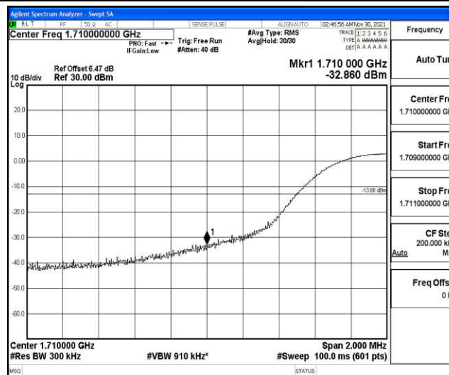
Band4-15MHz-QPSK-20325-75RB#0
