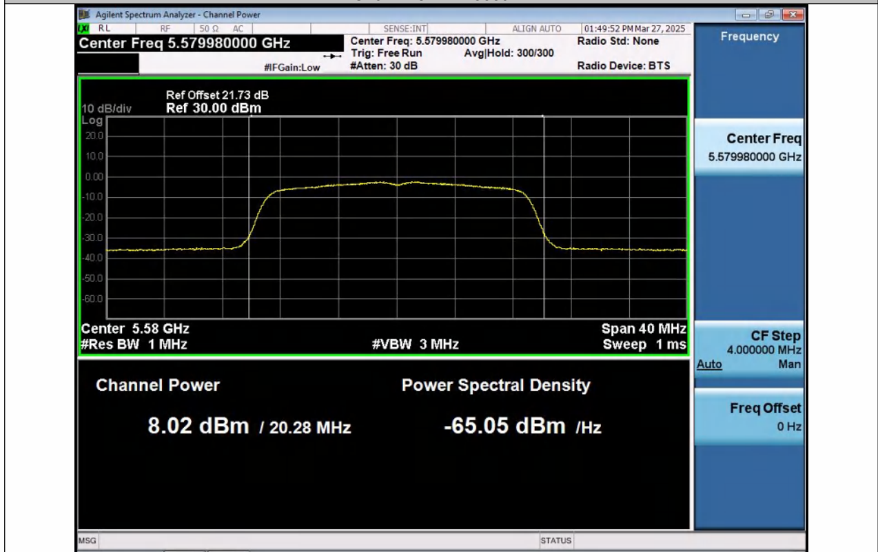
11AC20MIMO-Ant2-5580-PASS
