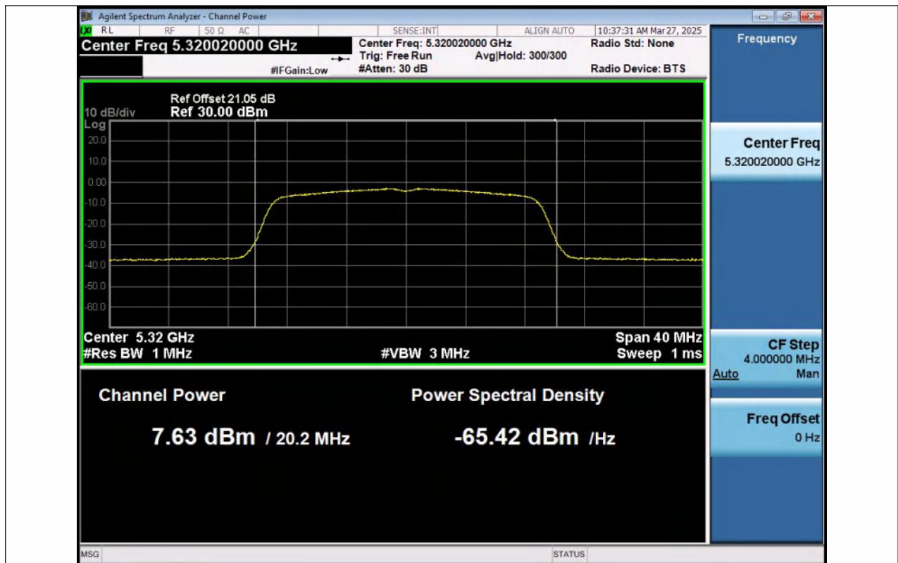
11N20MIMO-Ant1-5320-PASS
