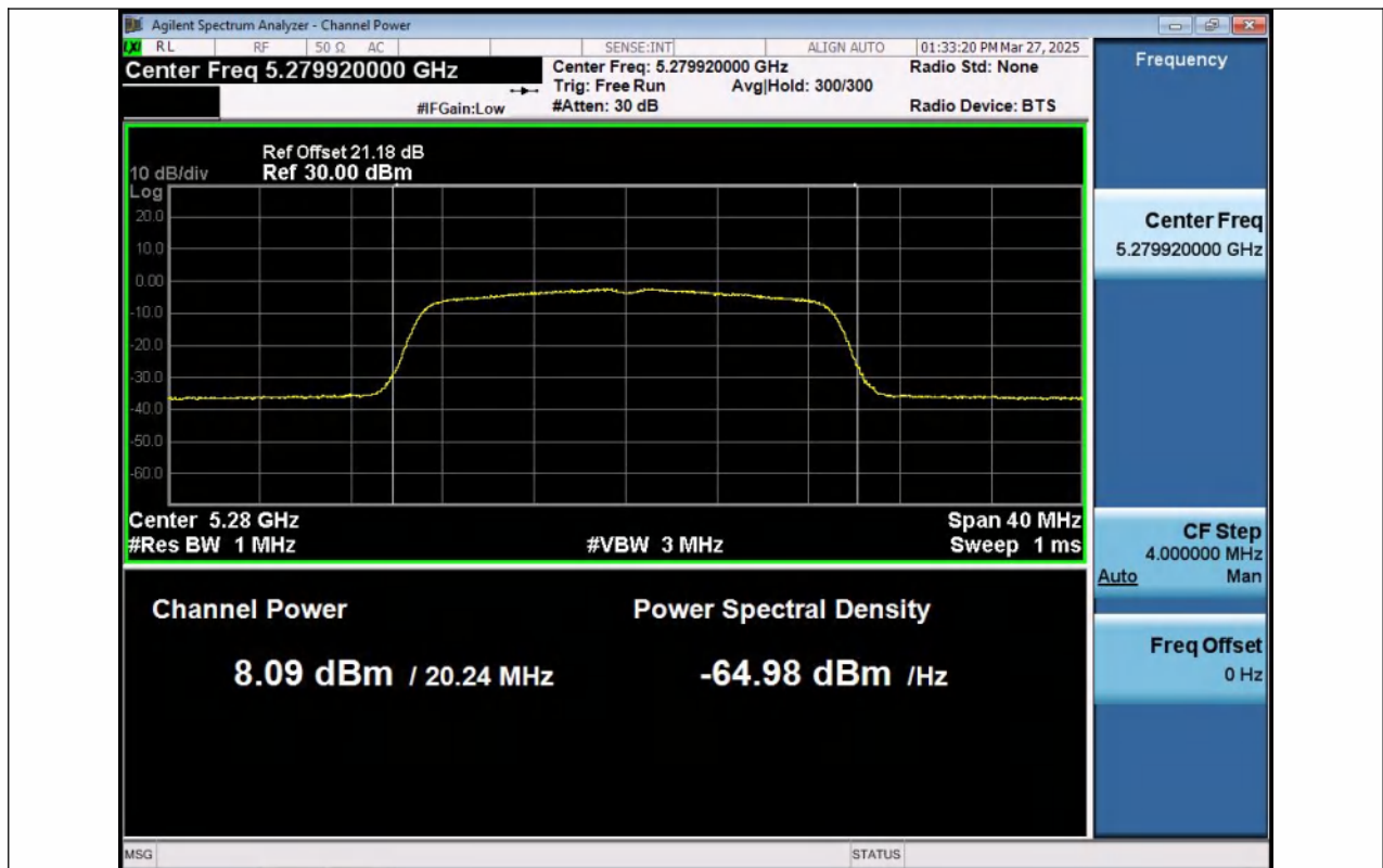
11AC20MIMO-Ant1-5280-PASS
