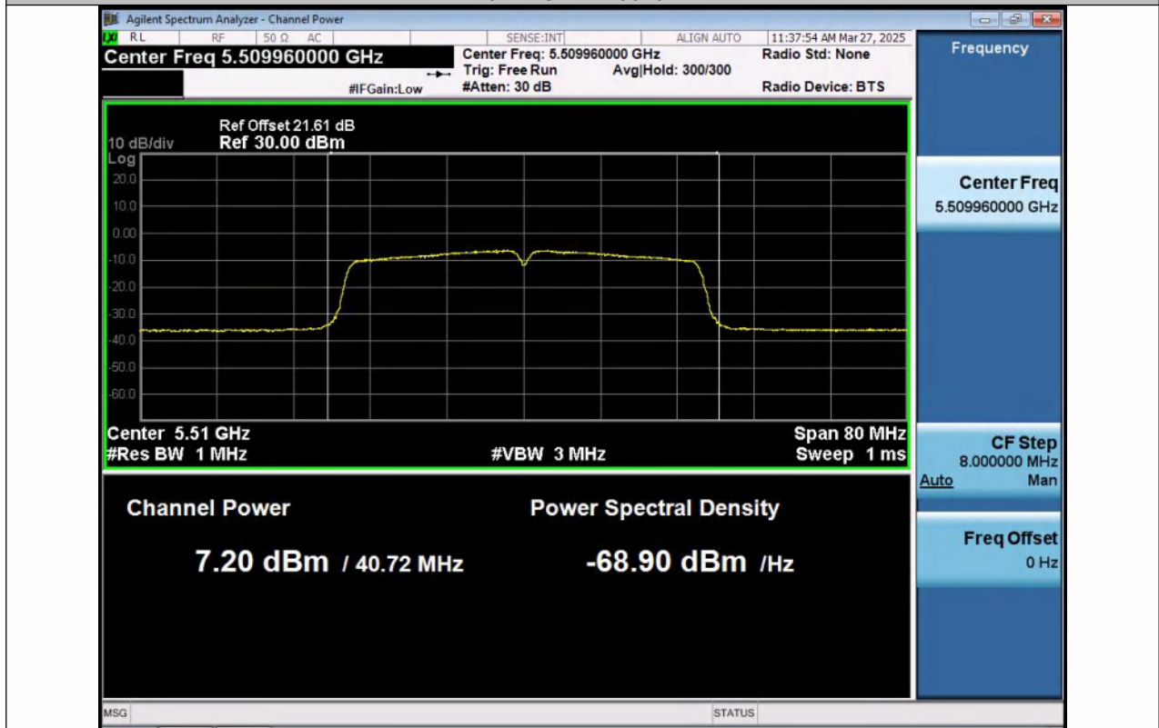
11N40MIMO-Ant2-5510-PASS
