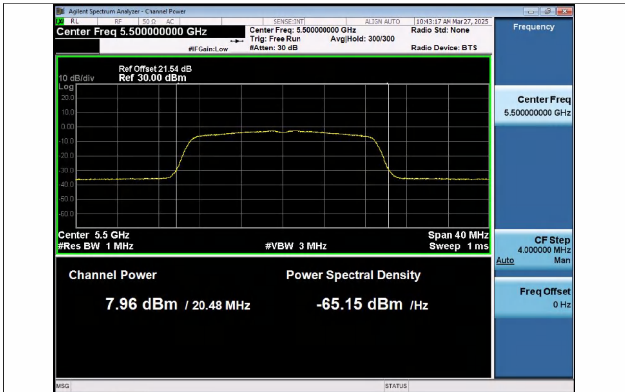
11N20MIMO-Ant1-5500-PASS
