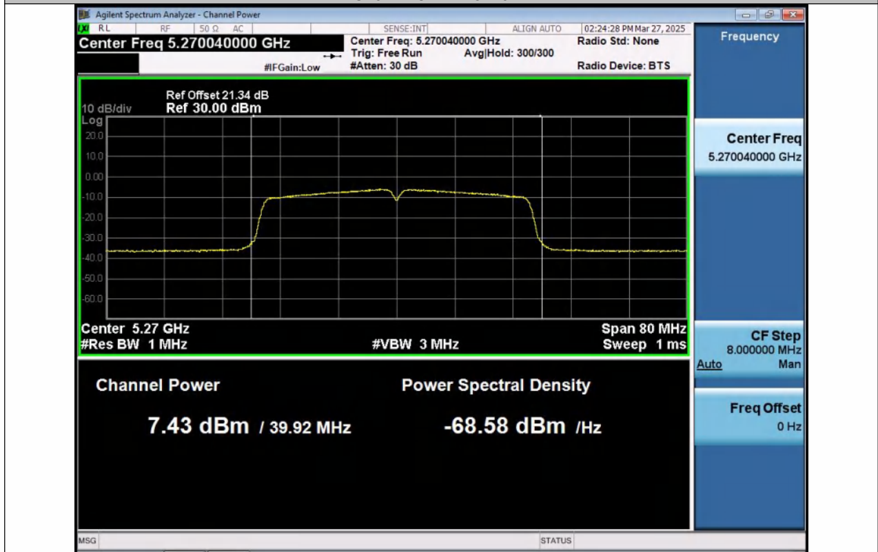
11AC40MIMO-Ant2-5270-PASS
