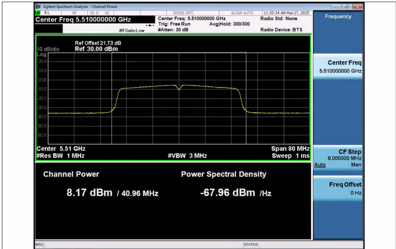
11N40MIMO-Ant1-5510-PASS
