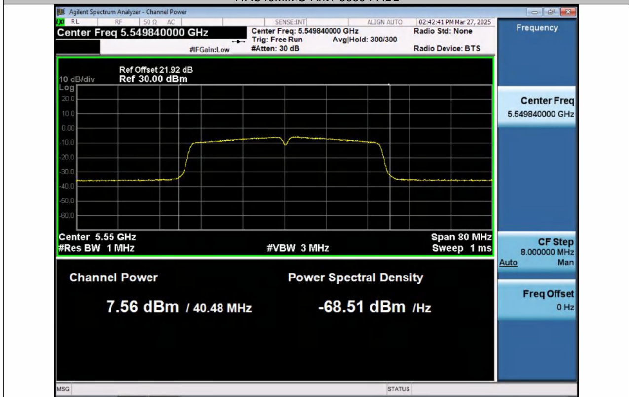
11AC40MIMO-Ant2-5550-PASS
