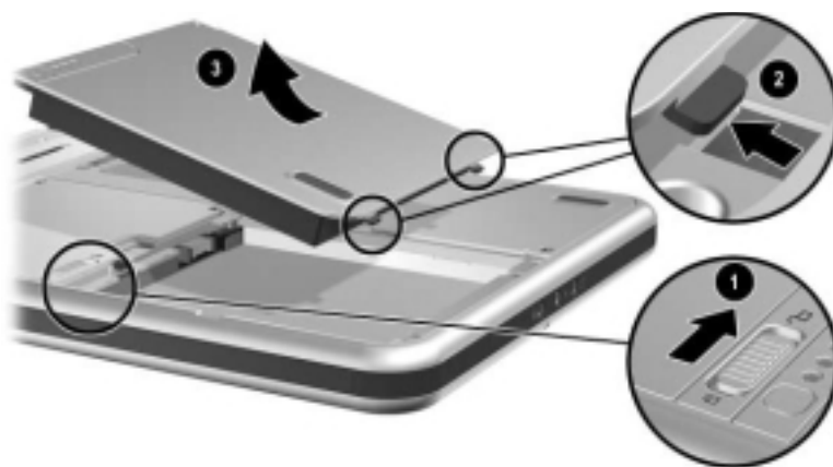
Removing a battery pack
