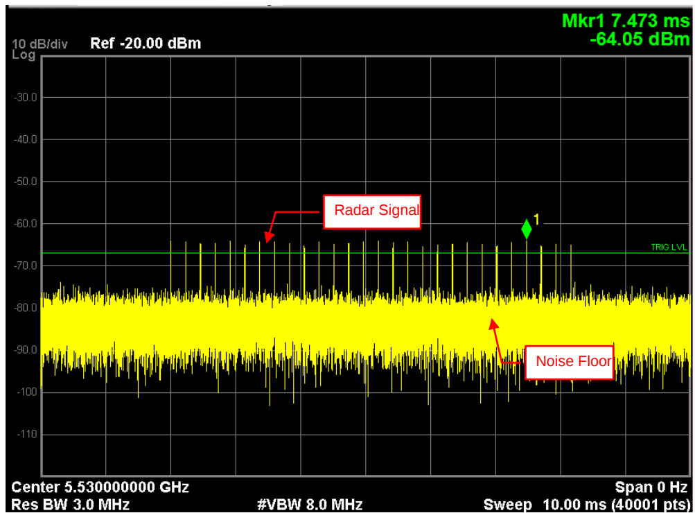
Radar Signal 2
