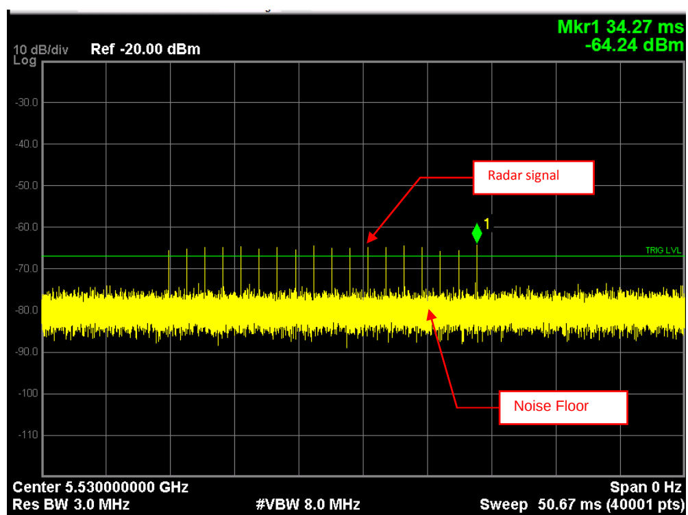
Radar Signal 0
