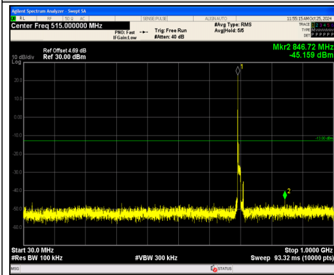
Band12-10MHz-16QAM-23060-1RB#0-Range1:30~1000MHz
