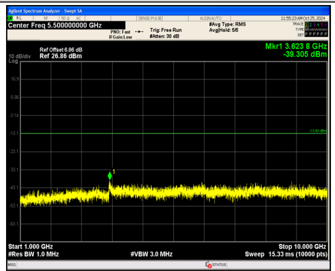
Band12-10MHz-16QAM-23060-1RB#0-Range2:1000~10000MHz
