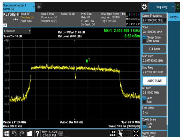
11AX20MIMO-Ant2-2412-106Tone-RU54-PASS
