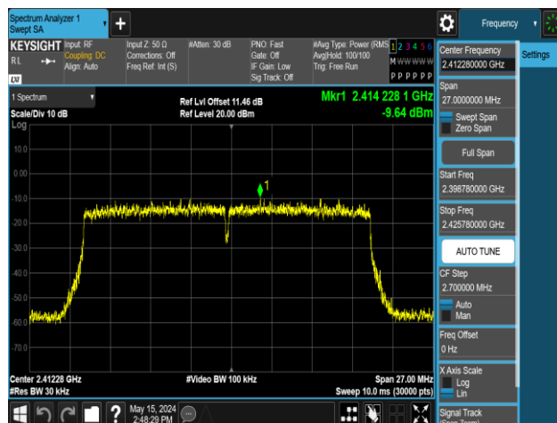
11AX20MIMO-Ant1-2412-106Tone-RU54-PASS
