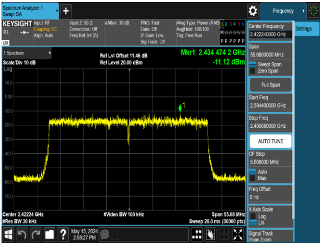
11AX40MIMO-Ant1-2422-242Tone-RU62-PASS
