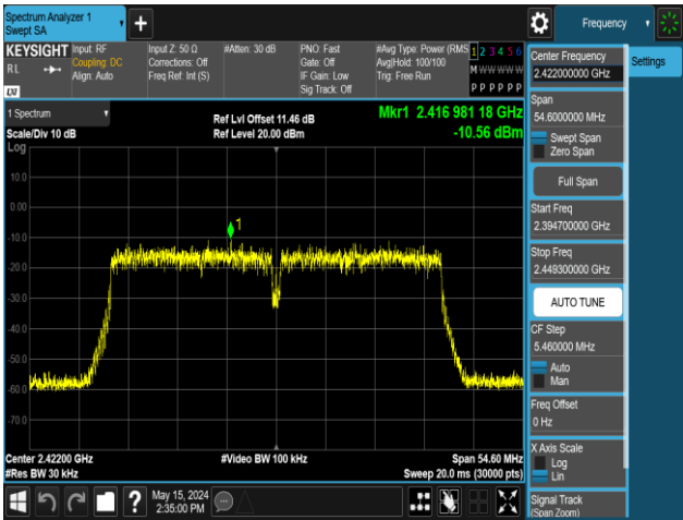
11N40MIMO-Ant1-2422-PASS
