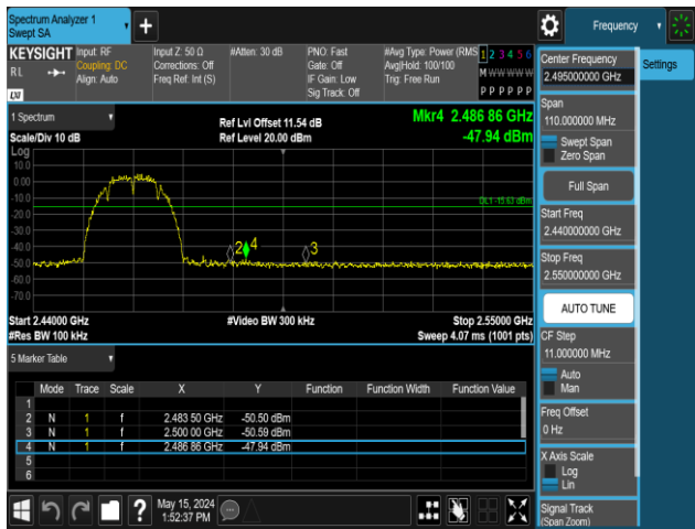
11B-Ant1-2462-PASS
