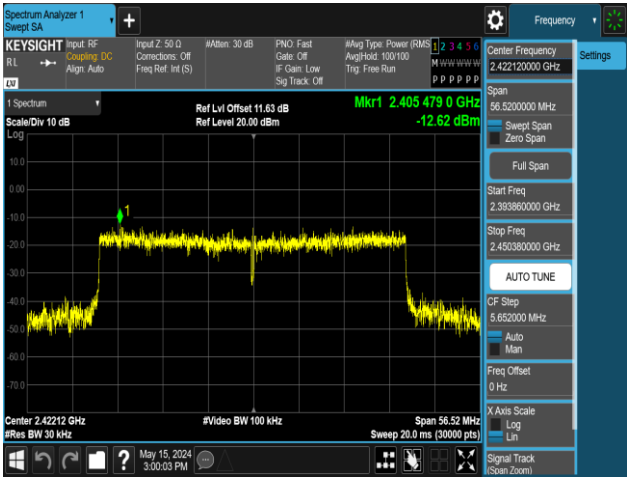
11AX40MIMO-Ant2-2422-242Tone-RU62-PASS
