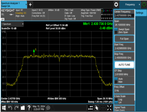
11N20MIMO-Ant1-2437-PASS
