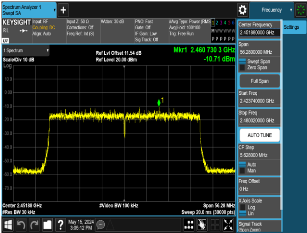
11AX40MIMO-Ant1-2452-242Tone-RU62-PASS
