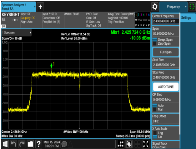
11AX40MIMO-Ant1-2437-242Tone-RU62-PASS
