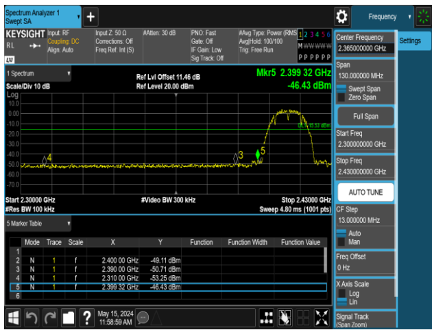
11B-Ant1-2412-PASS
