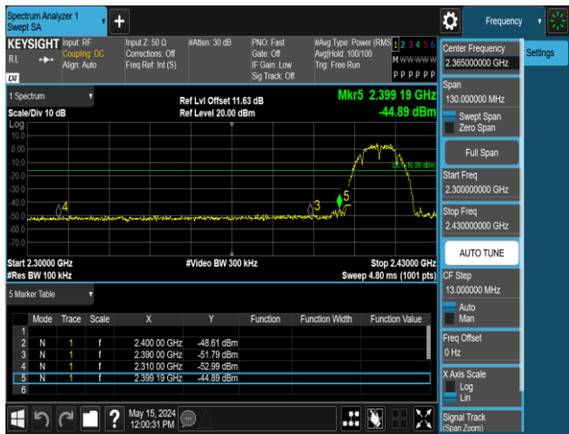
11B-Ant2-2412-PASS
