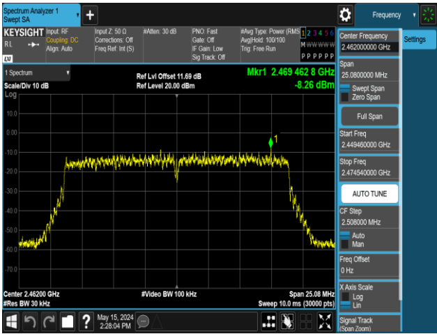
11N20MIMO-Ant2-2462-PASS
