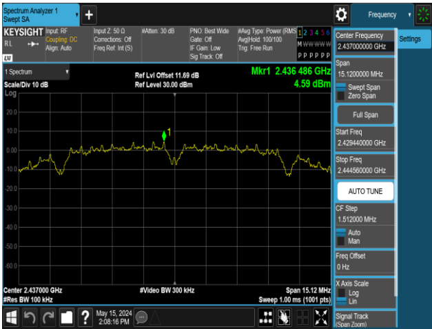
11B-Ant2-2437-PASS
