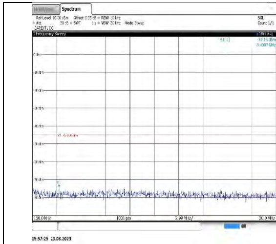
Band41_10MHz_16QAM_39700_1RB#0_1000~2000_00_1000~20000
