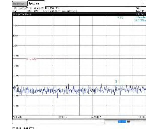
Band66-15MHz-16QAM-132047-1RB#0-Range1:30~1000MHz
