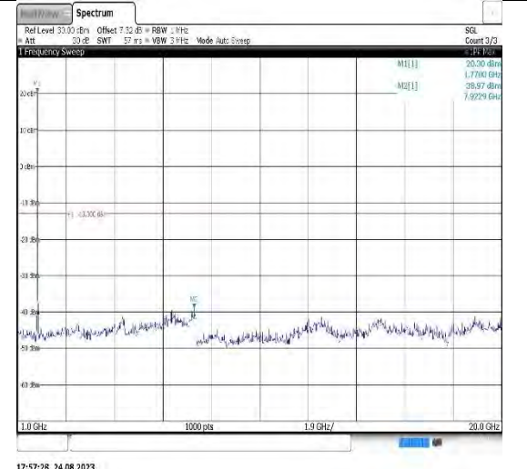
Band66-15MHz-16QAM-132047-1RB#0-Range2:1000~20000MHz
