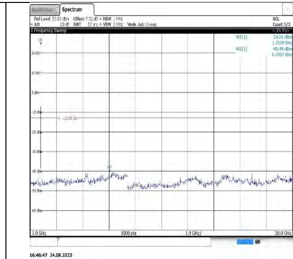
Band66-3MHz-16QAM-132657-1RB#0-Range2:1000~20000MHz
