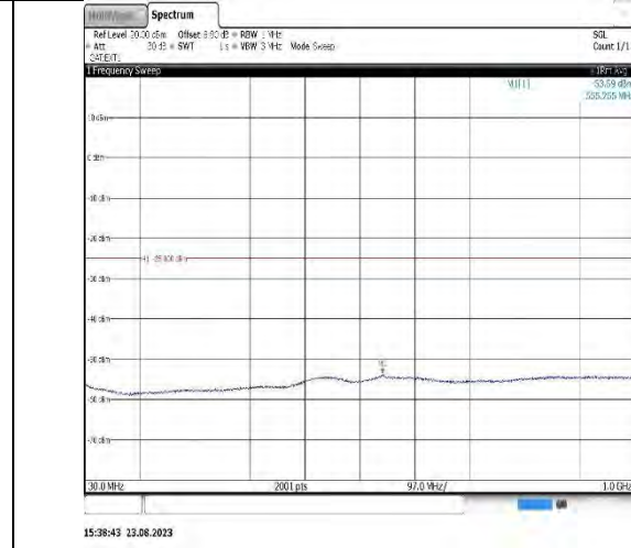
Band41_5MHz_16QAM_41565_1RB#0_20000~2700_0_20000~27000
