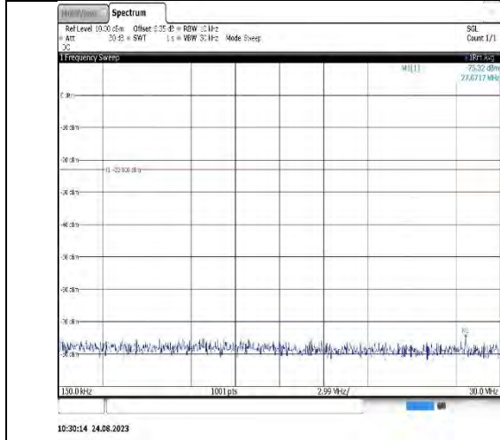
Band26_10MHz_16QAM_26915_1RB#0_1000~300_0_1000~3000
