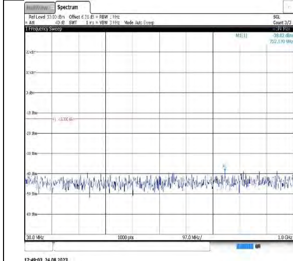
Band66-10MHz-16QAM-132322-1RB#0-Range1:30~1000MHz
