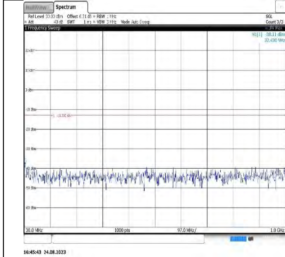
Band66-3MHz-QPSK-132322-1RB#0- Range1:30~1000MHz
