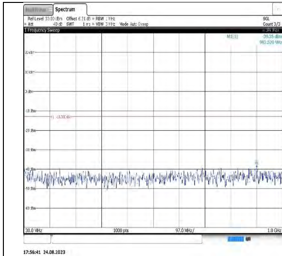
Band66-15MHz-QPSK-132597-1RB#0-Range1:30~1000MHz
