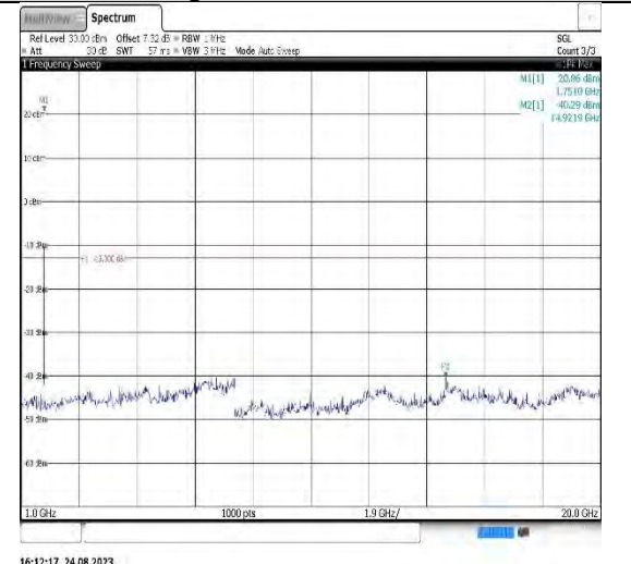
Band66-1.4MHz-QPSK-132665-1RB#0-Range2:1000~20000MHz
