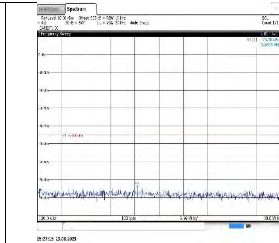
Band41_5MHz_QPSK_39675_1RB#0_1000~20000_1000~20000
