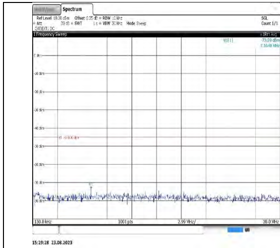
Band41_5MHz_16QAM_39675_1RB#0_1000~2000_0_1000~20000
