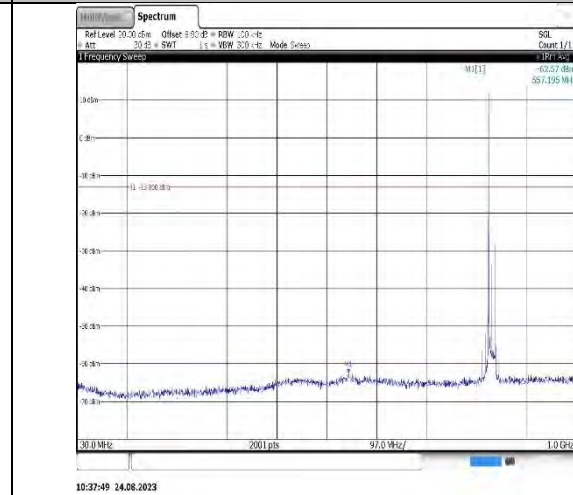
Band26_15MHz_16QAM_26915_1RB#0_3000~1000_0_3000~10000
