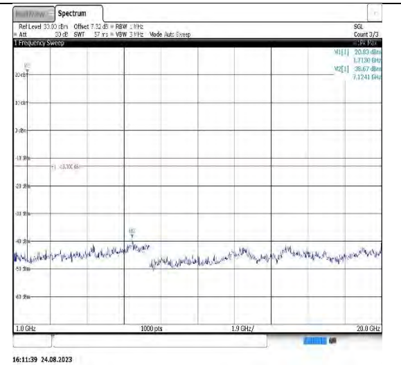
Band66-1.4MHz-QPSK-132322-1RB#0-Range2:1000~20000MHz
