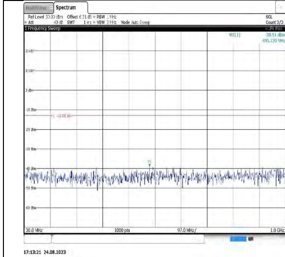
Band66-5MHz-16QAM-132647-1RB#0-Range1:30~1000MHz
