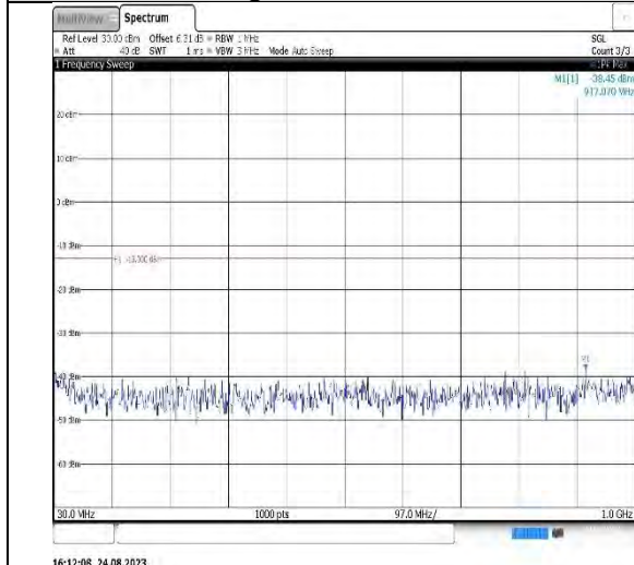
Band66-1.4MHz-QPSK-132665-1RB#0-Range1:30~1000MHz
