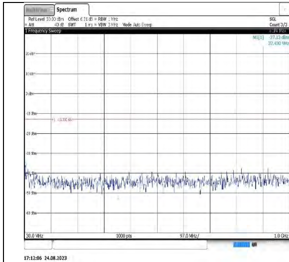
Band66-5MHz-16QAM-132322-1RB#0-Range1:30~1000MHz
