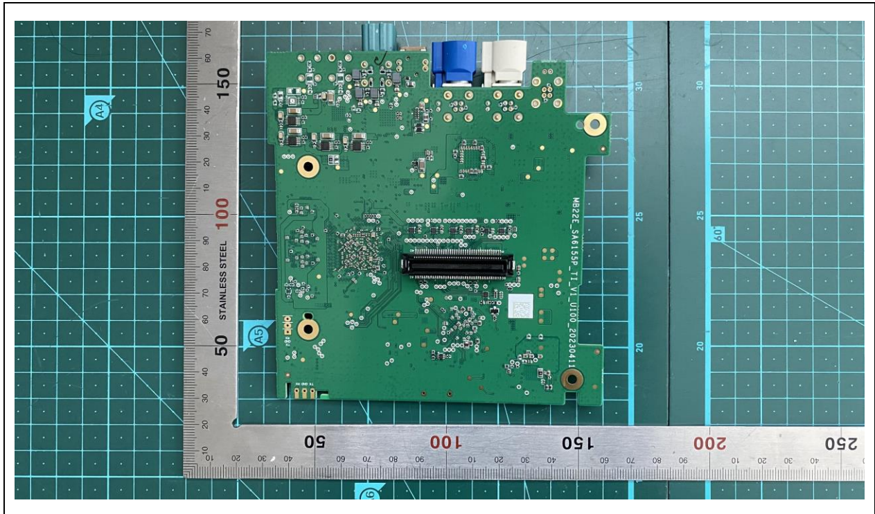
RF PCB Rear
