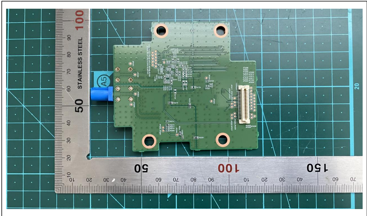
DAB PCB Rear
