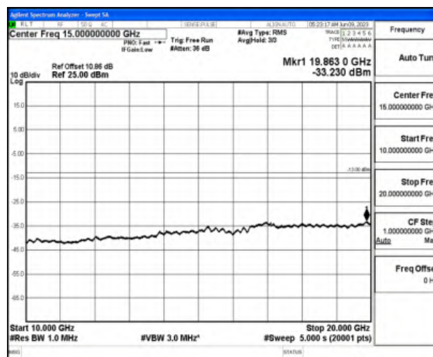
Band2-20MHz-16QAM-19100-1RB#0-Range5:10000~20000MHz
