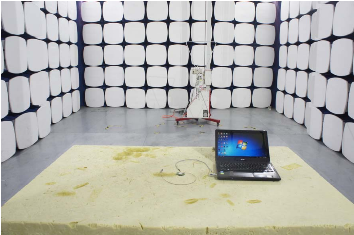
Radiated Emission Above 1G Test Photo
