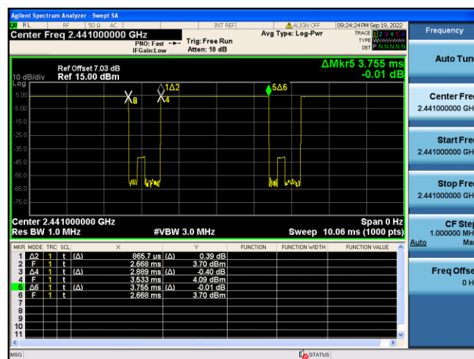
Bluetooth-GFSK
