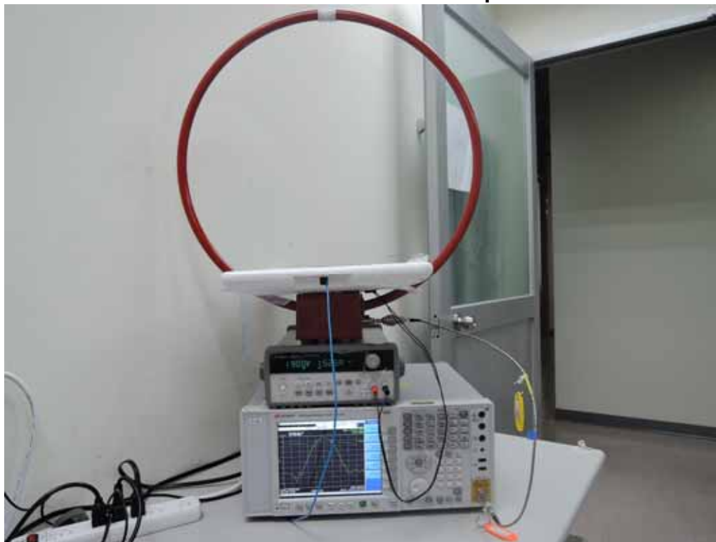
Bandwidth measurement Setup Photo
