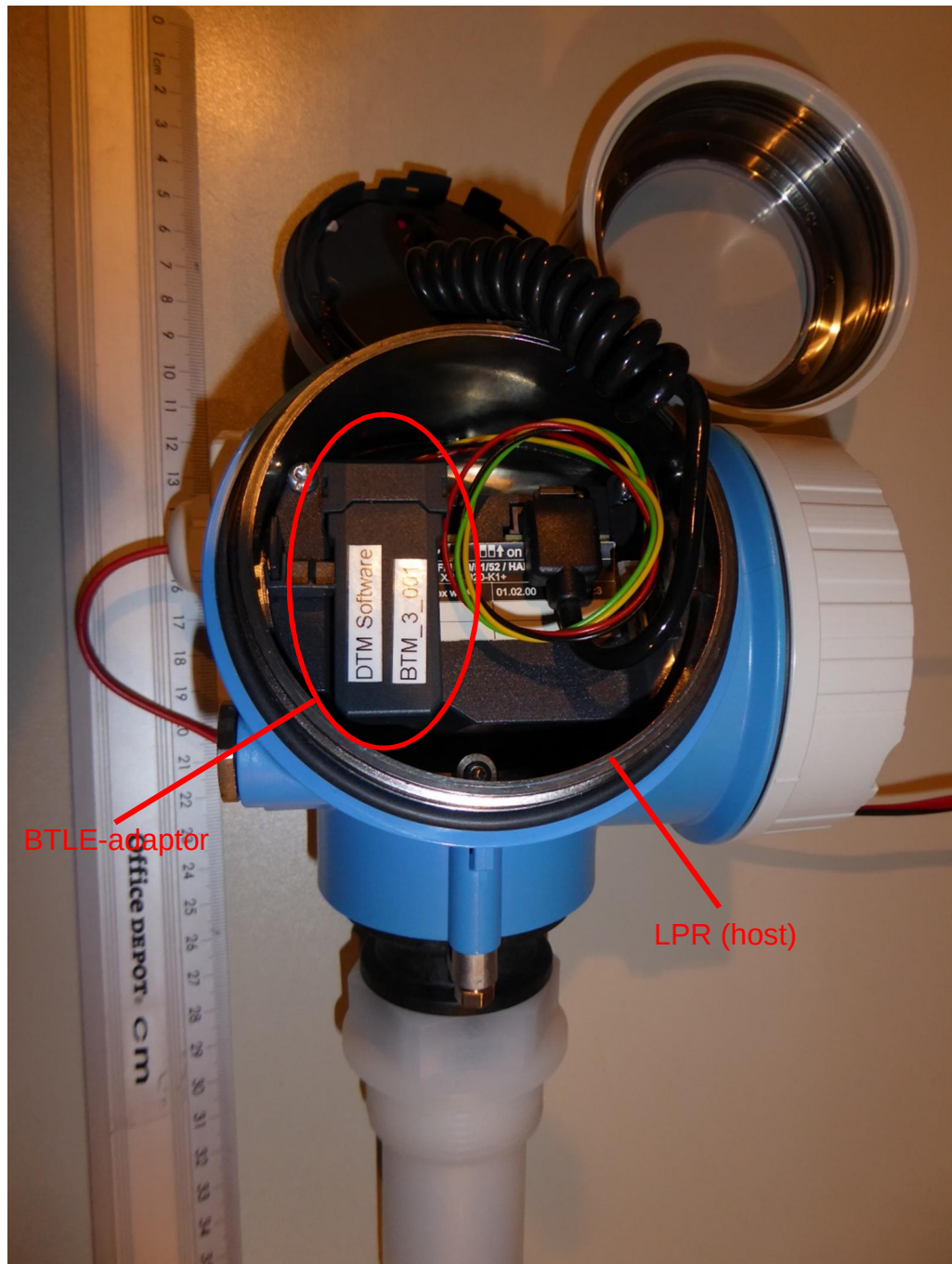
172289_e.JPG: ProToF BTLE-adaptor 2.4 GHz inside FMR50, internal view to mounted BTLE module (display removed)
