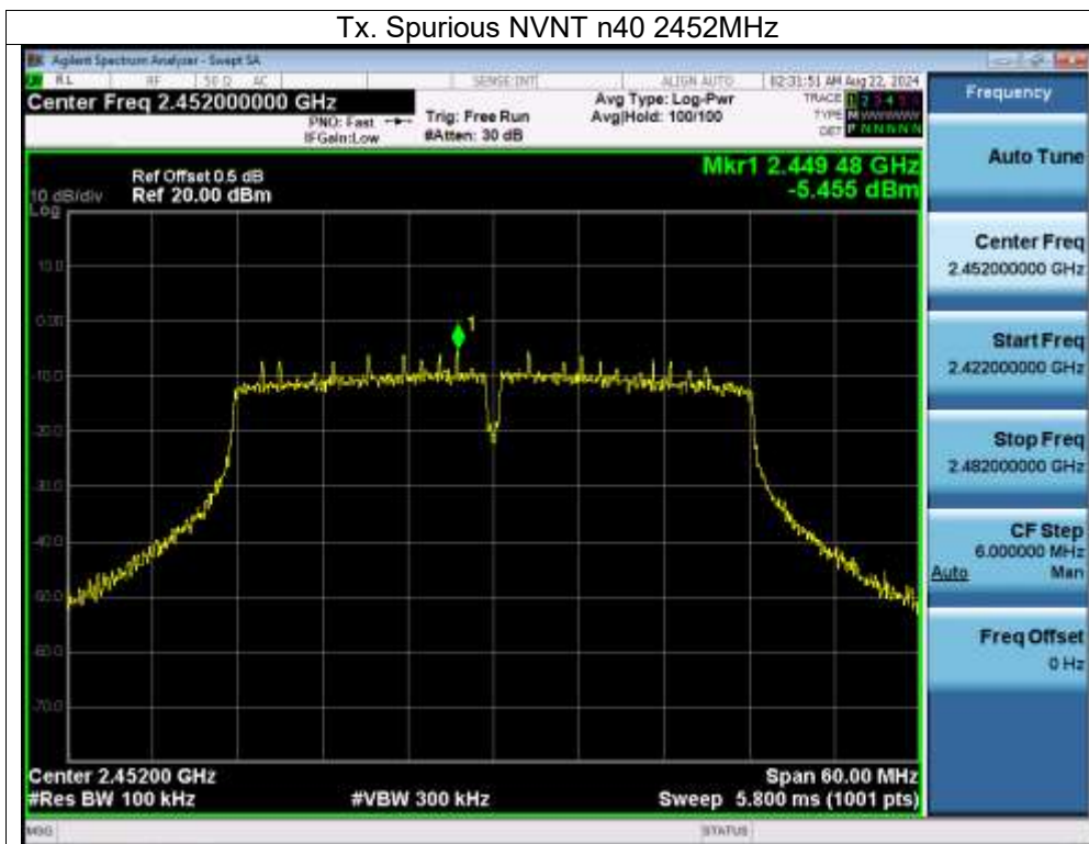
Tx. Spurious NVNT n40 2452MHz Emission
