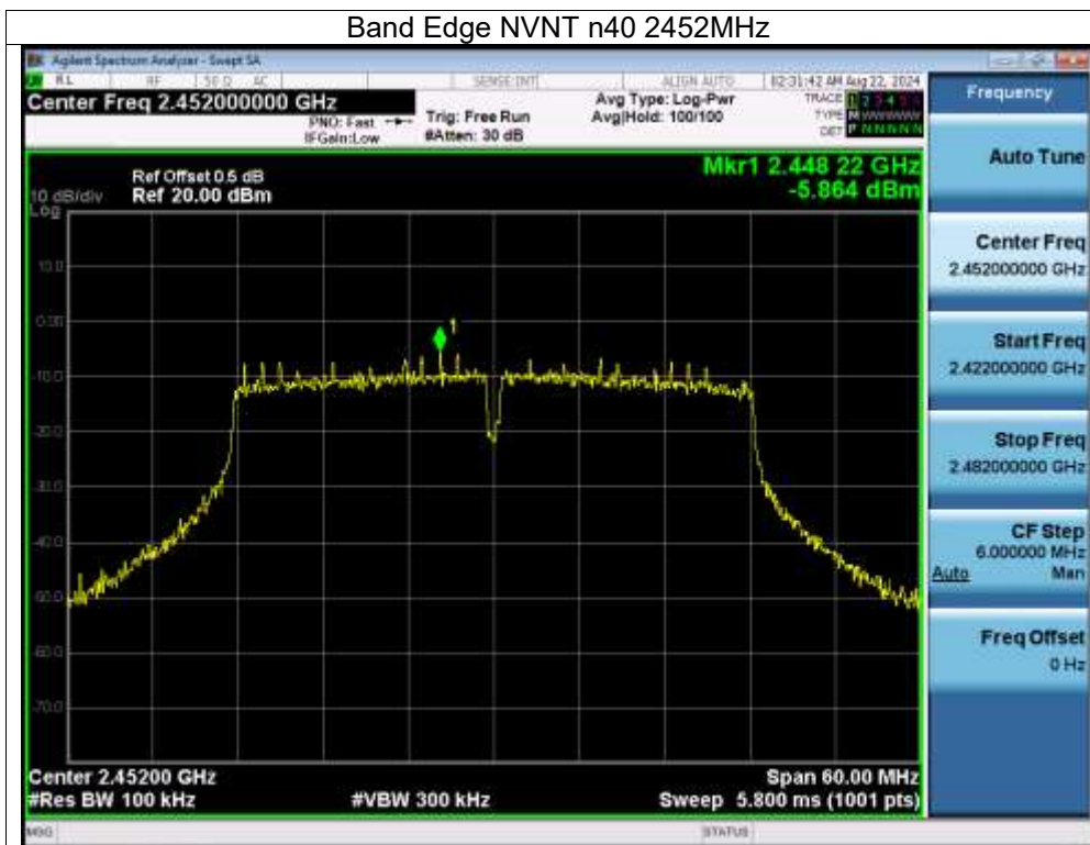
Band Edge NVNT n40 2452MHz Emission
