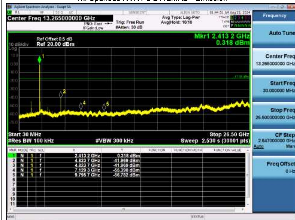
Tx. Spurious NVNT b 2412MHz Emission
