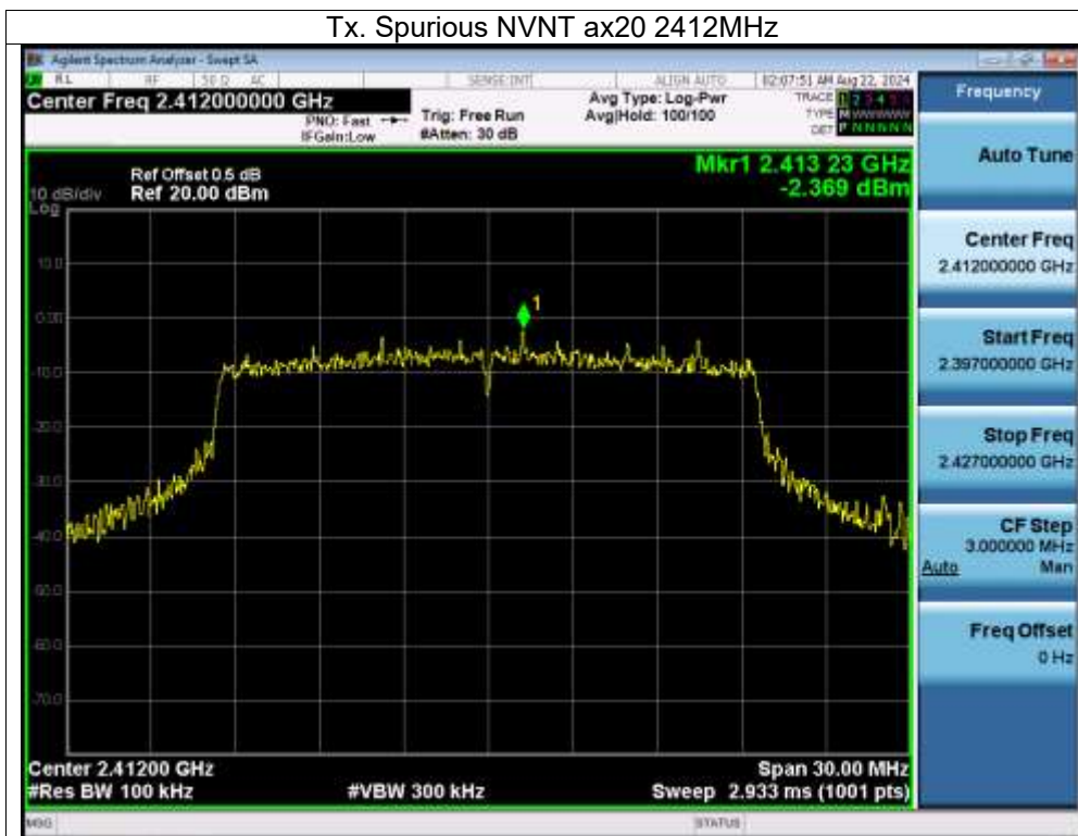
Tx. Spurious NVNT ax20 2412MHz Emission
