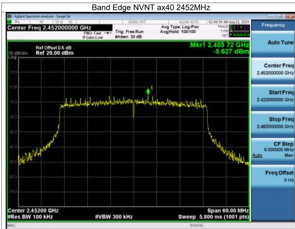
Band Edge NVNT ax40 2452MHz Emission
