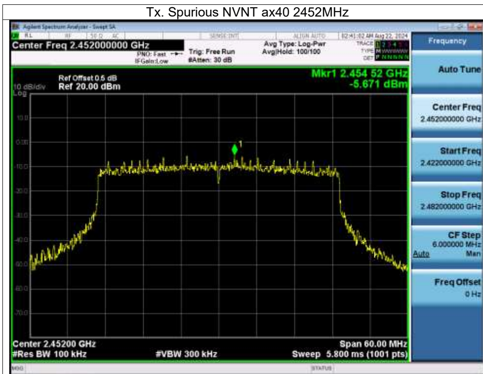
Tx. Spurious NVNT ax40 2452MHz Emission
