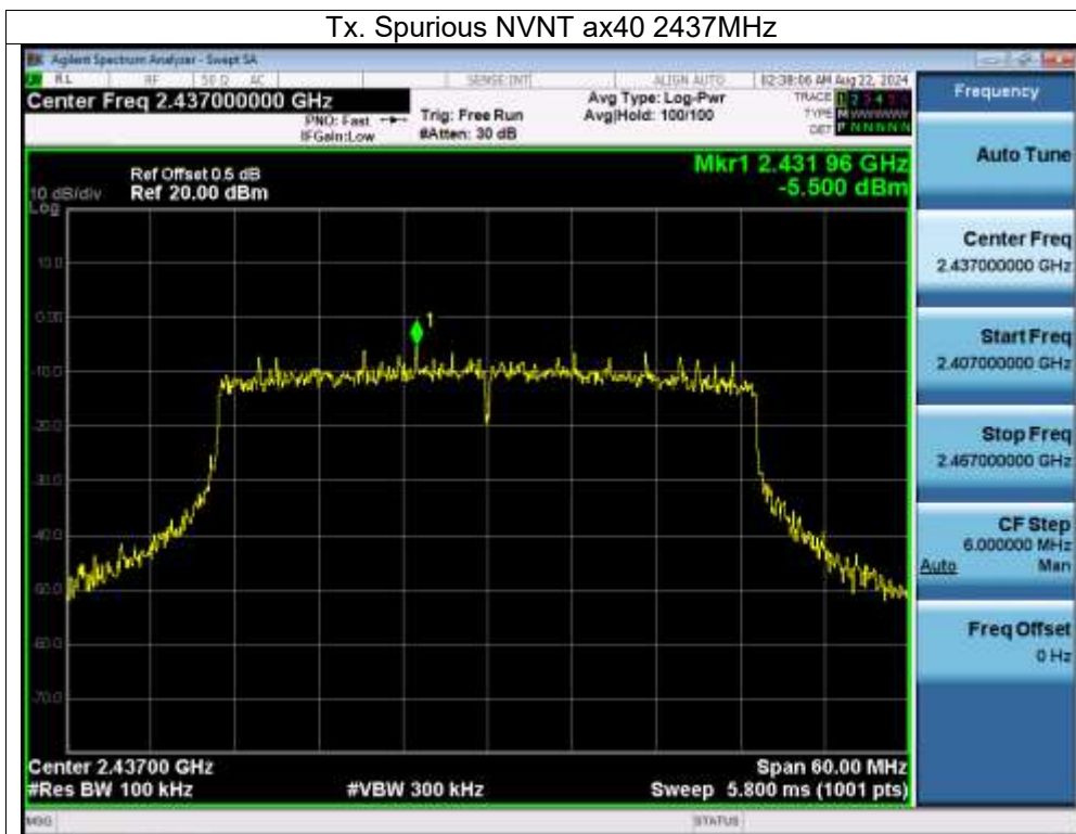
Tx. Spurious NVNT ax40 2437MHz Emission
