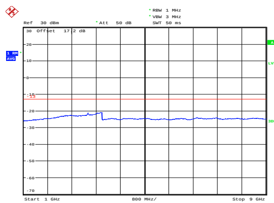
LTE Band 5 1.4MHz CH-Middle 1GHz~9GHz
