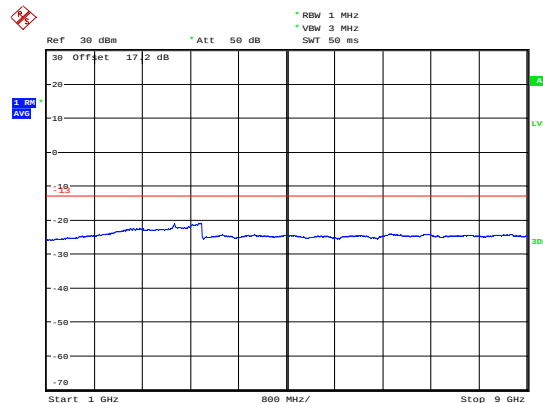
LTE Band 5 1.4MHz CH-High 1GHz~9GHz
