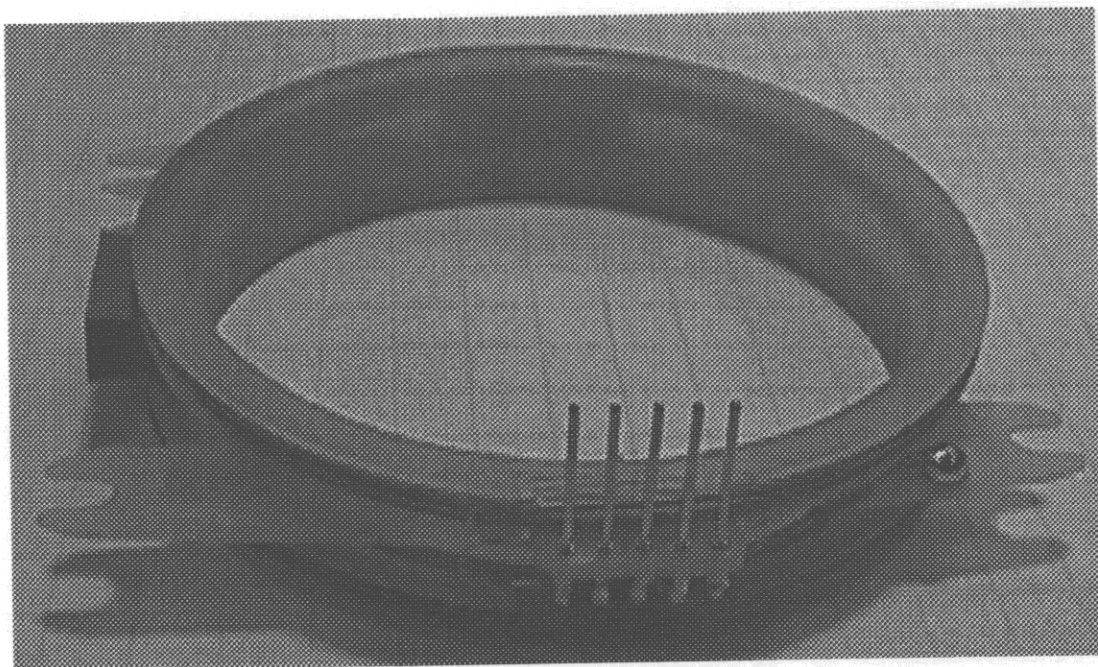
Figure 8: Close Coupled Coil (Top Side)
