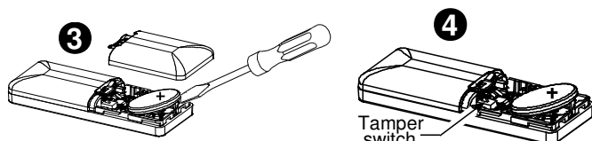
Fig. 4 – Battery Replacement
