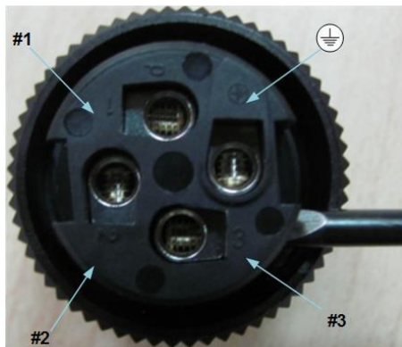
Figure 43: Numbered connector contacts
