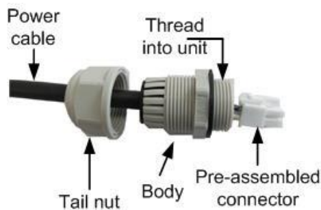
Figure 35: Power cable assembly
