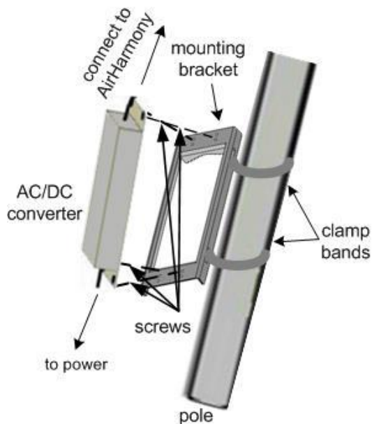
Figure 29: Pole mounting – exploded view
