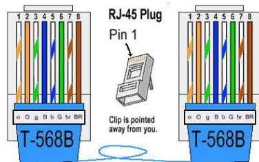
Figure 55: RJ45 wire positioning
