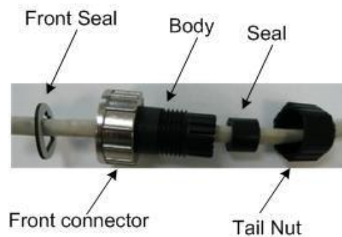
Figure 53: Ethernet cable thru connector
