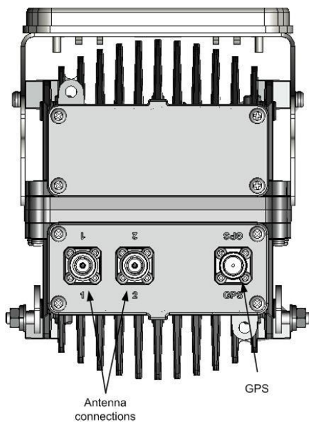
Figure 5: AirHarmony-1000 Unit, Top, RF ports
