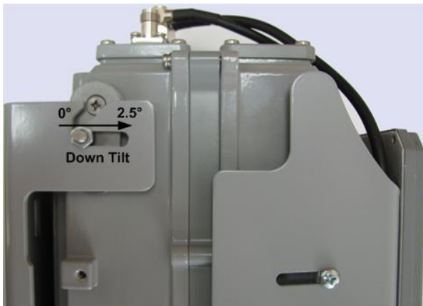
Figure 22: Tilt adjustment body
