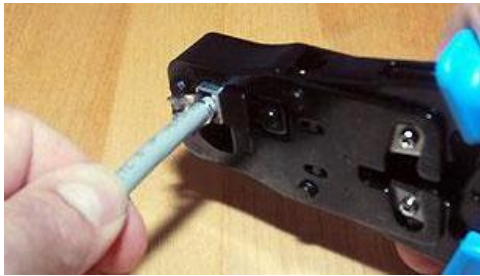
Figure 58: RJ45 crimping
