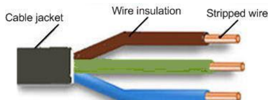
Figure 38: AC power cable preparation
