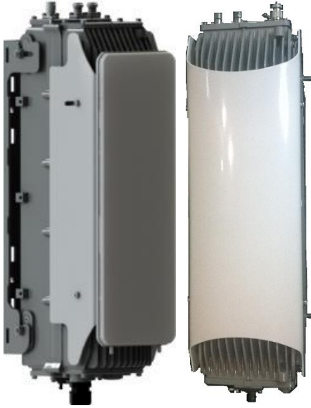
Figure 1: AirHarmony-1000 with front mounted antenna and AirHarmony-1000 with sun-shield
