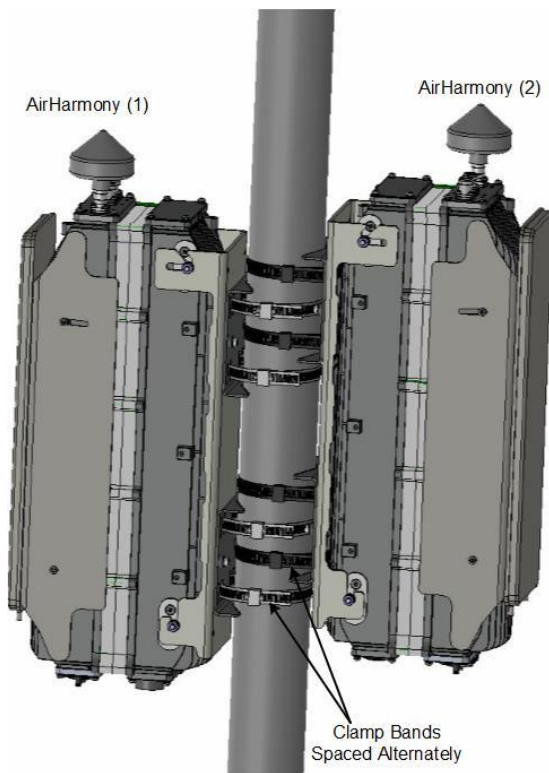
Figure 16: Back-2-Back Assembly
