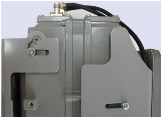
Figure 20: unit engages into slots on the top of mounting plate
