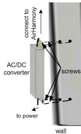
Figure 30: Wall mount – exploded view
