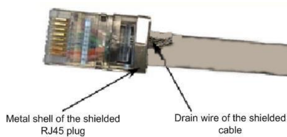
Figure 59: Crimped cable
