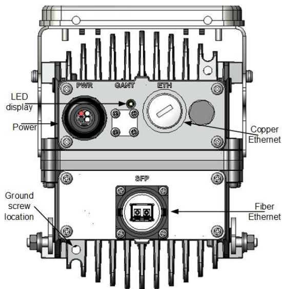
Figure 4: AirHarmony-1000 Unit, bottom termination
