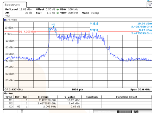
RU 26T offset 0 / 2 437 MHz
