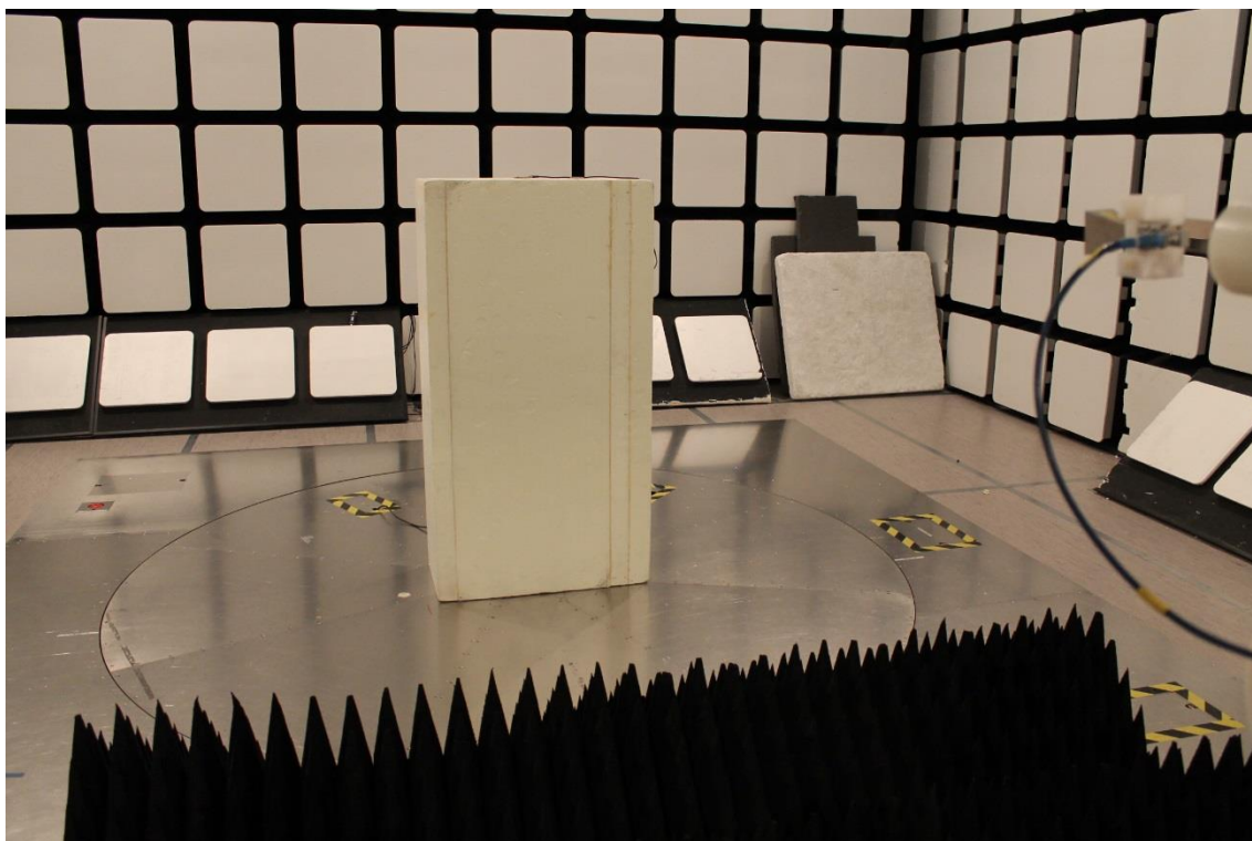
Photograph 5. Radiated Spurious Emissions 18 – 26.5 GHz
