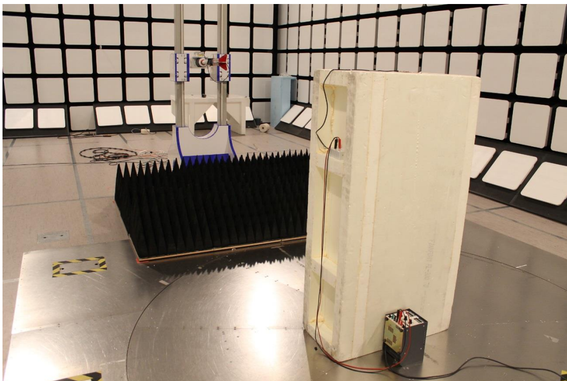
Photograph 4. Radiated Spurious Emissions 1 – 18 GHz
