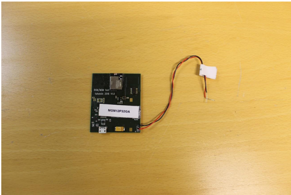
Photograph 1. DUT 1
