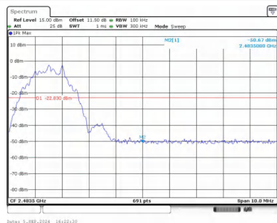
Out Of Band Emission BLE 2M_Channel 39
