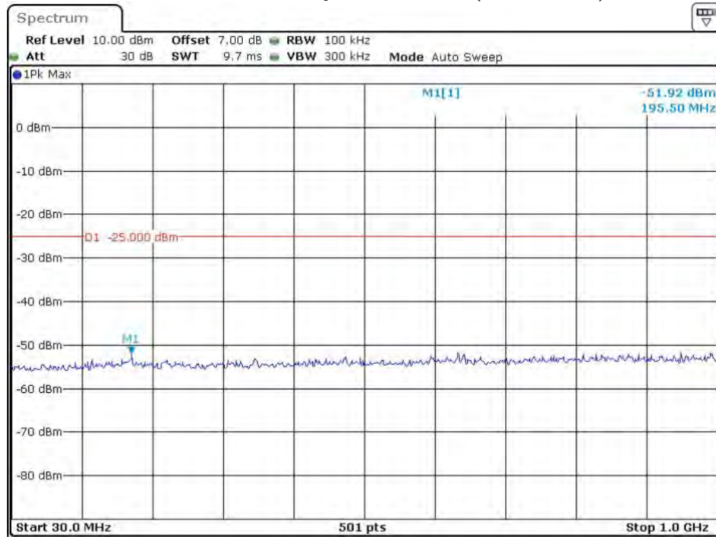
Band 7_20 MHz_Low_QPSK_RB100#0_1(30MHz-1GHz)
