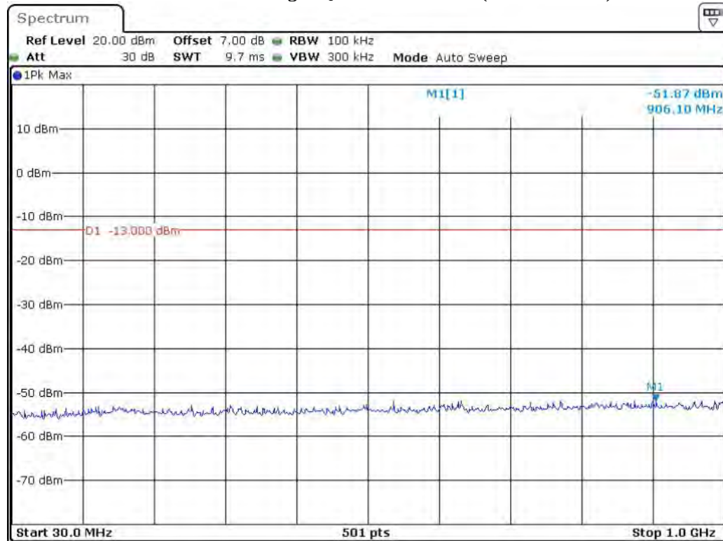
Band 2_20 MHz_High_QPSK_RB100#0_1(30MHz-1GHz)
