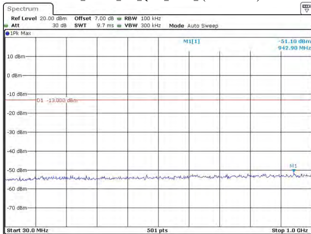
Band 2_1.4 MHz_Low_QPSK_RB6#0_1(30MHz-1GHz)
