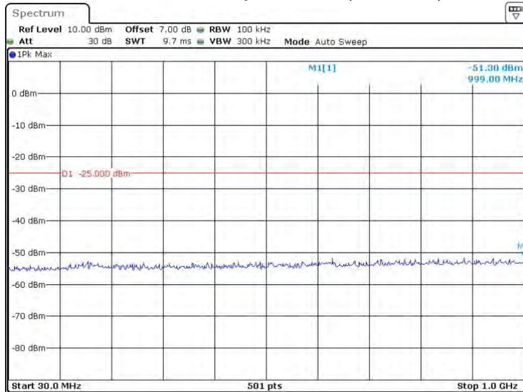
Band 7_5 MHz_Middle_QPSK_RB25#0_1(30MHz-1GHz)
