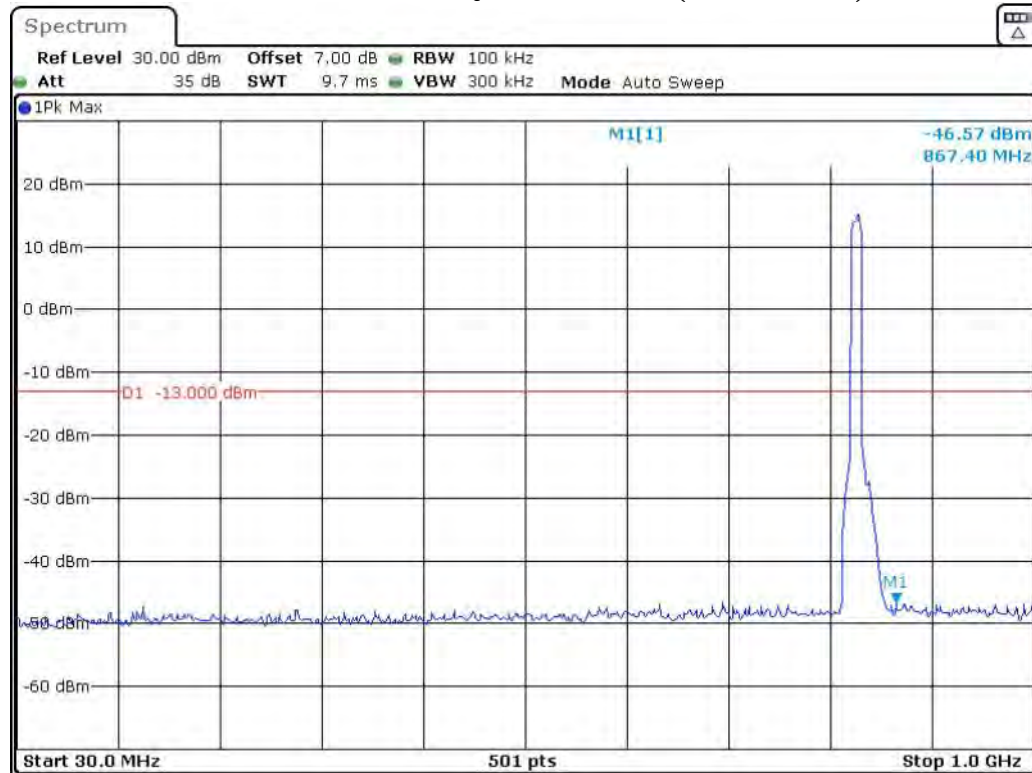
Band 5_10 MHz_Low_QPSK_RB50#0_1(30MHz-1GHz)
