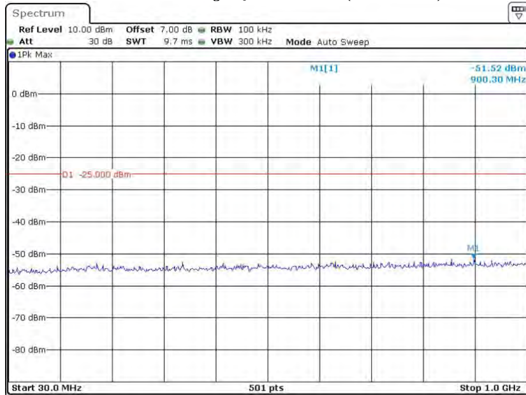
Band 7_10 MHz_High_QPSK_RB50#0_1(30MHz-1GHz)
