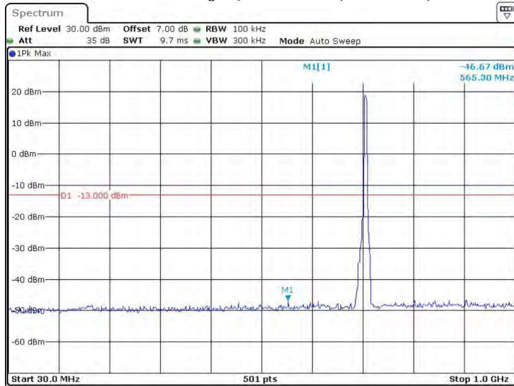
Band 17_5 MHz_High_QPSK_RB25#0_1(30MHz-1GHz)
