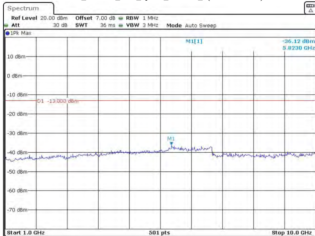
Band 5_10 MHz_Low_QPSK_RB50#0_2(1GHz-10GHz)
