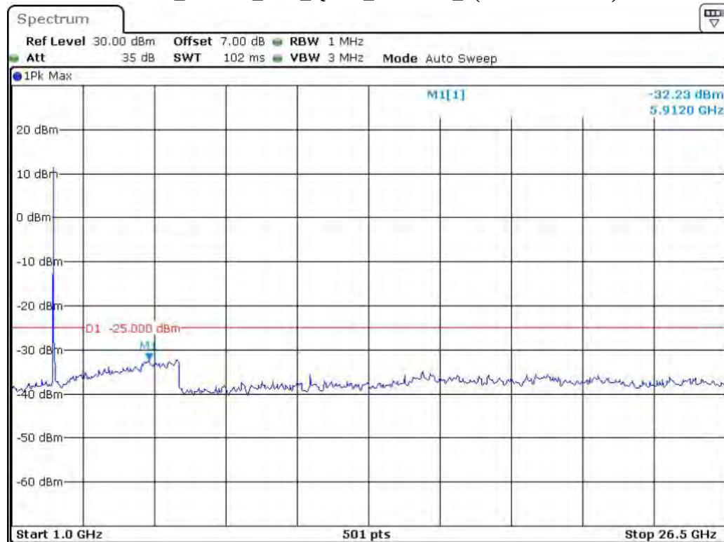
Band 7_20 MHz_Low_QPSK_RB100#0_2(1GHz-26.5GHz)
