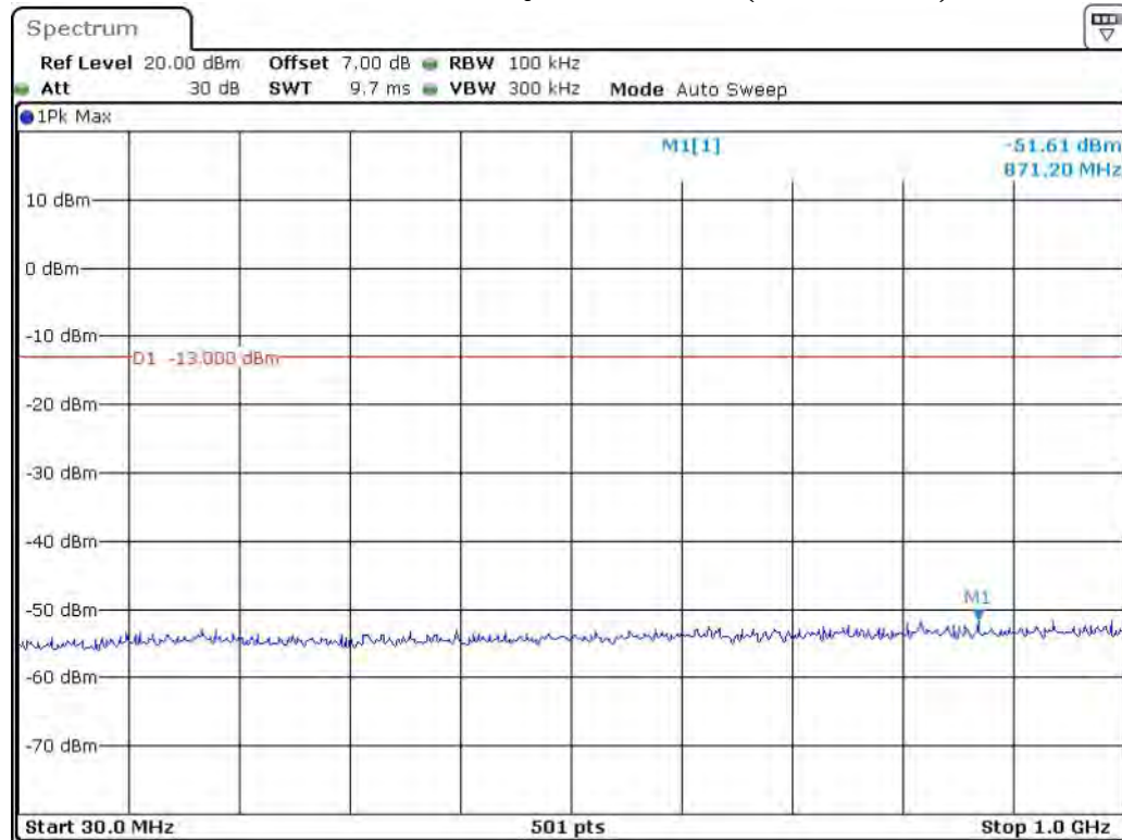
Band 2_3 MHz_Middle_QPSK_RB15#0_1(30MHz-1GHz)
