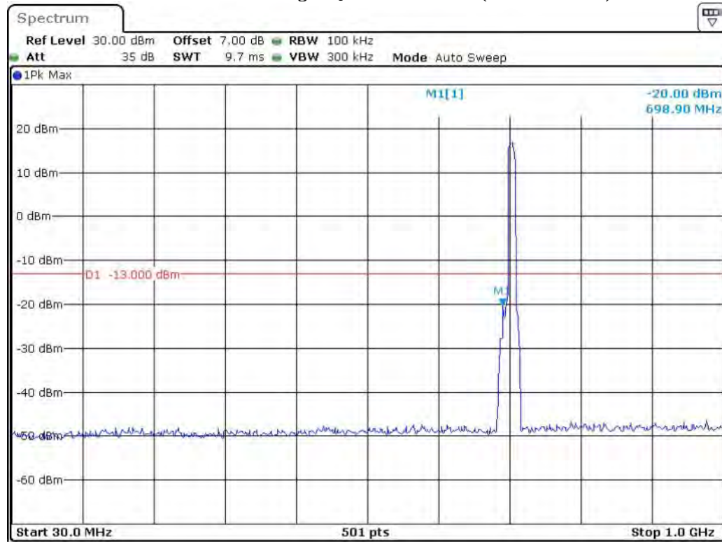
Band 17_10 MHz_High_QPSK_RB50#0_1(30MHz-1GHz)
