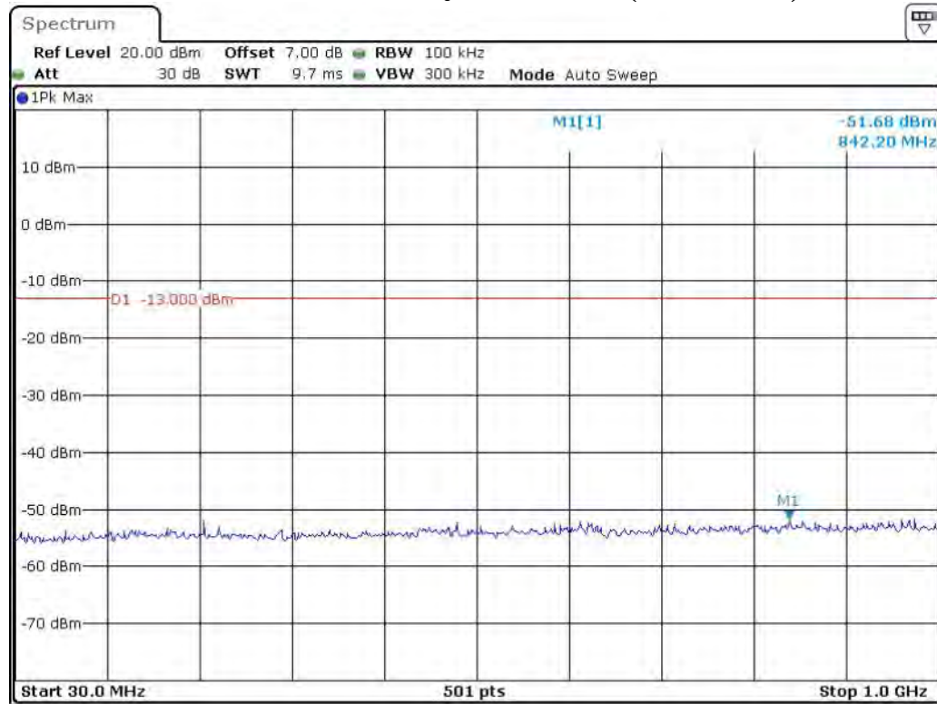
Band 2_10 MHz_Middle_QPSK_RB50#0_1(30MHz-1GHz)
