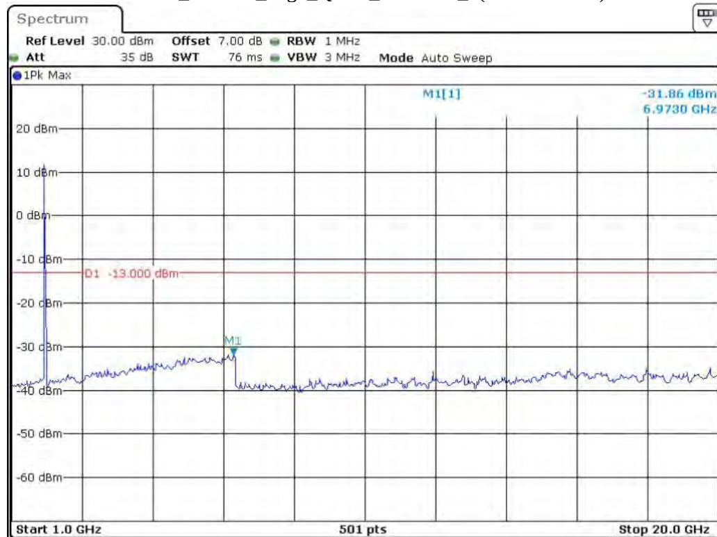
Band 2_20 MHz_High_QPSK_RB100#0_2(1GHz-20GHz)
