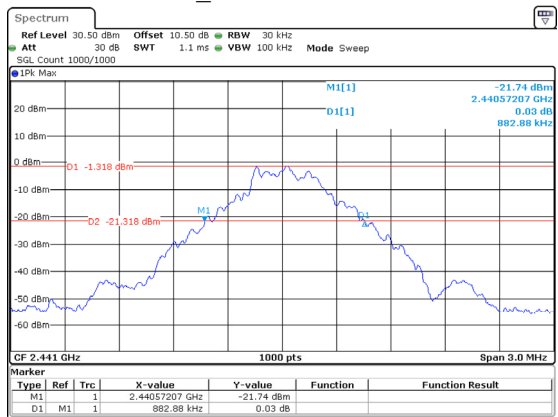
DH1_Middle 0.883MHz
