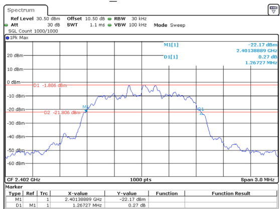
2DH1_Low 1.267MHz
