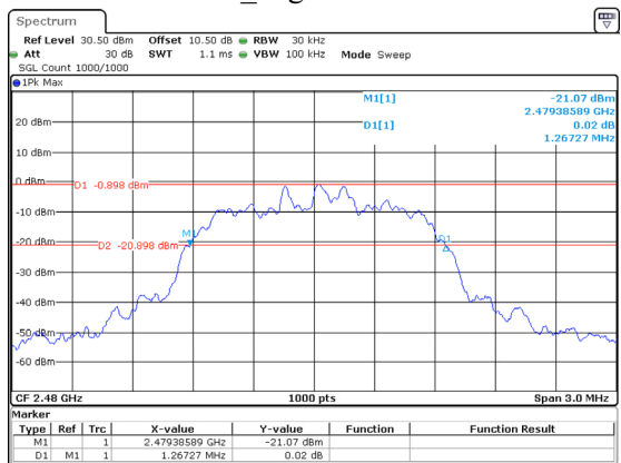
2DH1_High 1.267MHz
