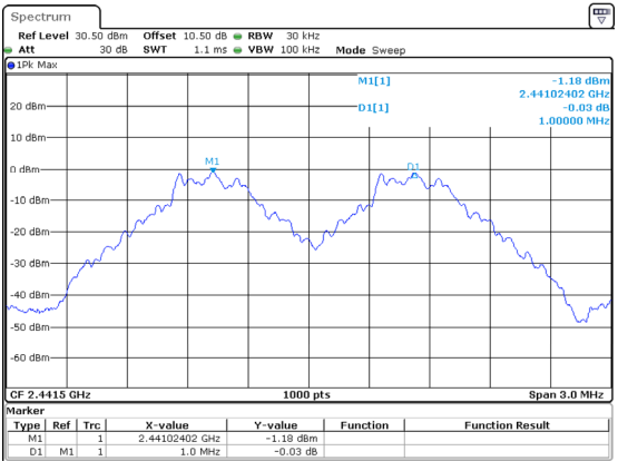
DH1_Middle 1MHz
