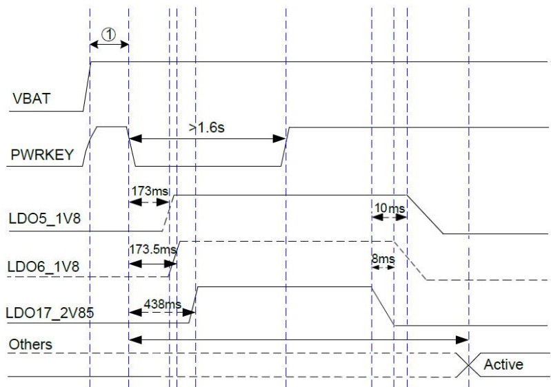
Figure 4.7: Using PWRKEY boot timing diagram
