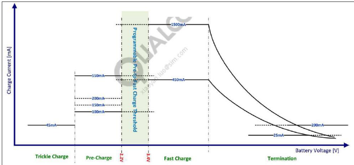
Figure 4.28: Charging diagram
