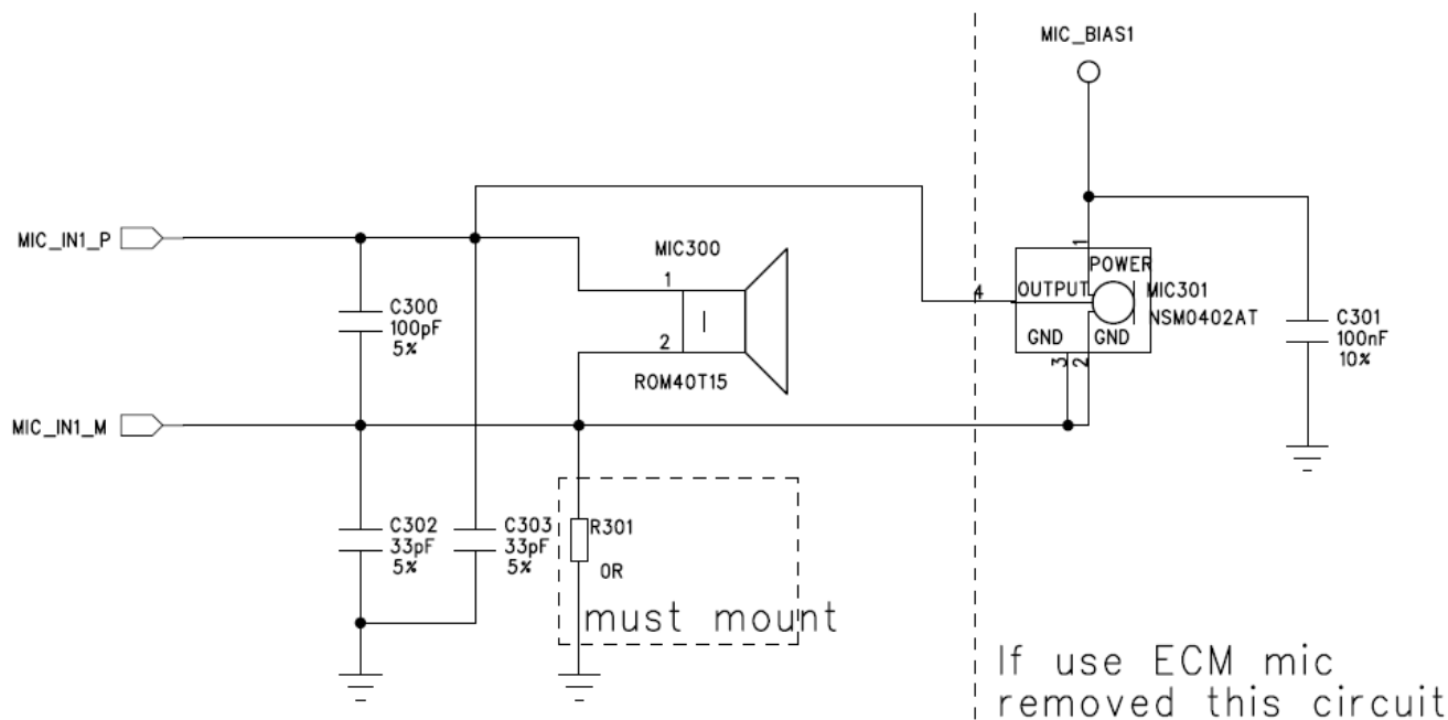
Figure 4.22: Microphone Differential Interface Circuit
