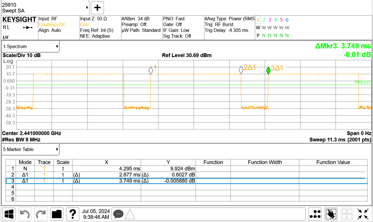
Duty Cycle plot (BT-BDR)
