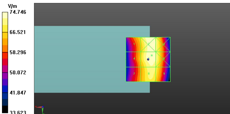
Fig A.1 HAC RF E-Field GSM850
