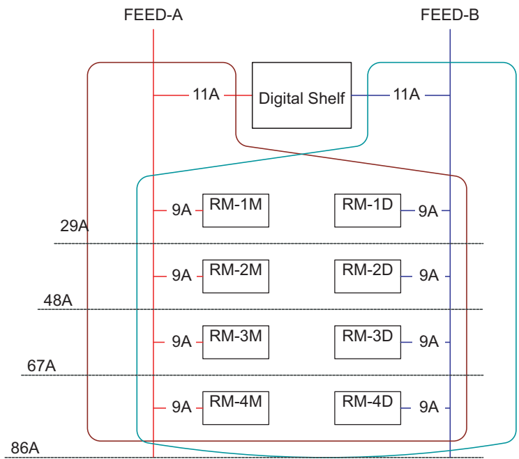
Figure 2.3 Power Consumption
