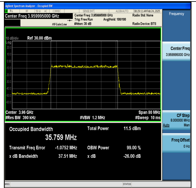
NTNV-n77(3700-3980)-PC2-30-40-H-DFT-BPSK-Outer_Full-Ant1-PASS
