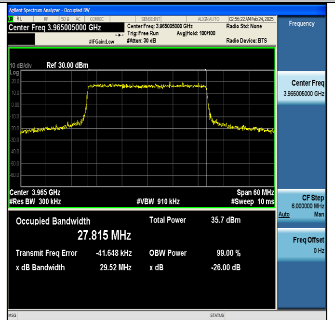
NTNV-n77(3700-3980)-PC2-30-30-H-CP-QPSK-Outer_Full-Ant1-PASS
