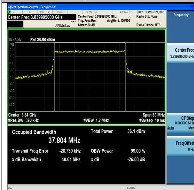
NTNV-n77(3700-3980)-PC2-30-40-M-CP-16QAM-Outer_Full-Ant1-PASS
