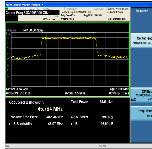
NTNV-n77(3700-3980)-PC2-30-50-M-CP-QPSK-Outer_Full-Ant1-PASS
