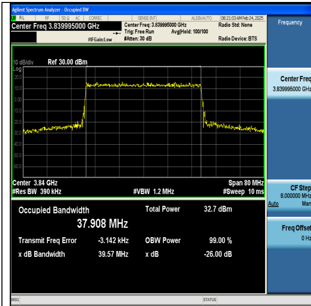
NTNV-n77(3700-3980)-PC2-30-40-M-CP-256QAM-Outer_Full-Ant1-PASS
