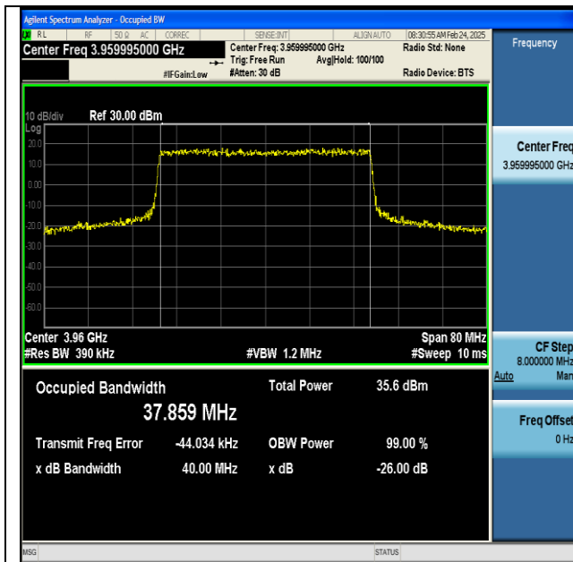
NTNV-n77(3700-3980)-PC2-30-40-H-CP-64QAM-Outer_Full-Ant1-PASS
