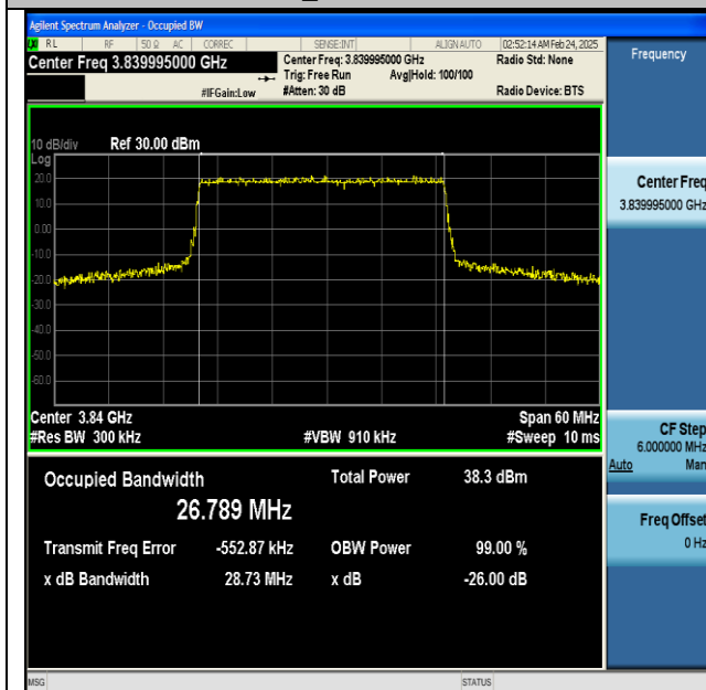
NTNV-n77(3700-3980)-PC2-30-30-M-DFT-QPSK-Outer_Full-Ant1-PASS
