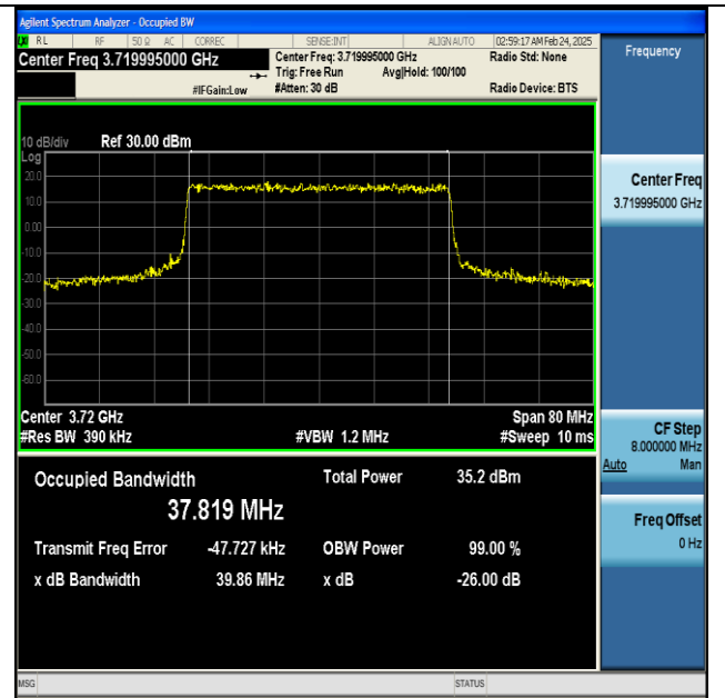
NTNV-n77(3700-3980)-PC2-30-40-L-CP-16QAM-Outer_Full-Ant1-PASS
