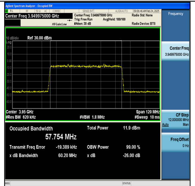
NTNV-n77(3700-3980)-PC2-30-60-H-DFT-BPSK-Outer_Full-Ant1-PASS
