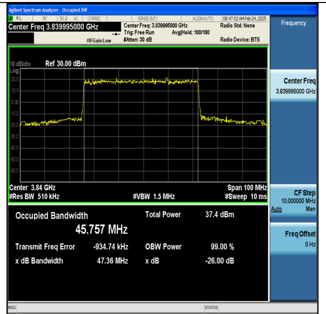
NTNV-n77(3700-3980)-PC2-30-50-M-DFT-16QAM-Outer_Full-Ant1-PASS
