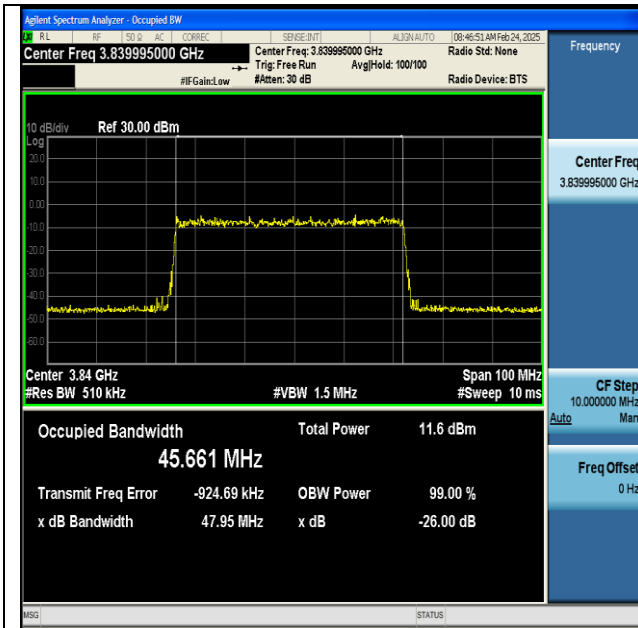
NTNV-n77(3700-3980)-PC2-30-50-M-DFT-QPSK-Outer_Full-Ant1-PASS
