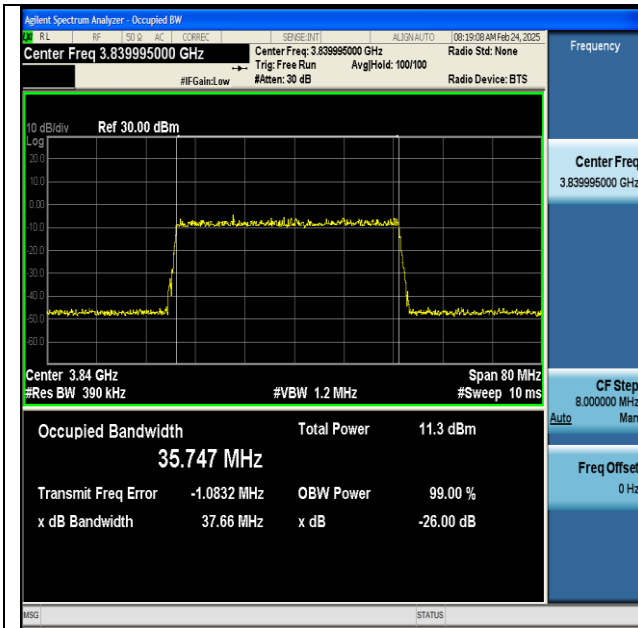
NTNV-n77(3700-3980)-PC2-30-40-M-DFT-BPSK-Outer_Full-Ant1-PASS
