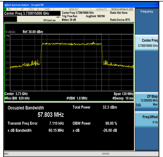
NTNV-n77(3700-3980)-PC2-30-60-L-CP-256QAM- Outer_Full-Ant1-PASS
