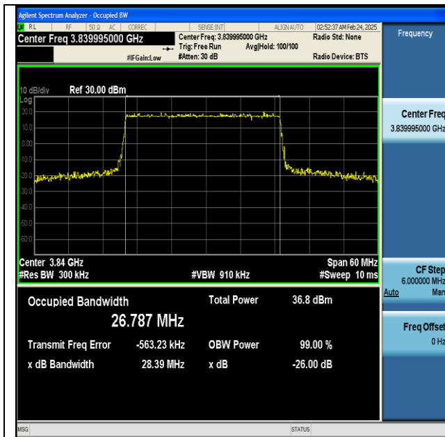
NTNV-n77(3700-3980)-PC2-30-30-M-DFT-64QAM-Outer_Full-Ant1-PASS
