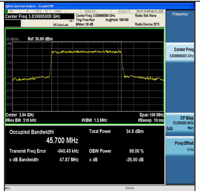
NTNV-n77(3700-3980)-PC2-30-50-M-DFT-256QAM-Outer_Full-Ant1-PASS
