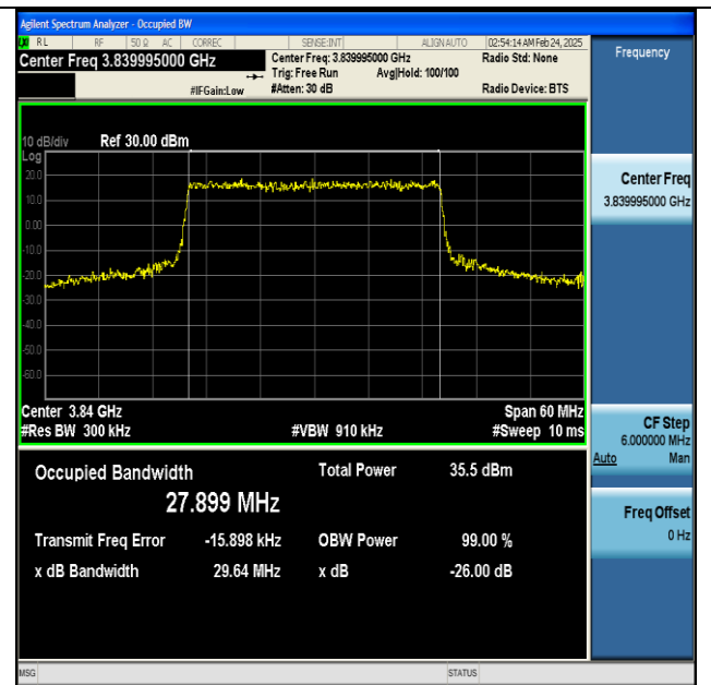
NTNV-n77(3700-3980)-PC2-30-30-M-CP-256QAM-Outer_Full-Ant1-PASS
