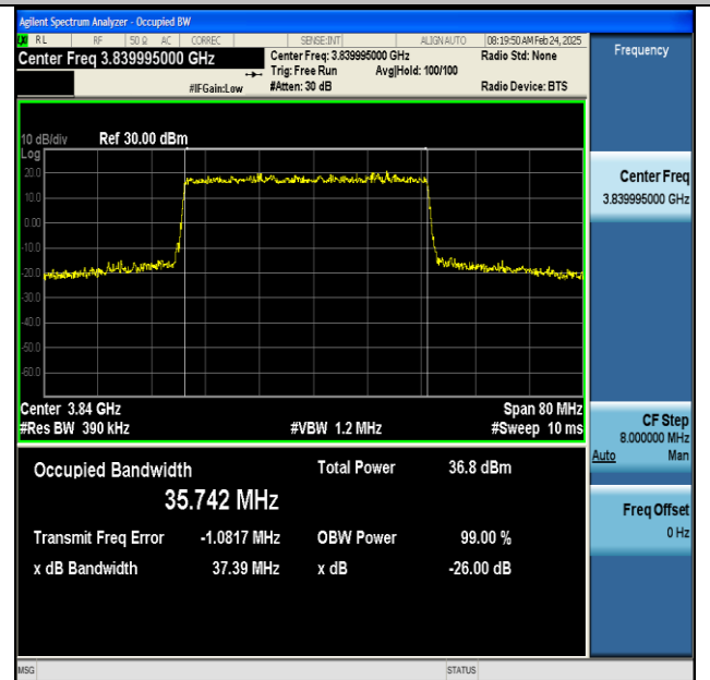
NTNV-n77(3700-3980)-PC2-30-40-M-DFT-64QAM-Outer_Full-Ant1-PASS
