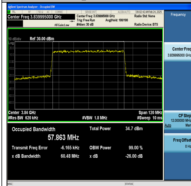
NTNV-n77(3700-3980)-PC2-30-60-M-DFT-256QAM-Outer_Full-Ant1-PASS
