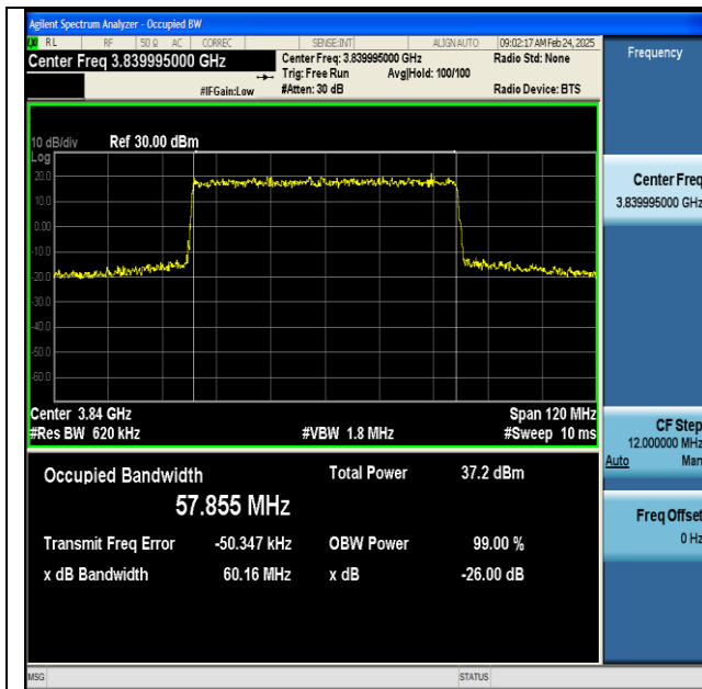
NTNV-n77(3700-3980)-PC2-30-60-M-DFT-16QAM-Outer_Full-Ant1-PASS
