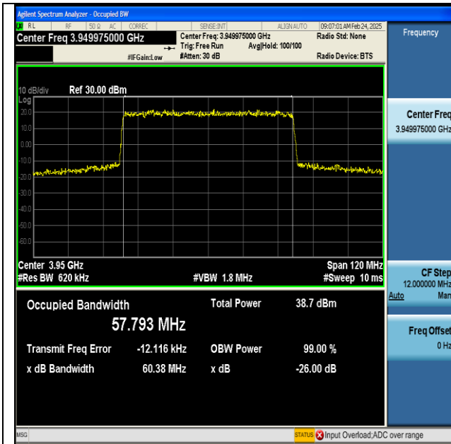
NTNV-n77(3700-3980)-PC2-30-60-H-DFT-QPSK- Outer_Full-Ant1-PASS
