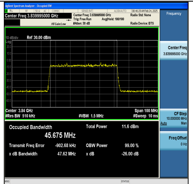
NTNV-n77(3700-3980)-PC2-30-50-M-DFT-BPSK-Outer_Full-Ant1-PASS
