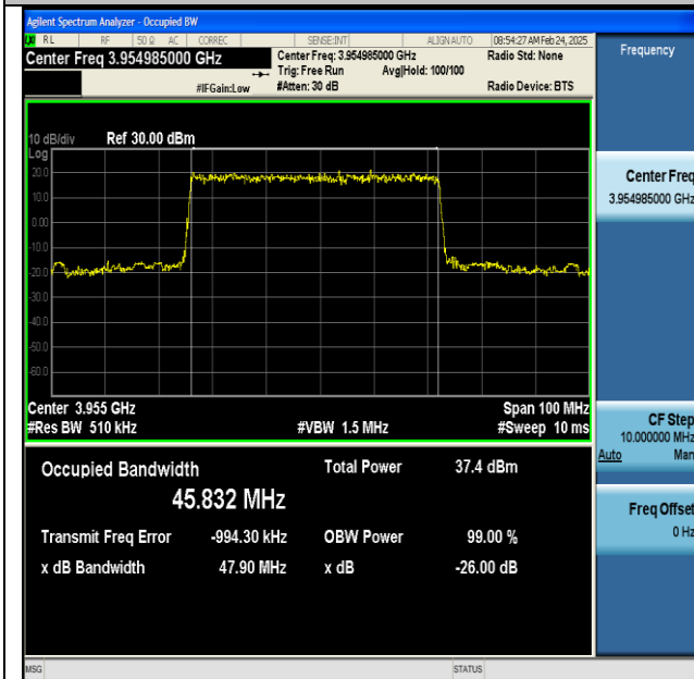
NTNV-n77(3700-3980)-PC2-30-50-H-DFT-16QAM-Outer_Full-Ant1-PASS
