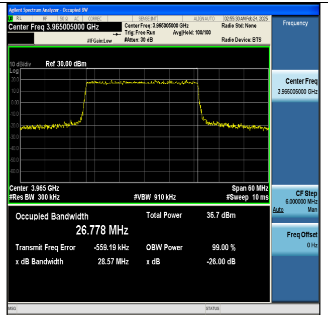
NTNV-n77(3700-3980)-PC2-30-30-H-DFT-64QAM-Outer_Full-Ant1-PASS
