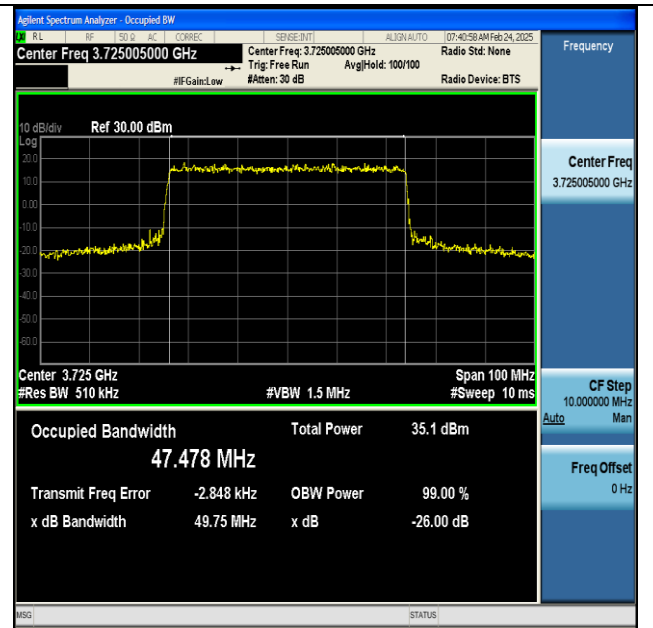
NTNV-n77(3700-3980)-PC2-30-50-L-CP-64QAM-Outer_Full-Ant1-PASS
