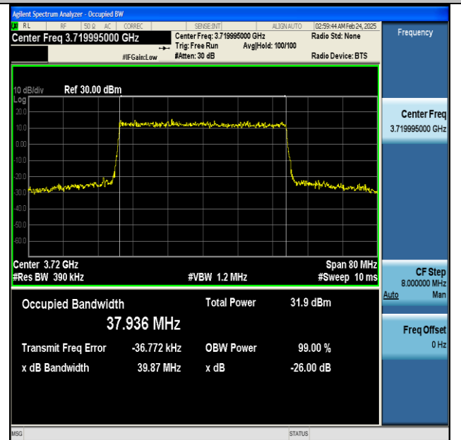
NTNV-n77(3700-3980)-PC2-30-40-L-CP-256QAM-Outer_Full-Ant1-PASS
