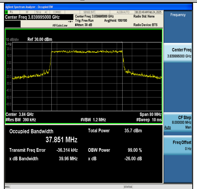
NTNV-n77(3700-3980)-PC2-30-40-M-CP-64QAM-Outer_Full-Ant1-PASS
