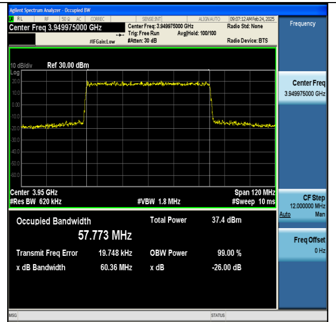
NTNV-n77(3700-3980)-PC2-30-60-H-DFT-16QAM- Outer_Full-Ant1-PASS
