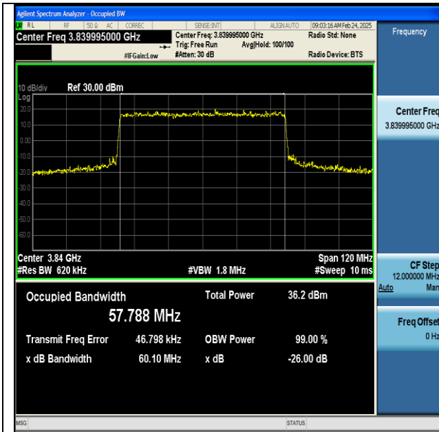
NTNV-n77(3700-3980)-PC2-30-60-M-CP-16QAM-Outer_Full-Ant1-PASS
