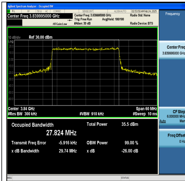
NTNV-n77(3700-3980)-PC2-30-30-M-CP-64QAM-Outer_Full-Ant1-PASS
