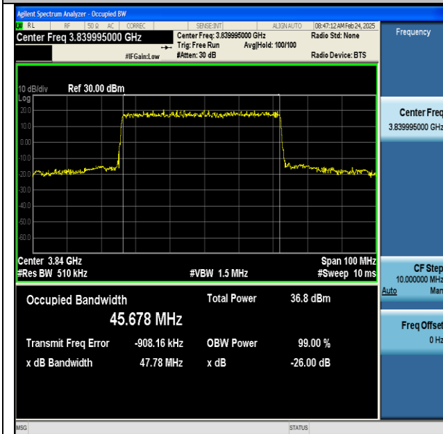
NTNV-n77(3700-3980)-PC2-30-50-M-DFT-64QAM-Outer_Full-Ant1-PASS
