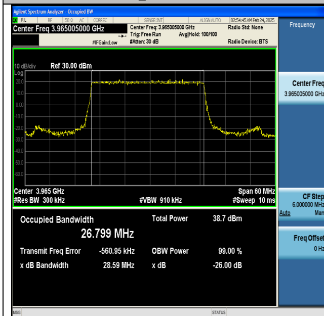
NTNV-n77(3700-3980)-PC2-30-30-H-DFT-BPSK-Outer_Full-Ant1-PASS
