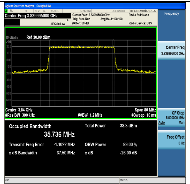
NTNV-n77(3700-3980)-PC2-30-40-M-DFT-QPSK-Outer_Full-Ant1-PASS
