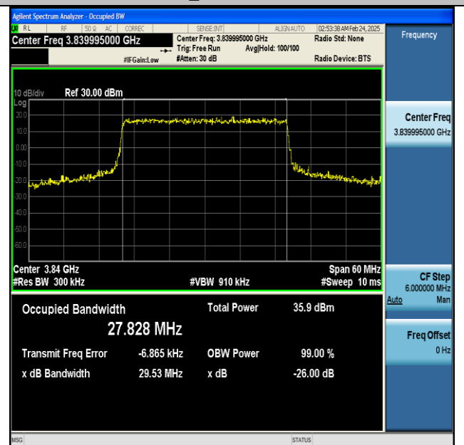
NTNV-n77(3700-3980)-PC2-30-30-M-CP-16QAM-Outer_Full-Ant1-PASS
