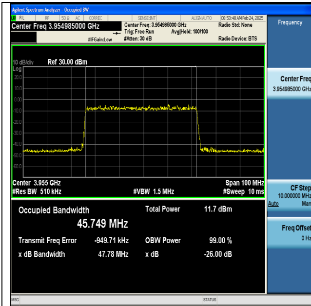
NTNV-n77(3700-3980)-PC2-30-50-H-DFT-BPSK-Outer_Full-Ant1-PASS
