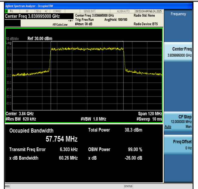
NTNV-n77(3700-3980)-PC2-30-60-M-DFT-QPSK- Outer_Full-Ant1-PASS
