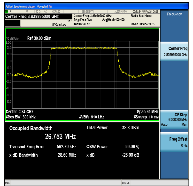
NTNV-n77(3700-3980)-PC2-30-30-M-DFT-BPSK-Outer_Full-Ant1-PASS
