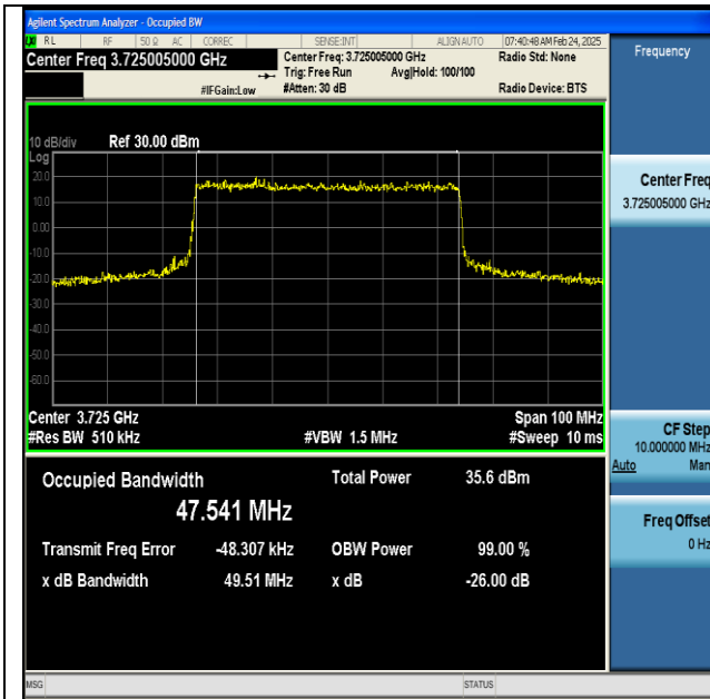
NTNV-n77(3700-3980)-PC2-30-50-L-CP-16QAM-Outer_Full-Ant1-PASS
