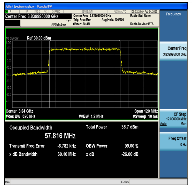
NTNV-n77(3700-3980)-PC2-30-60-M-DFT-64QAM-Outer_Full-Ant1-PASS
