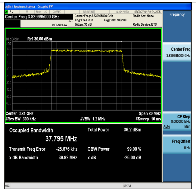
NTNV-n77(3700-3980)-PC2-30-40-M-CP-QPSK-Outer_Full-Ant1-PASS
