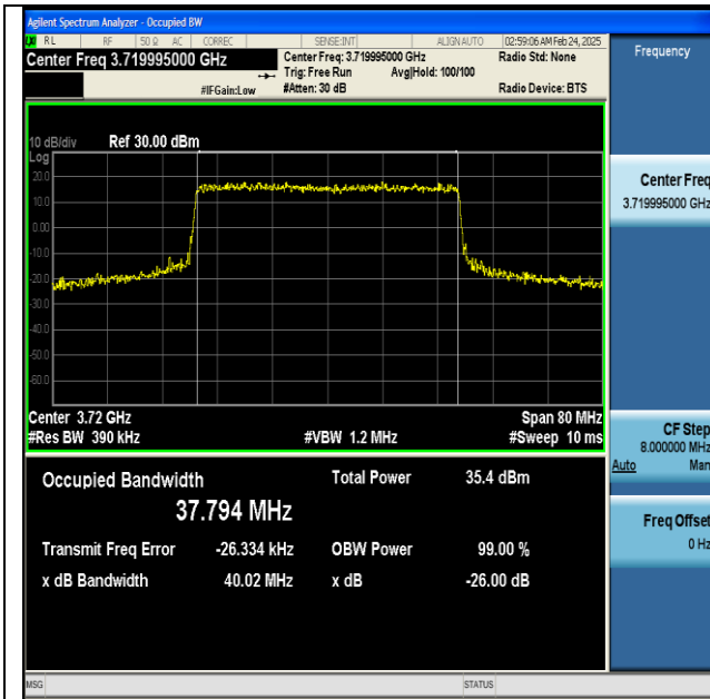
NTNV-n77(3700-3980)-PC2-30-40-L-CP-QPSK-Outer_Full-Ant1-PASS
