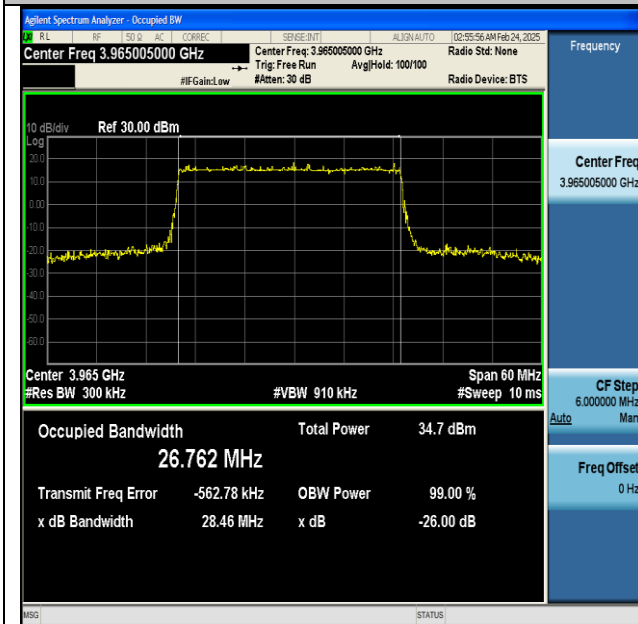
NTNV-n77(3700-3980)-PC2-30-30-H-DFT-256QAM-Outer_Full-Ant1-PASS
