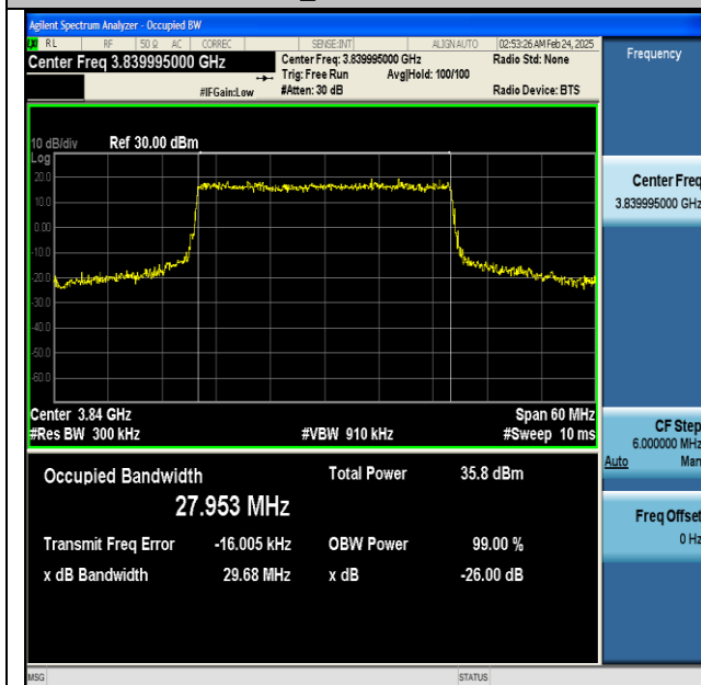
NTNV-n77(3700-3980)-PC2-30-30-M-CP-QPSK-Outer_Full-Ant1-PASS
