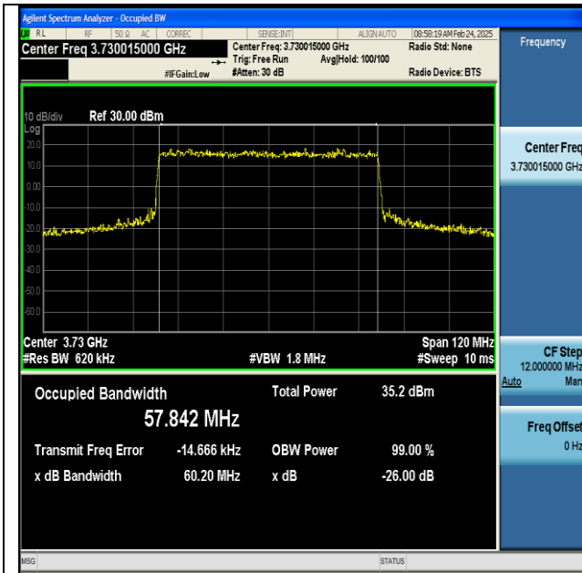
NTNV-n77(3700-3980)-PC2-30-60-L-CP-64QAM- Outer_Full-Ant1-PASS
