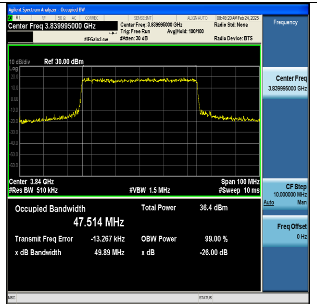
NTNV-n77(3700-3980)-PC2-30-50-M-CP-16QAM-Outer_Full-Ant1-PASS
