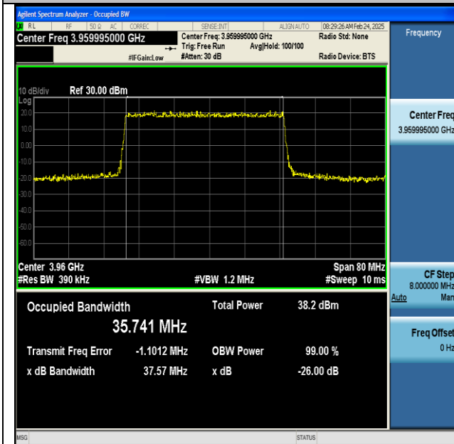
NTNV-n77(3700-3980)-PC2-30-40-H-DFT-QPSK-Outer_Full-Ant1-PASS
