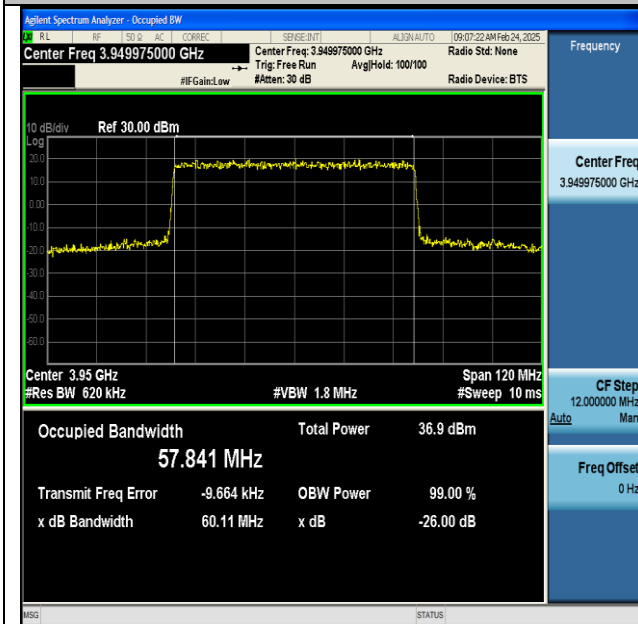
NTNV-n77(3700-3980)-PC2-30-60-H-DFT-64QAM- Outer_Full-Ant1-PASS
