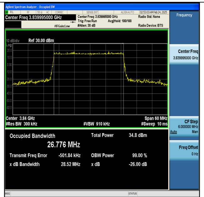
NTNV-n77(3700-3980)-PC2-30-30-M-DFT-256QAM-Outer_Full-Ant1-PASS
