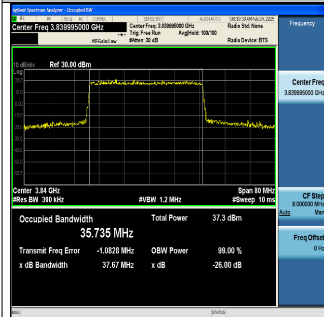
NTNV-n77(3700-3980)-PC2-30-40-M-DFT-16QAM-Outer_Full-Ant1-PASS
