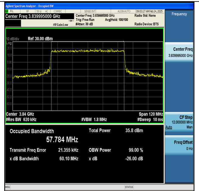
NTNV-n77(3700-3980)-PC2-30-60-M-CP-64QAM-Outer_Full-Ant1-PASS
