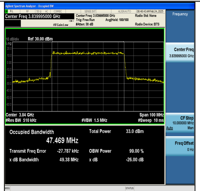
NTNV-n77(3700-3980)-PC2-30-50-M-CP-256QAM-Outer_Full-Ant1-PASS
