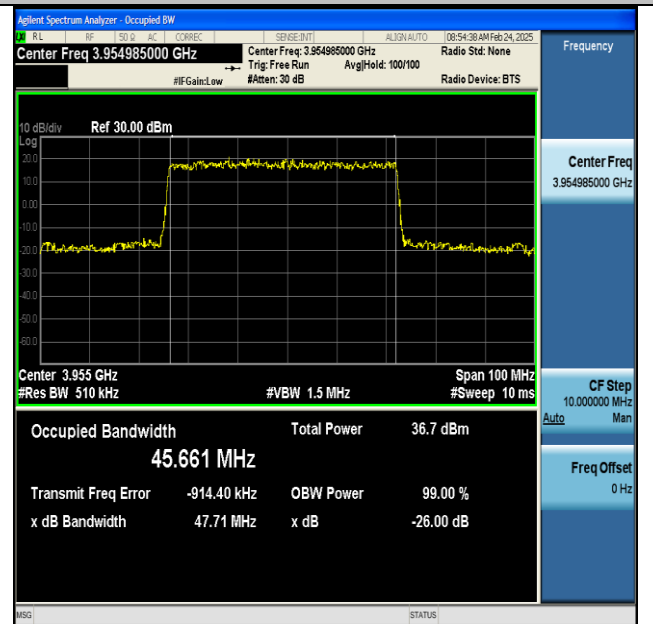
NTNV-n77(3700-3980)-PC2-30-50-H-DFT-64QAM-Outer_Full-Ant1-PASS
