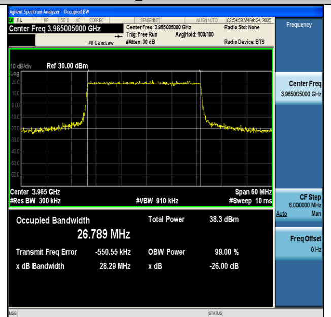
NTNV-n77(3700-3980)-PC2-30-30-H-DFT-QPSK-Outer_Full-Ant1-PASS
