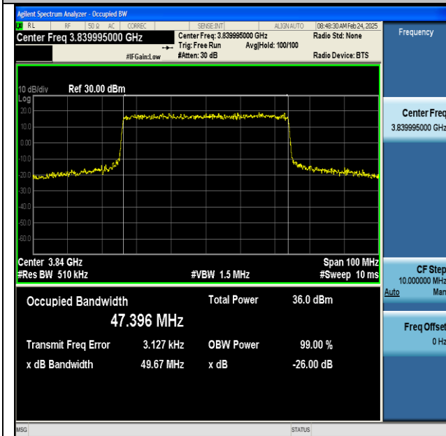
NTNV-n77(3700-3980)-PC2-30-50-M-CP-64QAM-Outer_Full-Ant1-PASS
