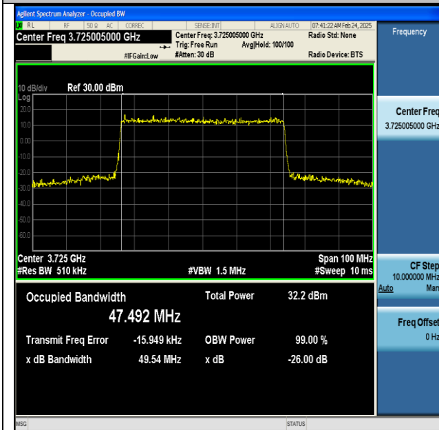
NTNV-n77(3700-3980)-PC2-30-50-L-CP-256QAM-Outer_Full-Ant1-PASS
