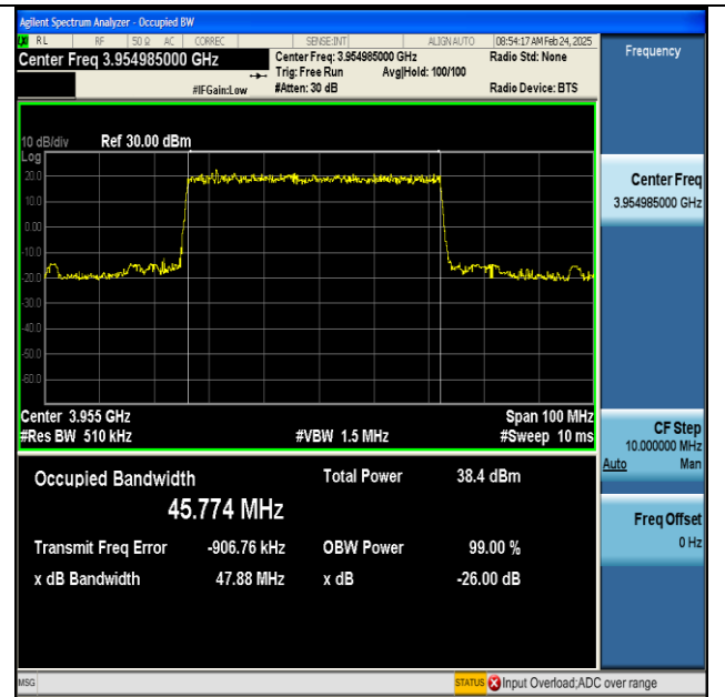
NTNV-n77(3700-3980)-PC2-30-50-H-DFT-QPSK-Outer_Full-Ant1-PASS
