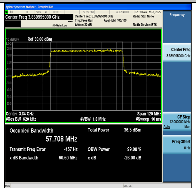
NTNV-n77(3700-3980)-PC2-30-60-M-CP-QPSK-Outer_Full-Ant1-PASS
