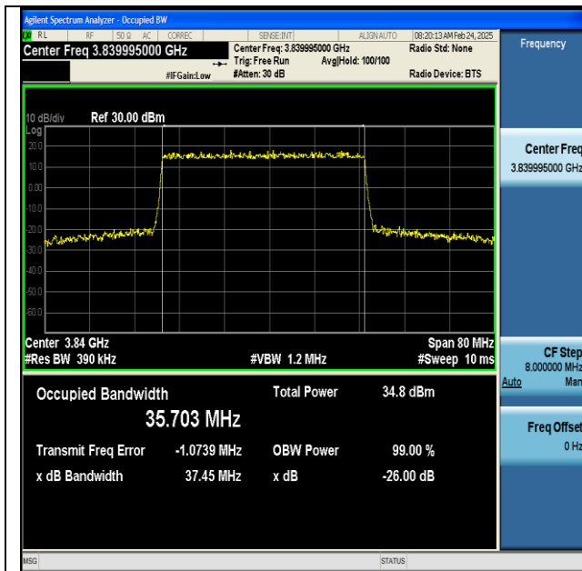
NTNV-n77(3700-3980)-PC2-30-40-M-DFT-256QAM-Outer_Full-Ant1-PASS
