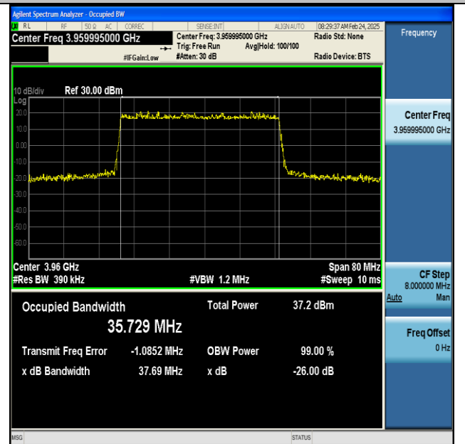
NTNV-n77(3700-3980)-PC2-30-40-H-DFT-16QAM-Outer_Full-Ant1-PASS
