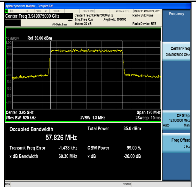
NTNV-n77(3700-3980)-PC2-30-60-H-DFT-256QAM- Outer_Full-Ant1-PASS
