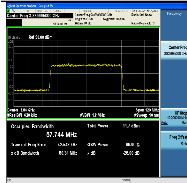
NTNV-n77(3700-3980)-PC2-30-60-M-DFT-BPSK- Outer_Full-Ant1-PASS
