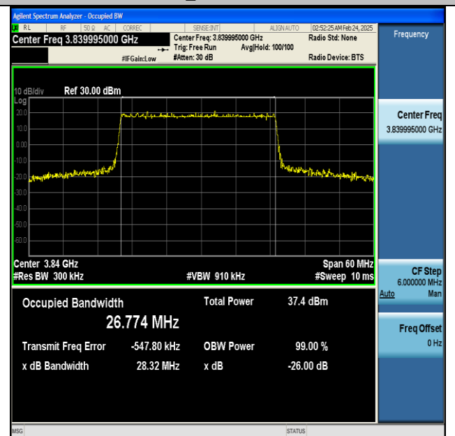
NTNV-n77(3700-3980)-PC2-30-30-M-DFT-16QAM-Outer_Full-Ant1-PASS
