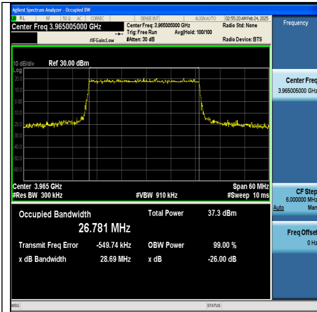
NTNV-n77(3700-3980)-PC2-30-30-H-DFT-16QAM-Outer_Full-Ant1-PASS
