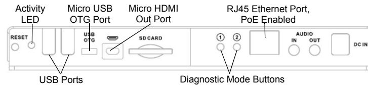
Figure 3. Ports
