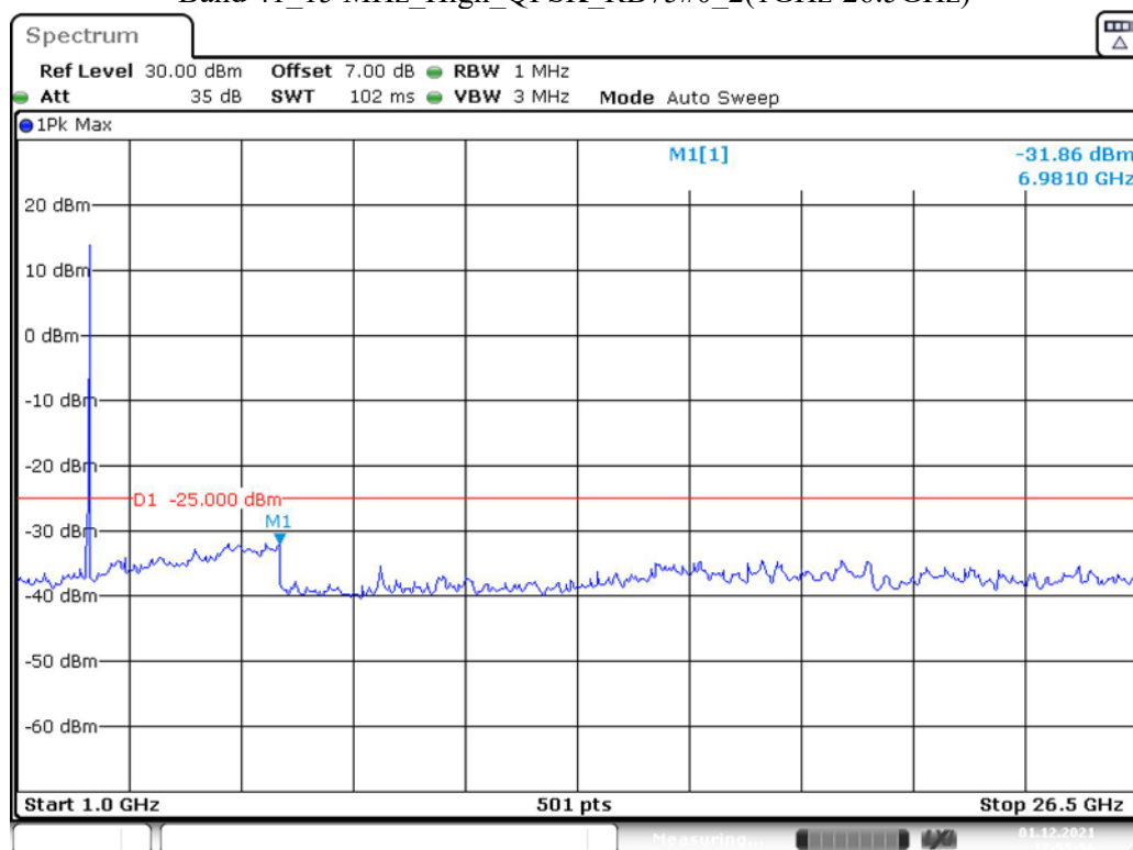
Band 41_15 MHz_High_QPSK_RB75#0_2(1GHz-26.5GHz)
