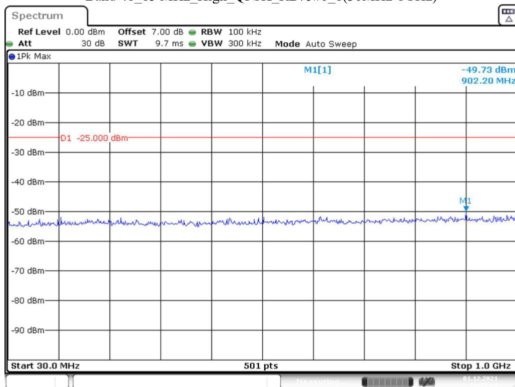
Band 41_15 MHz_High_QPSK_RB75#0_1(30MHz-1GHz)
