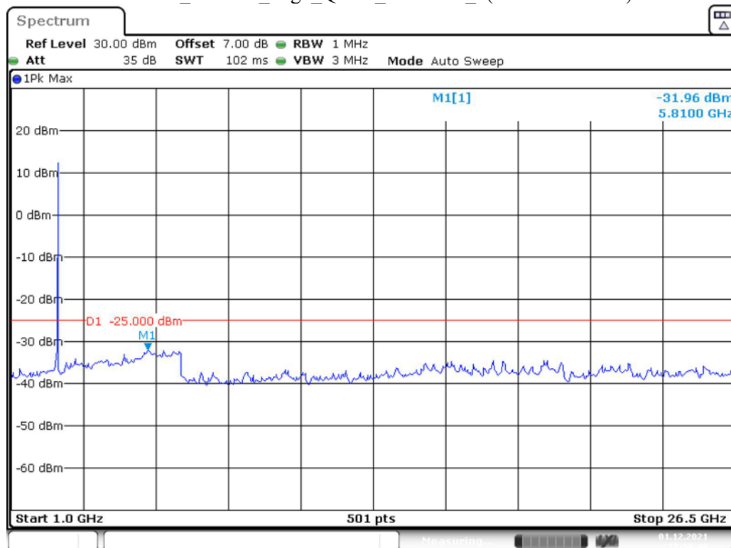
Band 41_20 MHz_High_QPSK_RB100#0_2(1GHz-26.5GHz)
