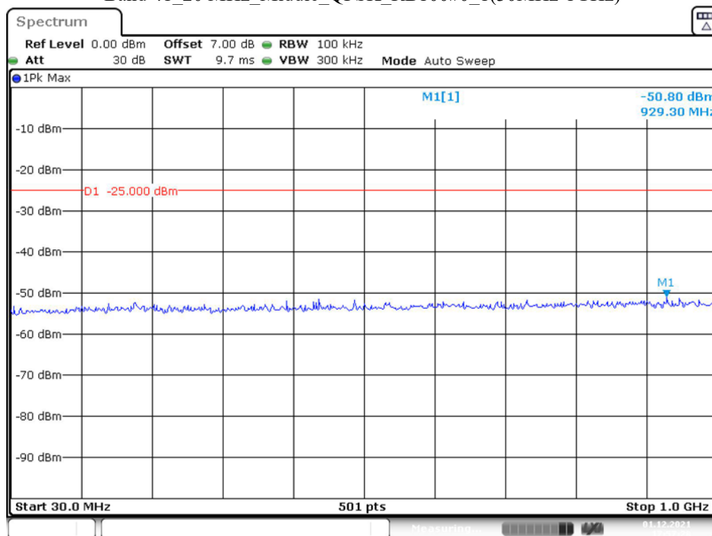
Band 41_20 MHz_Middle_QPSK_RB100#0_1(30MHz-1GHz)
