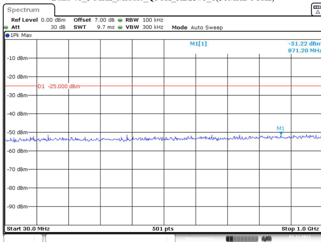
Band 41_5 MHz_Middle_QPSK_RB25#0_1(30MHz-1GHz)
