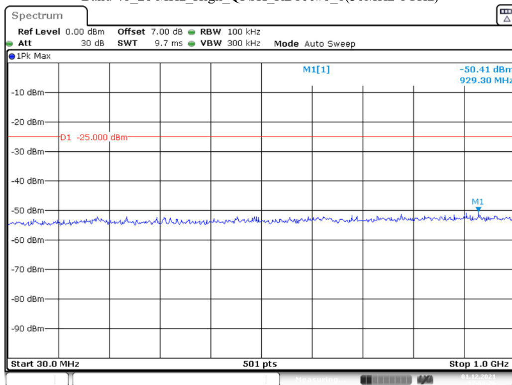
Band 41_20 MHz_High_QPSK_RB100#0_1(30MHz-1GHz)
