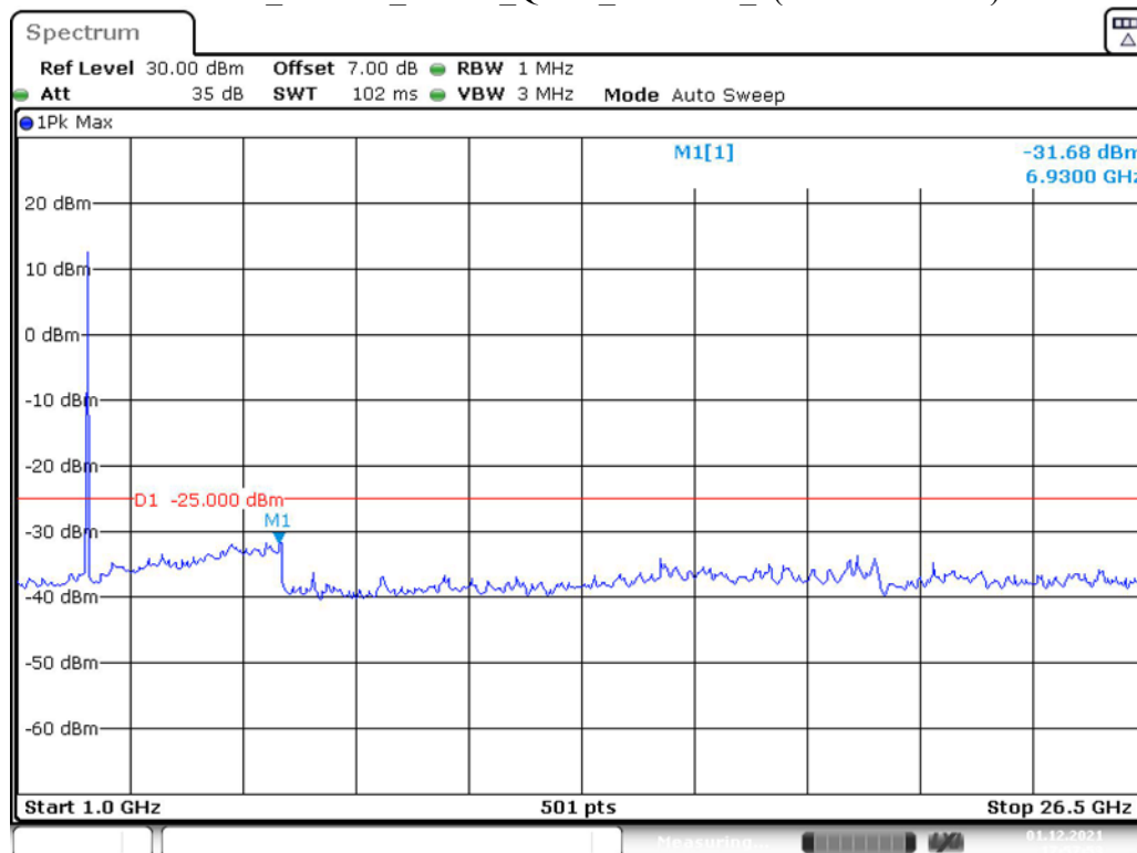
Band 41_20 MHz_Middle_QPSK_RB100#0_2(1GHz-26.5GHz)
