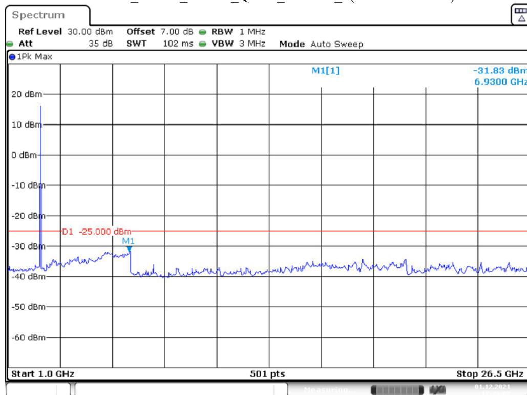
Band 41_5 MHz_Middle_QPSK_RB25#0_2(1GHz-26.5GHz)
