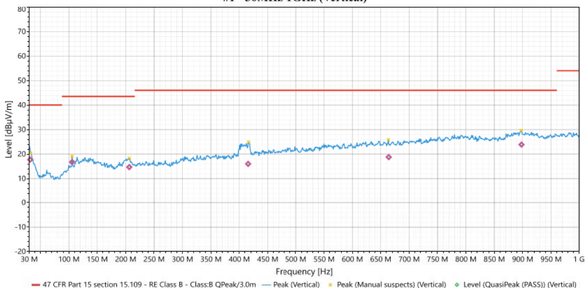
#1 - 30MHz-1GHz (Vertical)
