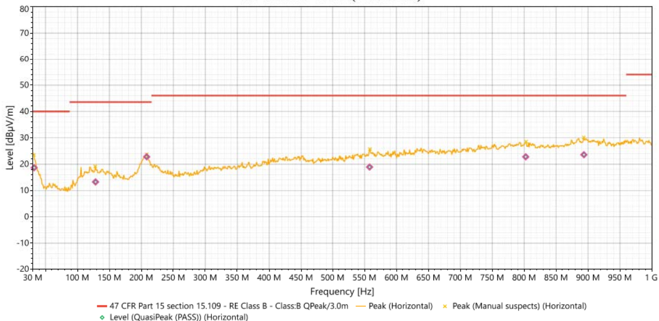
#2 - 30MHz-1GHz (Horizontal)
