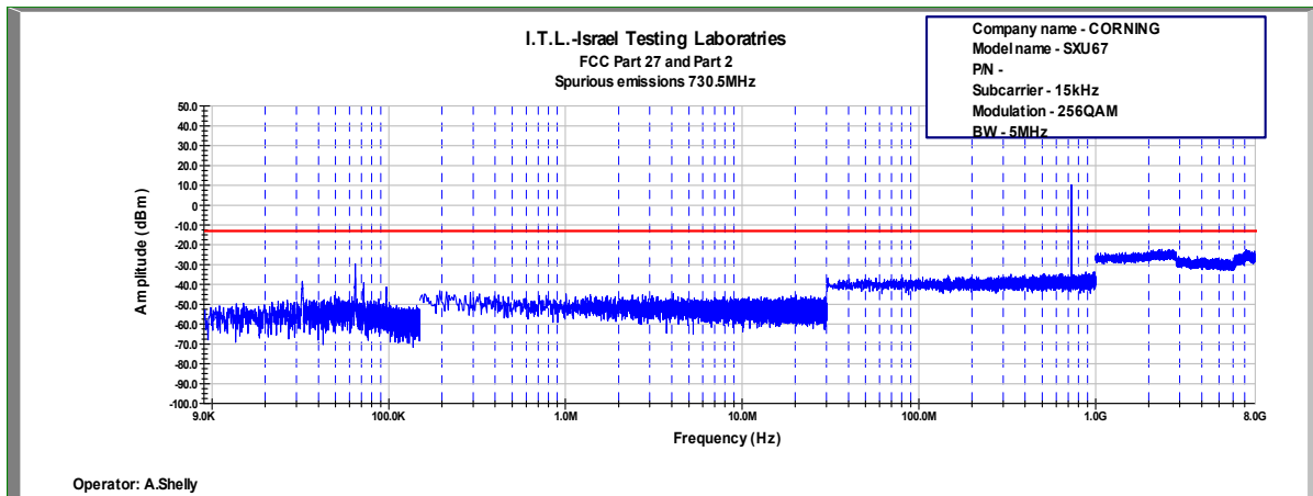
Figure 687: Spurious Emissions at Antenna Terminal 256QAM, 730.5MHz, B.W. 5MHz, Sub Carrier 15kHz
