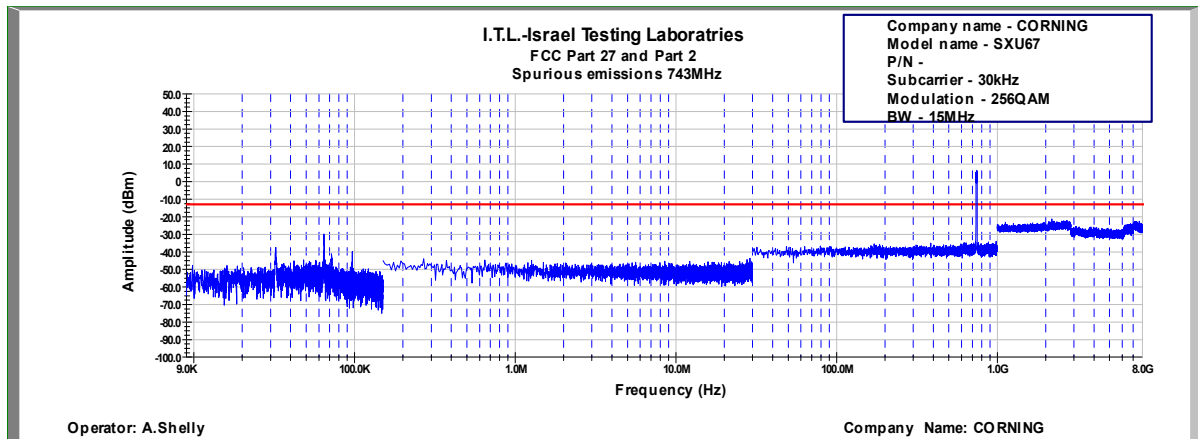
Figure 706: Spurious Emissions at Antenna Terminal 256QAM, 743.0MHz, B.W. 15MHz, Sub Carrier 30kHz
