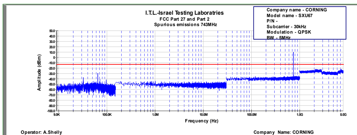
Figure 724: Spurious Emissions at Antenna Terminal QPSK, 743.0MHz, B.W. 5MHz, Sub Carrier 30kHz
