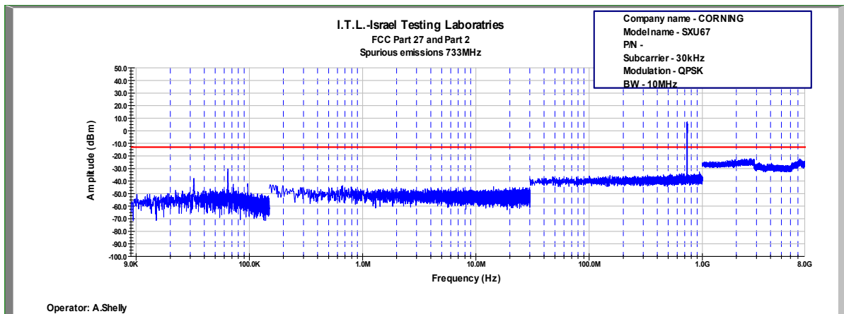
Figure 729: Spurious Emissions at Antenna Terminal QPSK, 733.0MHz, B.W. 10MHz, Sub Carrier 30kHz
