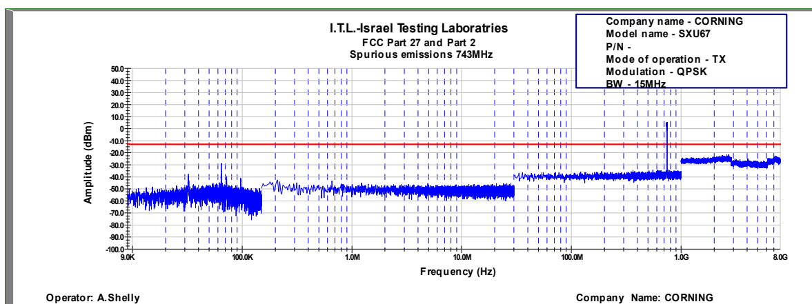
Figure 739: Spurious Emissions at Antenna Terminal QPSK, 743.0MHz, B.W. 15MHz, Sub Carrier 30kHz
