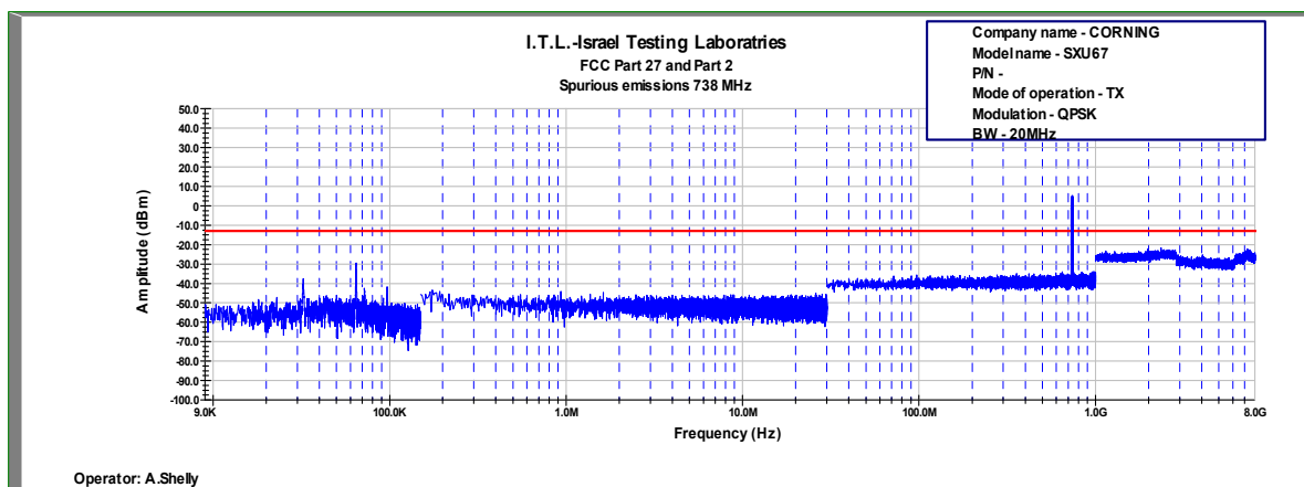
Figure 744: Spurious Emissions at Antenna Terminal QPSK, 738.0MHz, B.W. 20MHz, Sub Carrier 15kHz
