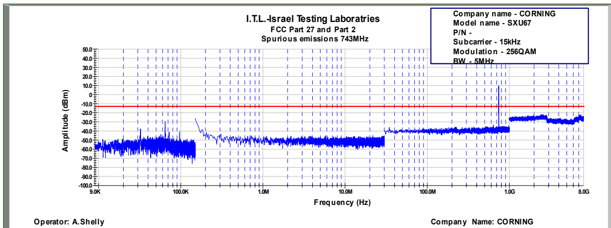
Figure 688: Spurious Emissions at Antenna Terminal 256QAM, 743.0MHz, B.W. 5MHz, Sub Carrier 15kHz
