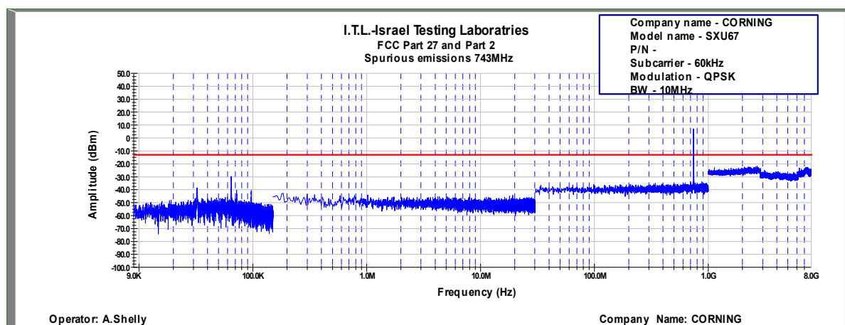
Figure 733: Spurious Emissions at Antenna Terminal QPSK, 743.0MHz, B.W. 10MHz, Sub Carrier 60kHz
