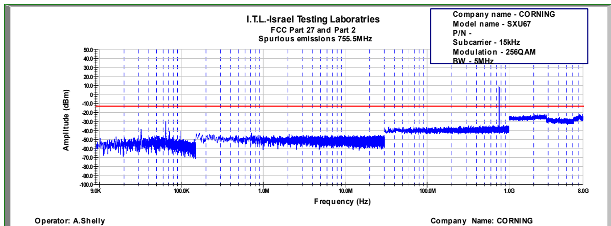
Figure 689: Spurious Emissions at Antenna Terminal 256QAM, 755.5MHz, B.W. 5MHz, Sub Carrier 15kHz
