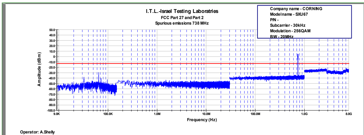
Figure 714: Spurious Emissions at Antenna Terminal 256QAM, 738.0MHz, B.W. 20MHz, Sub Carrier 30kHz
