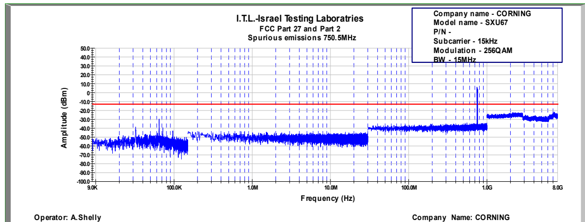
Figure 704: Spurious Emissions at Antenna Terminal 256QAM, 750.5MHz, B.W. 15MHz, Sub Carrier 15kHz
