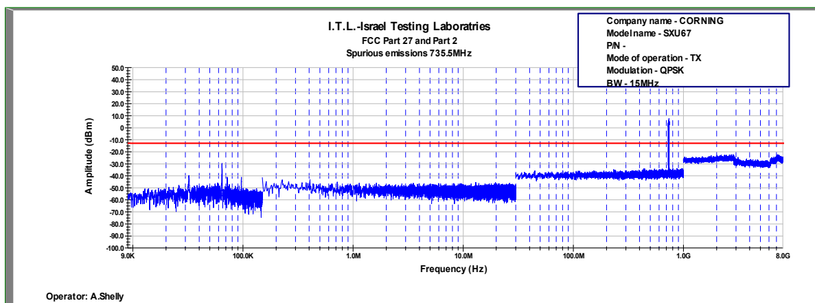
Figure 735: Spurious Emissions at Antenna Terminal QPSK, 735.5MHz, B.W. 15MHz, Sub Carrier 15kHz
