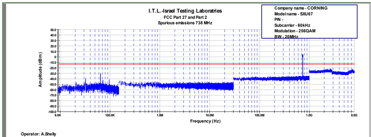
Figure 717: Spurious Emissions at Antenna Terminal 256QAM, 738.0MHz, B.W. 20MHz, Sub Carrier 60kHz
