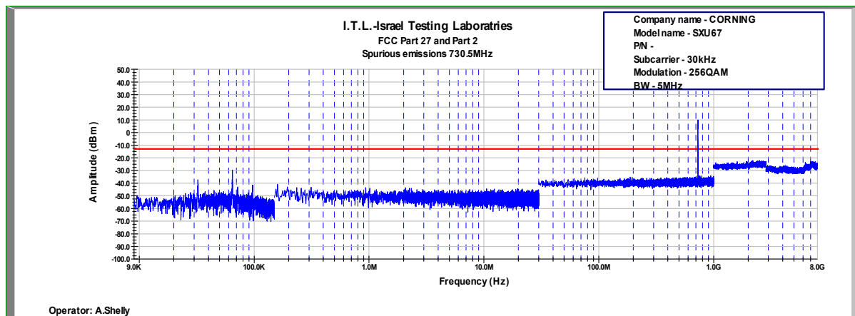
Figure 690: Spurious Emissions at Antenna Terminal 256QAM, 730.5MHz, B.W. 5MHz, Sub Carrier 30kHz
