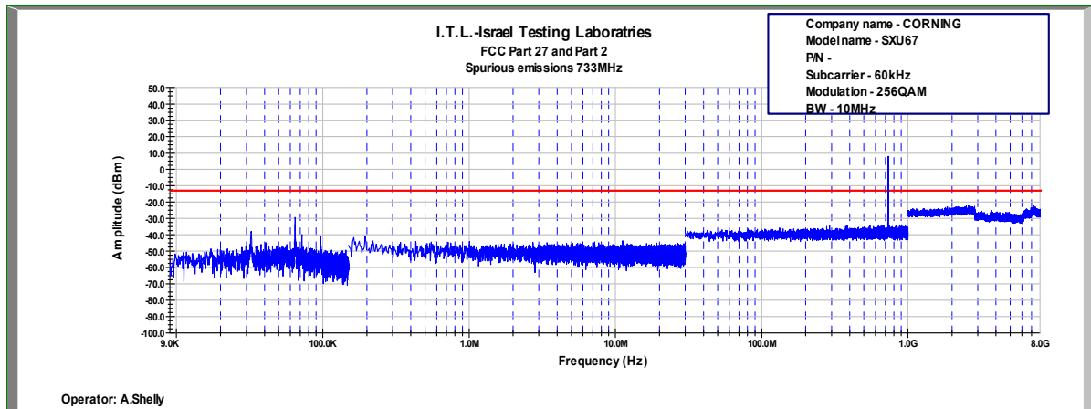
Figure 699: Spurious Emissions at Antenna Terminal 256QAM, 733.0MHz, B.W. 10MHz, Sub Carrier 60kHz
