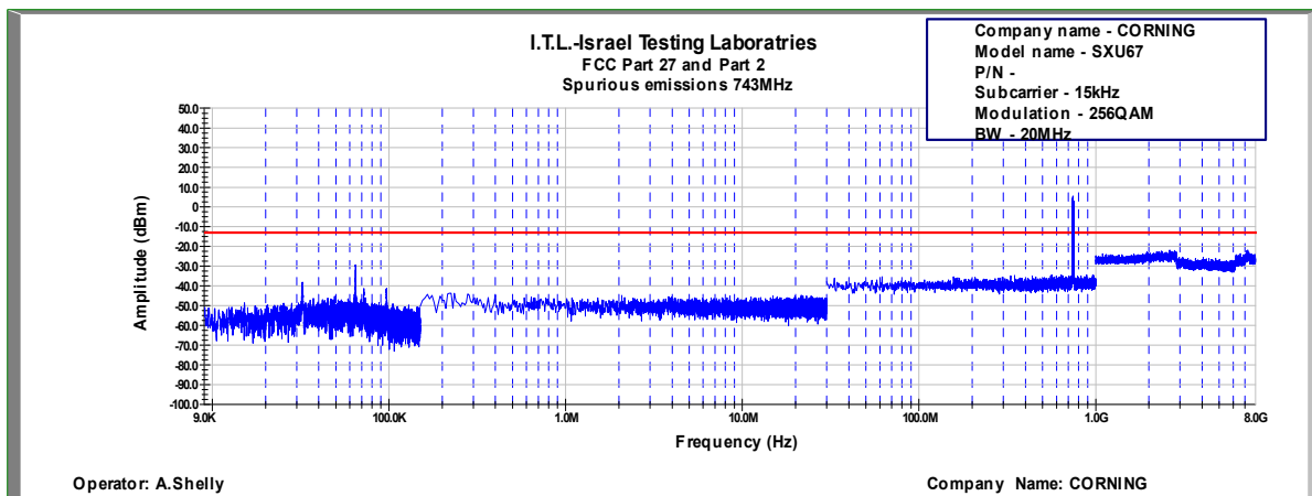
Figure 712: Spurious Emissions at Antenna Terminal 256QAM, 743.0MHz, B.W. 20MHz, Sub Carrier 15kHz
