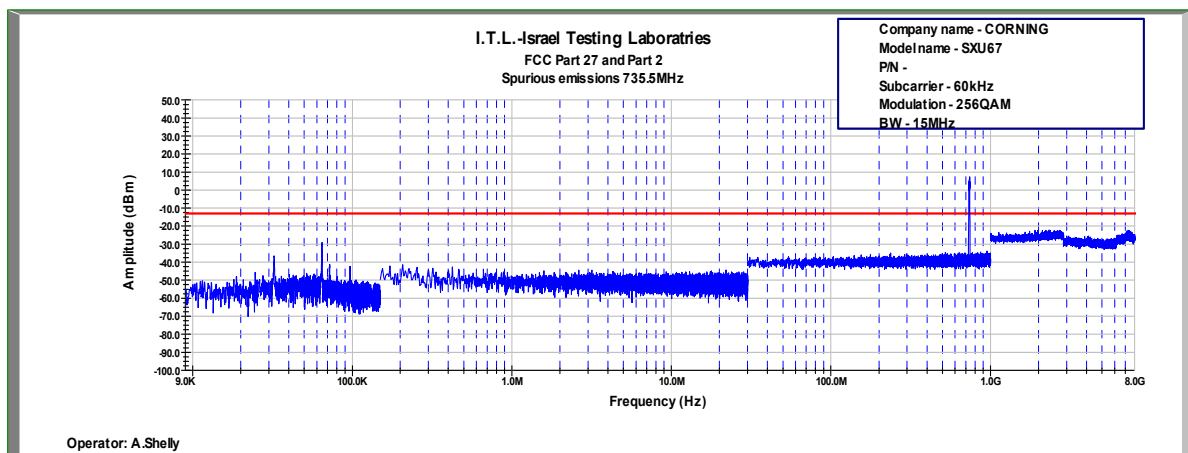
Figure 708: Spurious Emissions at Antenna Terminal 256QAM, 735.5MHz, B.W. 15MHz, Sub Carrier 60kHz
