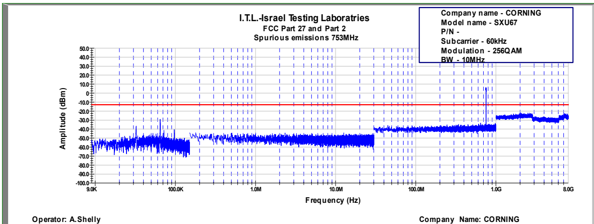
Figure 701: Spurious Emissions at Antenna Terminal 256QAM, 753.0MHz, B.W. 10MHz, Sub Carrier 60kHz
