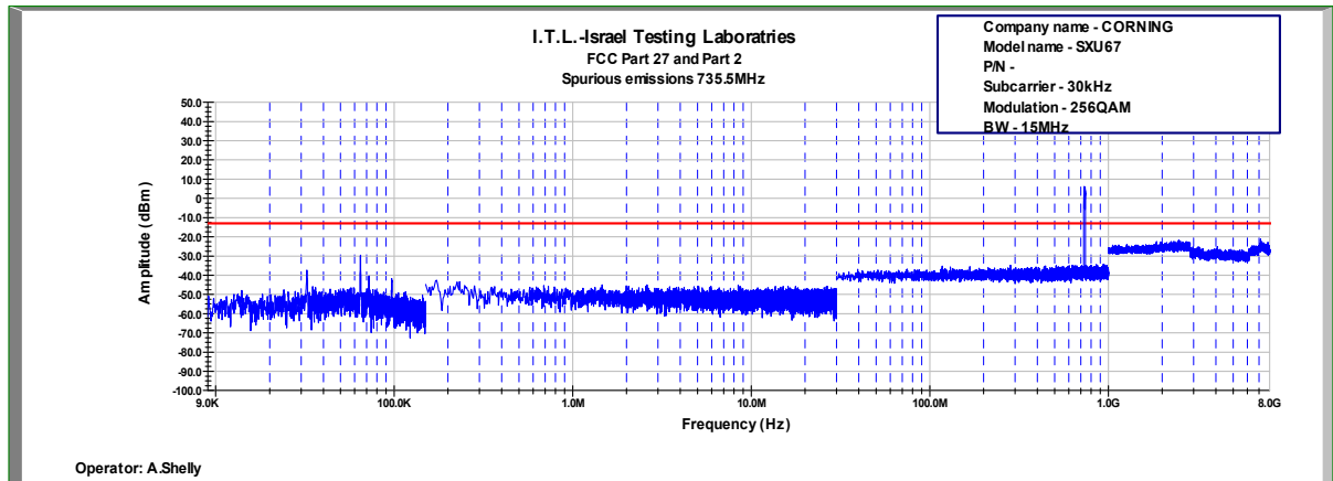
Figure 705: Spurious Emissions at Antenna Terminal 256QAM, 735.5MHz, B.W. 15MHz, Sub Carrier 30kHz
