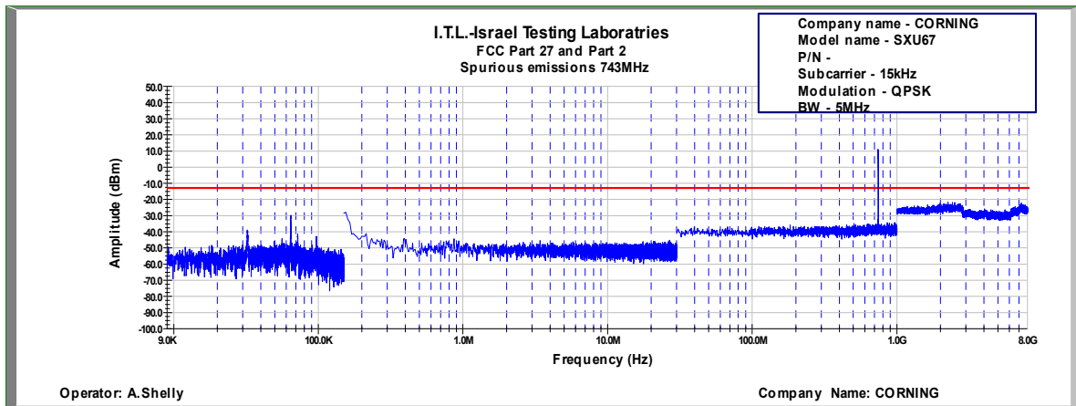
Figure 721: Spurious Emissions at Antenna Terminal QPSK, 743.0MHz, B.W. 5MHz, Sub Carrier 15kHz
