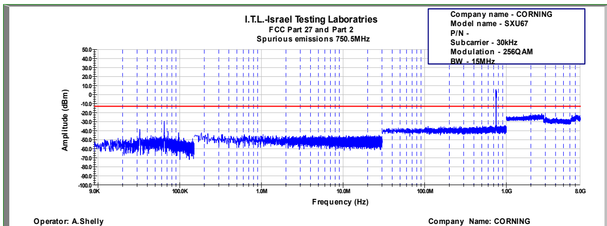
Figure 707: Spurious Emissions at Antenna Terminal 256QAM, 750.5MHz, B.W. 15MHz, Sub Carrier 30kHz
