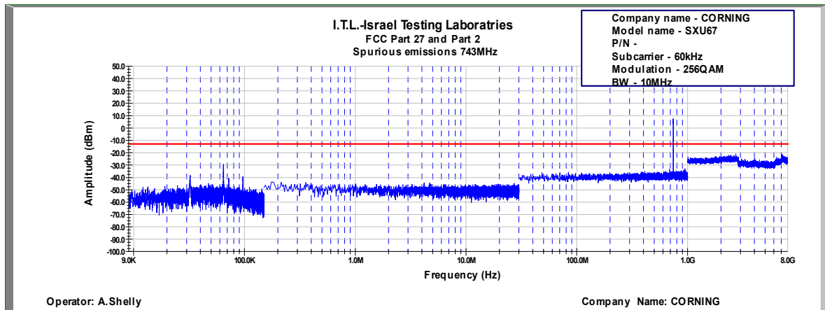
Figure 700: Spurious Emissions at Antenna Terminal 256QAM, 743.0MHz, B.W. 10MHz, Sub Carrier 60kHz
