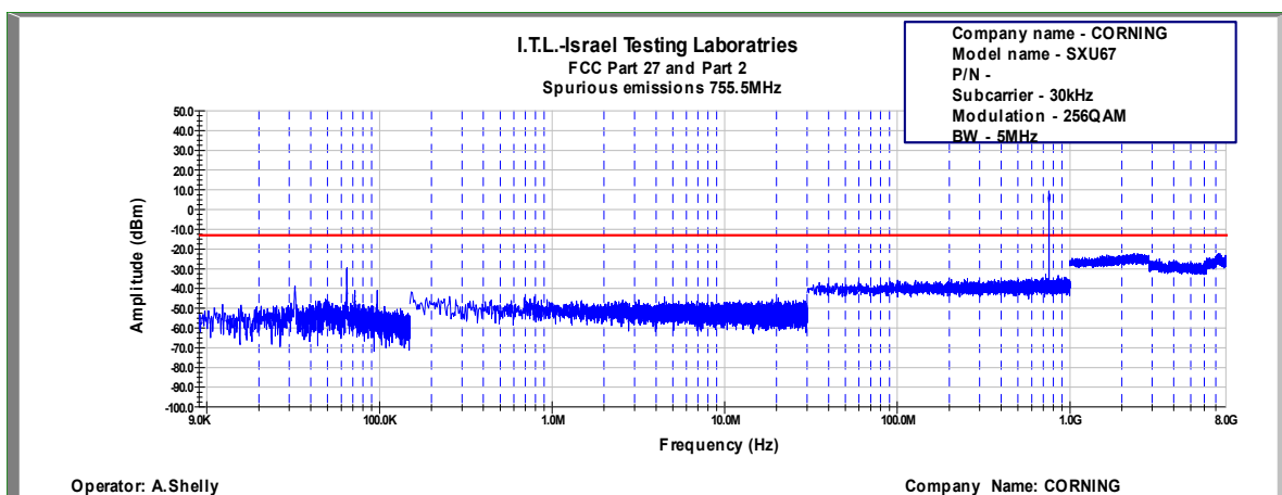
Figure 692: Spurious Emissions at Antenna Terminal 256QAM, 755.5MHz, B.W. 5MHz, Sub Carrier 30kHz
