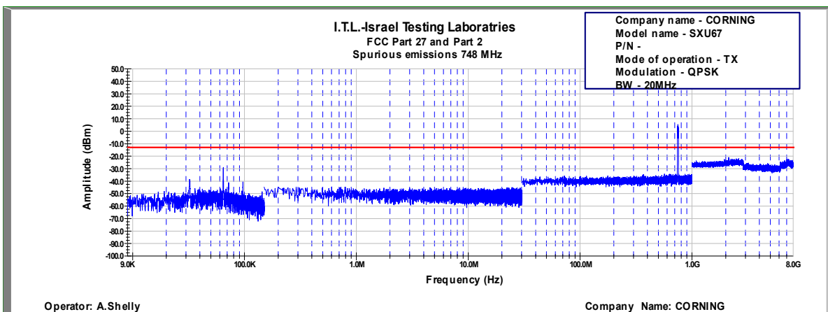
Figure 749: Spurious Emissions at Antenna Terminal QPSK, 748.0MHz, B.W. 20MHz, Sub Carrier 30kHz
