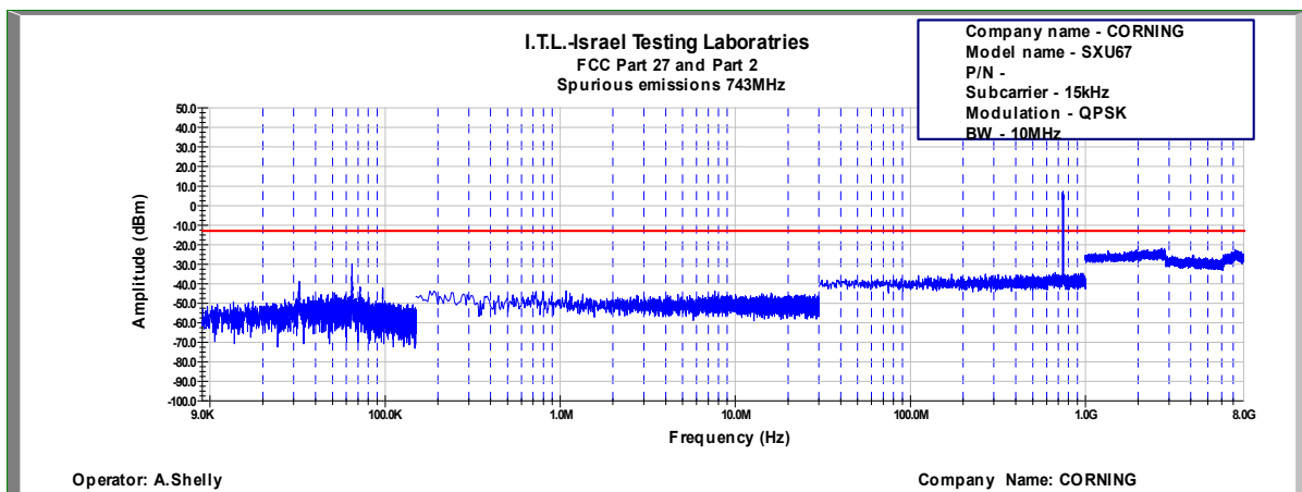
Figure 727: Spurious Emissions at Antenna Terminal QPSK, 743.0MHz, B.W. 10MHz, Sub Carrier 15kHz
