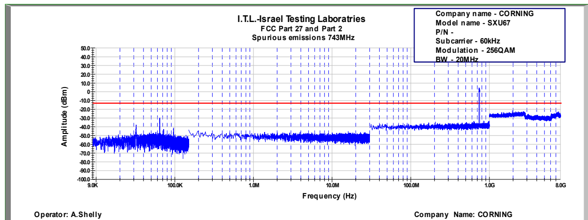
Figure 718: Spurious Emissions at Antenna Terminal 256QAM, 743.0MHz, B.W. 20MHz, Sub Carrier 60kHz
