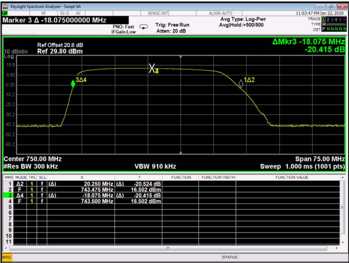
Figure 753. — Out-of-Band Rejection Plot
