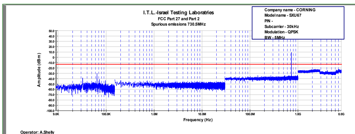
Figure 723: Spurious Emissions at Antenna Terminal QPSK, 730.5MHz, B.W. 5MHz, Sub Carrier 30kHz
