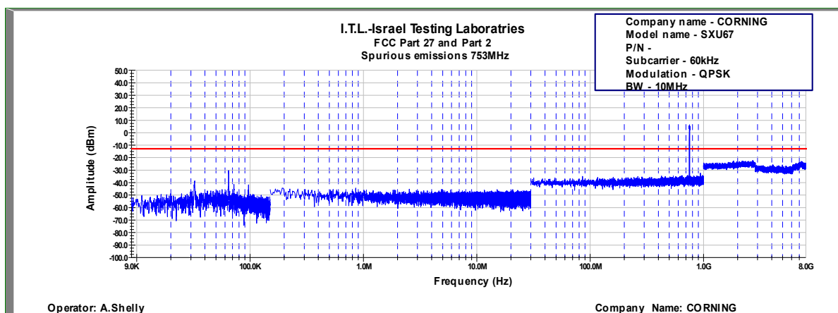
Figure 734: Spurious Emissions at Antenna Terminal QPSK, 753.0MHz, B.W. 10MHz, Sub Carrier 60kHz
