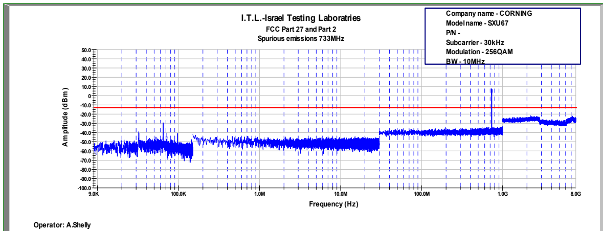
Figure 696: Spurious Emissions at Antenna Terminal 256QAM, 733.0MHz, B.W. 10MHz, Sub Carrier 30kHz
