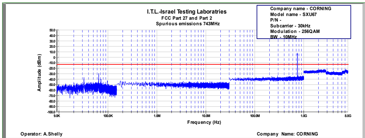
Figure 697: Spurious Emissions at Antenna Terminal 256QAM, 743.0MHz, B.W. 10MHz, Sub Carrier 30kHz
