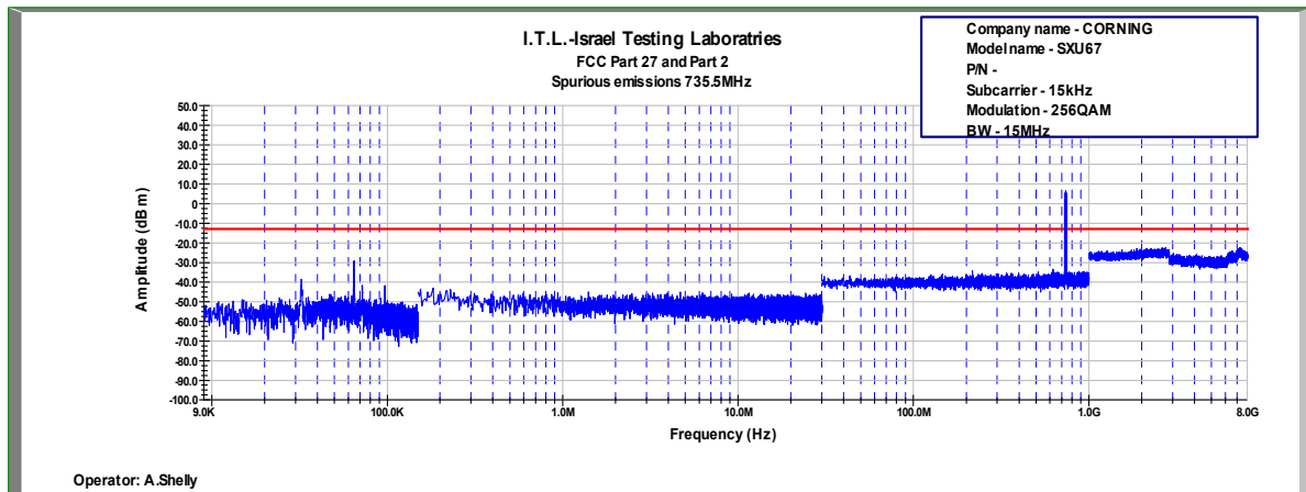
Figure 702: Spurious Emissions at Antenna Terminal 256QAM, 735.5MHz, B.W. 15MHz, Sub Carrier 15kHz
