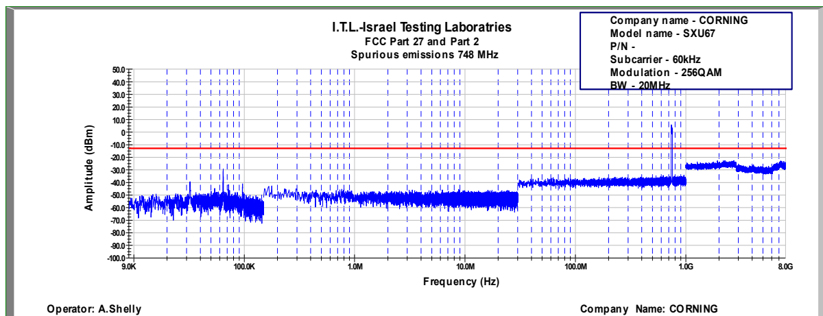
Figure 719: Spurious Emissions at Antenna Terminal 256QAM, 748.0MHz, B.W. 20MHz, Sub Carrier 60kHz
