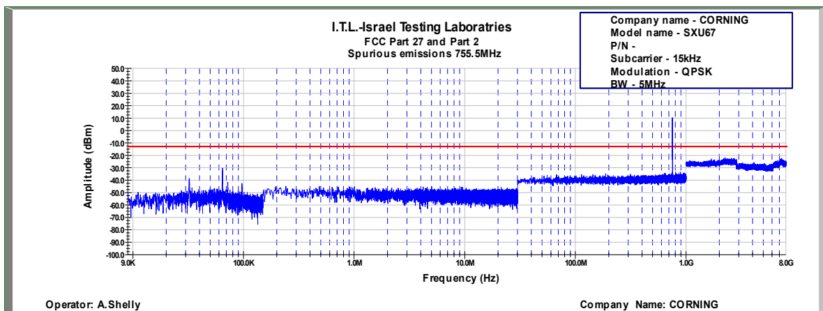
Figure 722: Spurious Emissions at Antenna Terminal QPSK, 755.5MHz, B.W. 5MHz, Sub Carrier 15kHz
