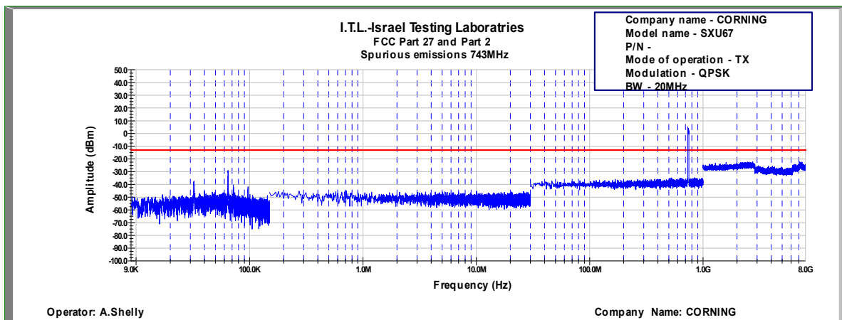
Figure 751: Spurious Emissions at Antenna Terminal QPSK, 743.0MHz, B.W. 20MHz, Sub Carrier 60kHz
