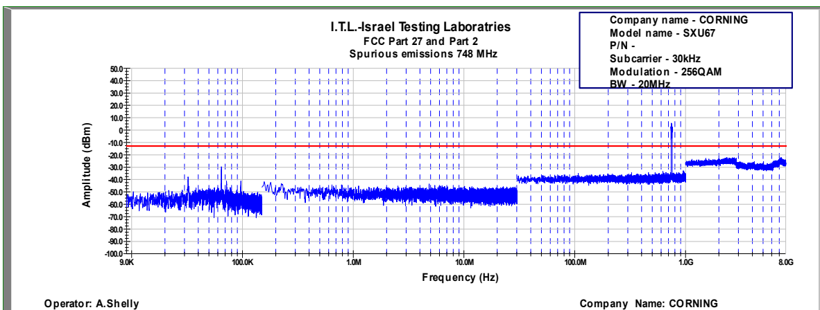
Figure 716: Spurious Emissions at Antenna Terminal 256QAM, 748.0MHz, B.W. 20MHz, Sub Carrier 30kHz
