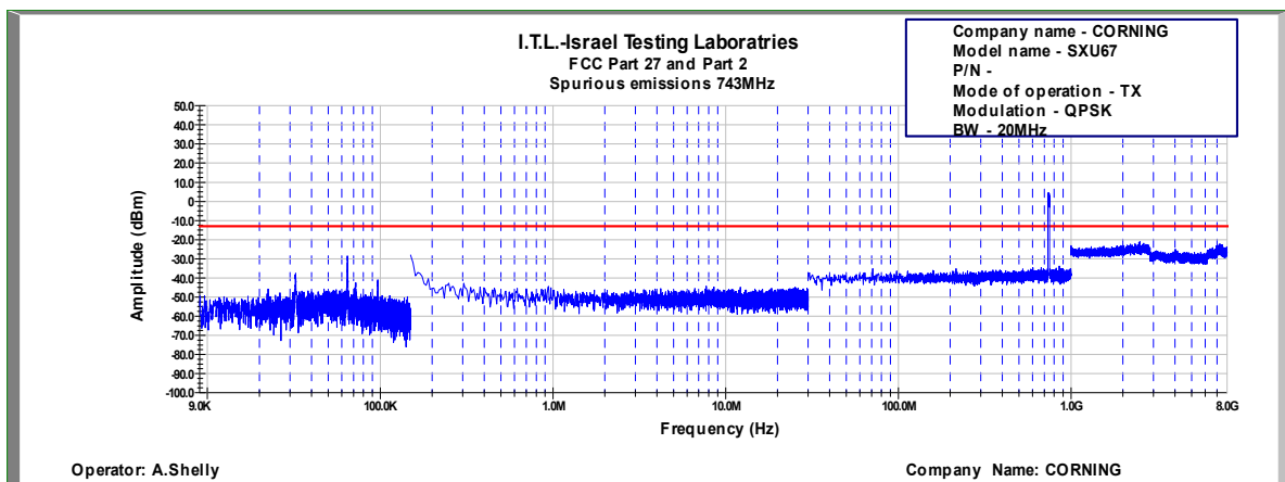
Figure 748: Spurious Emissions at Antenna Terminal QPSK, 743.0MHz, B.W. 20MHz, Sub Carrier 30kHz
