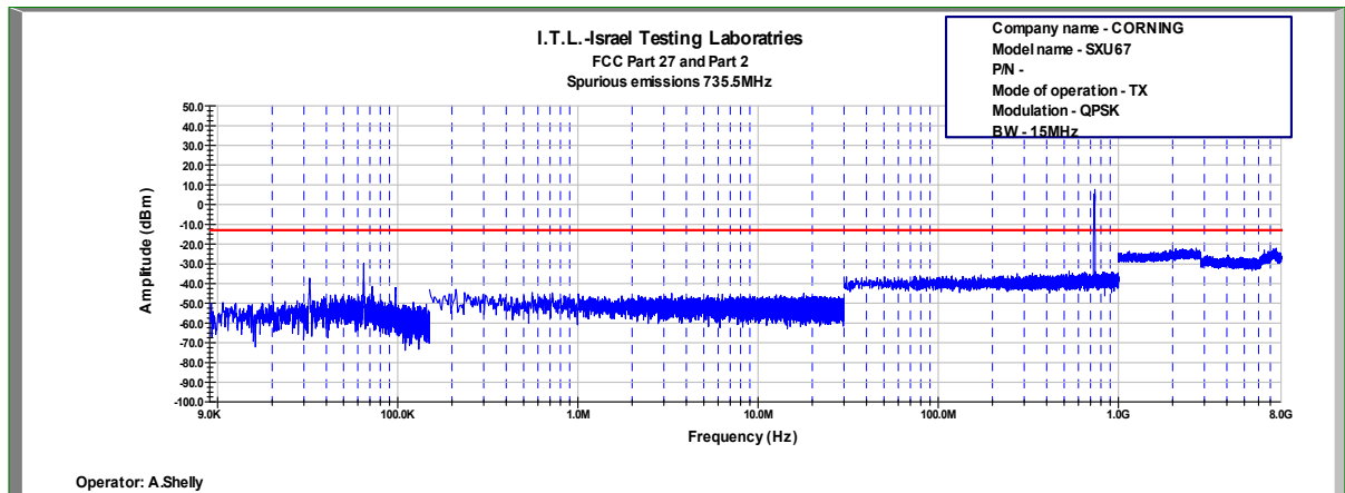
Figure 741: Spurious Emissions at Antenna Terminal QPSK, 735.5MHz, B.W. 15MHz, Sub Carrier 60kHz
