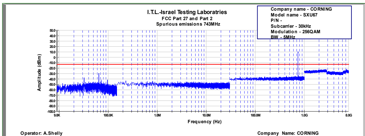
Figure 691: Spurious Emissions at Antenna Terminal 256QAM, 743.0MHz, B.W. 5MHz, Sub Carrier 30kHz
