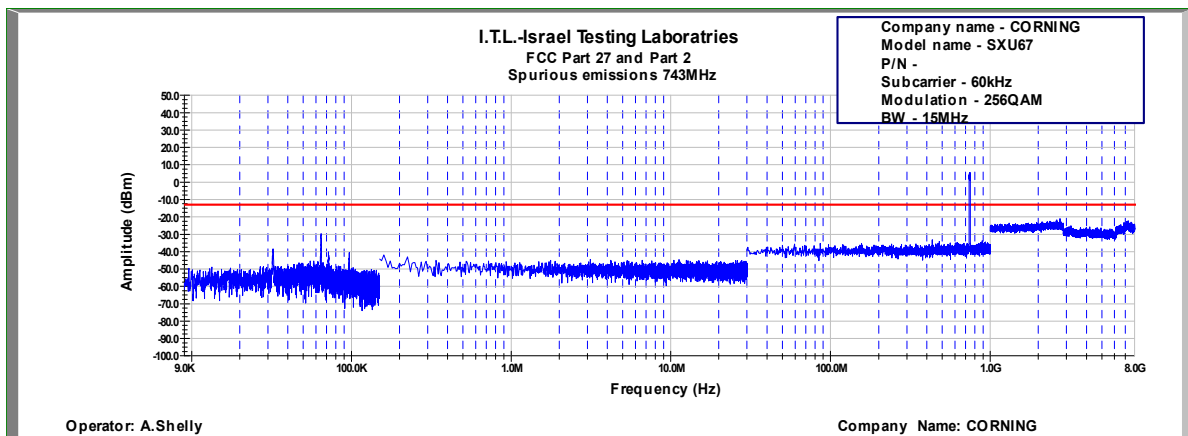
Figure 709: Spurious Emissions at Antenna Terminal 256QAM, 743.0MHz, B.W. 15MHz, Sub Carrier 60kHz
