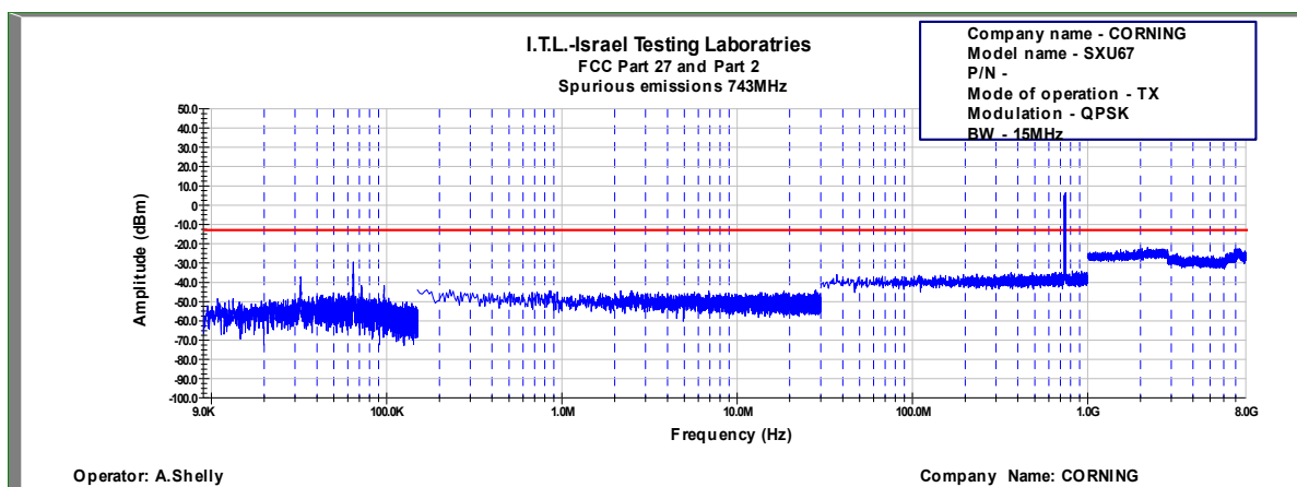
Figure 736: Spurious Emissions at Antenna Terminal QPSK, 743.0MHz, B.W. 15MHz, Sub Carrier 15kHz
