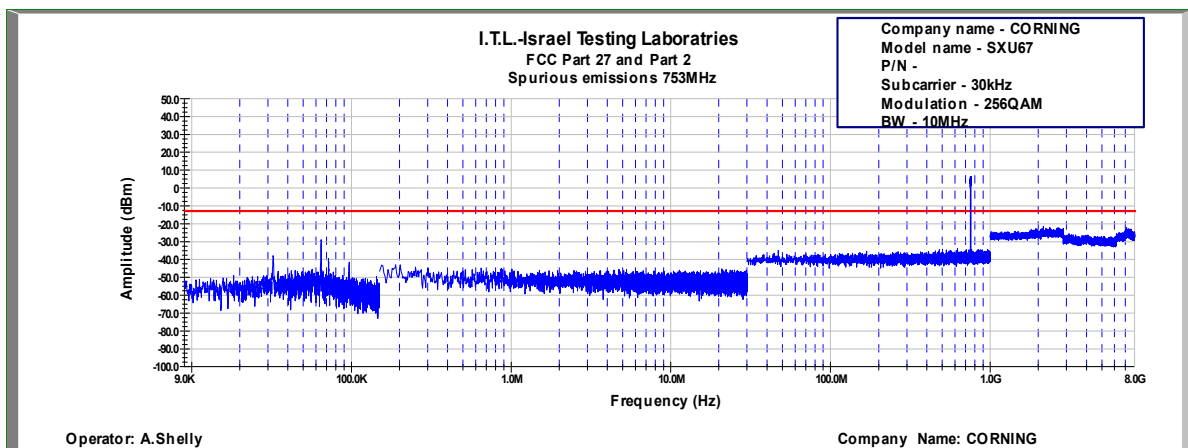
Figure 698: Spurious Emissions at Antenna Terminal 256QAM, 753.0MHz, B.W. 10MHz, Sub Carrier 30kHz
