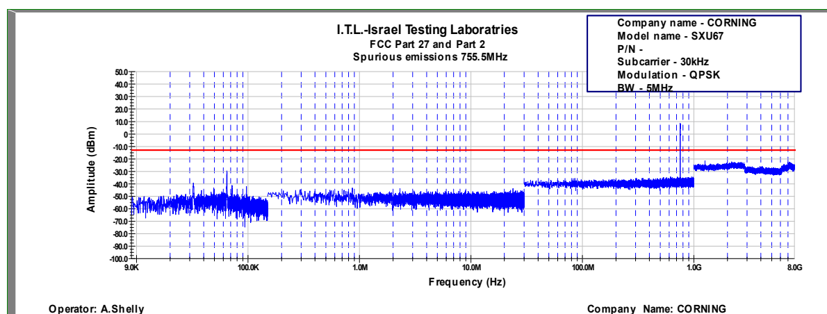
Figure 725: Spurious Emissions at Antenna Terminal QPSK, 755.5MHz, B.W. 5MHz, Sub Carrier 30kHz
