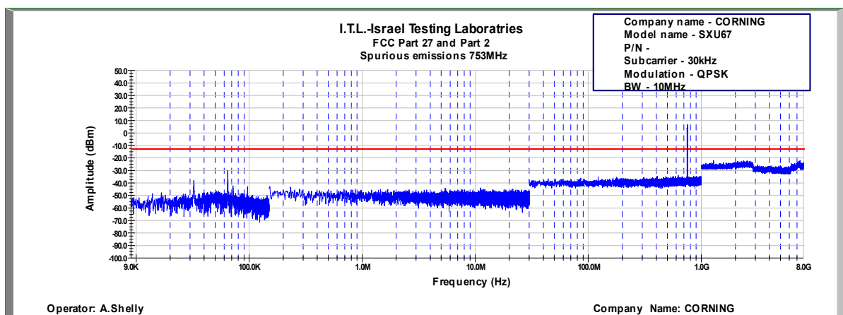
Figure 731: Spurious Emissions at Antenna Terminal QPSK, 753.0MHz, B.W. 10MHz, Sub Carrier 30kHz
