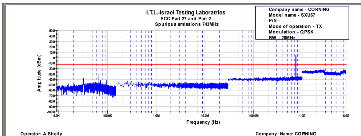
Figure 745: Spurious Emissions at Antenna Terminal QPSK, 743.0MHz, B.W. 20MHz, Sub Carrier 15kHz
