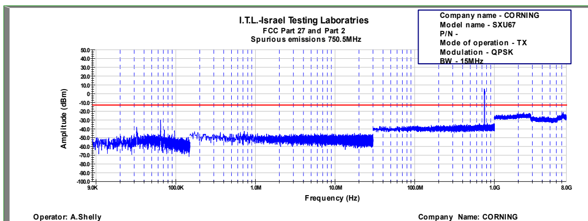
Figure 740: Spurious Emissions at Antenna Terminal QPSK, 750.5MHz, B.W. 15MHz, Sub Carrier 30kHz
