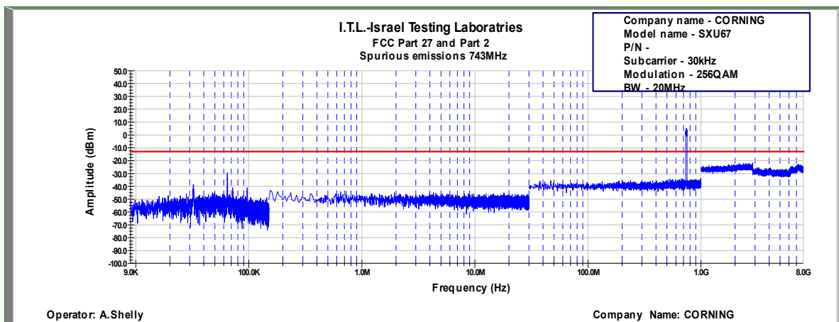
Figure 715: Spurious Emissions at Antenna Terminal 256QAM, 743.0MHz, B.W. 20MHz, Sub Carrier 30kHz
