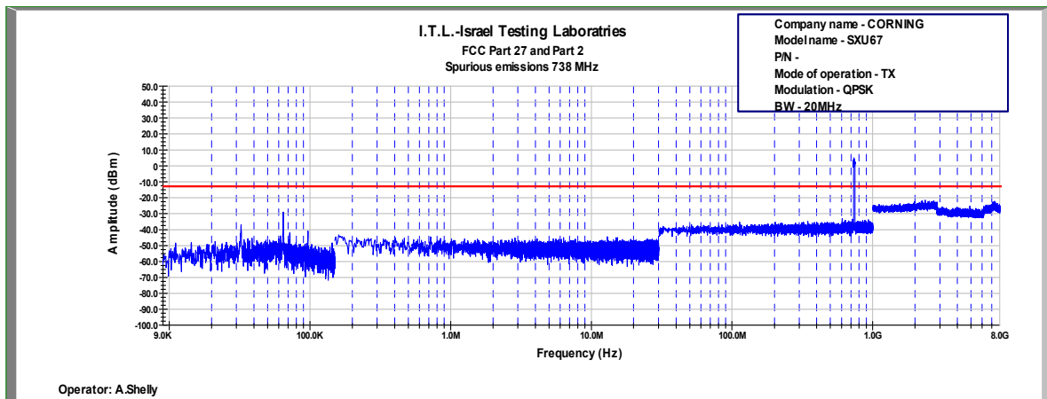
Figure 750: Spurious Emissions at Antenna Terminal QPSK, 738.0MHz, B.W. 20MHz, Sub Carrier 60kHz
