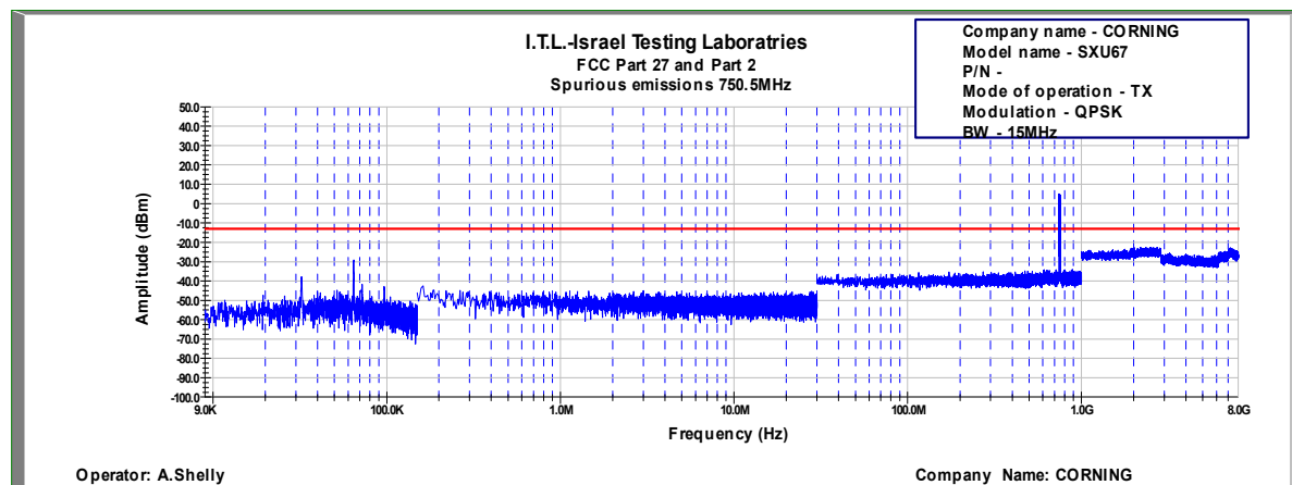
Figure 737: Spurious Emissions at Antenna Terminal QPSK, 750.5MHz, B.W. 15MHz, Sub Carrier 15kHz
