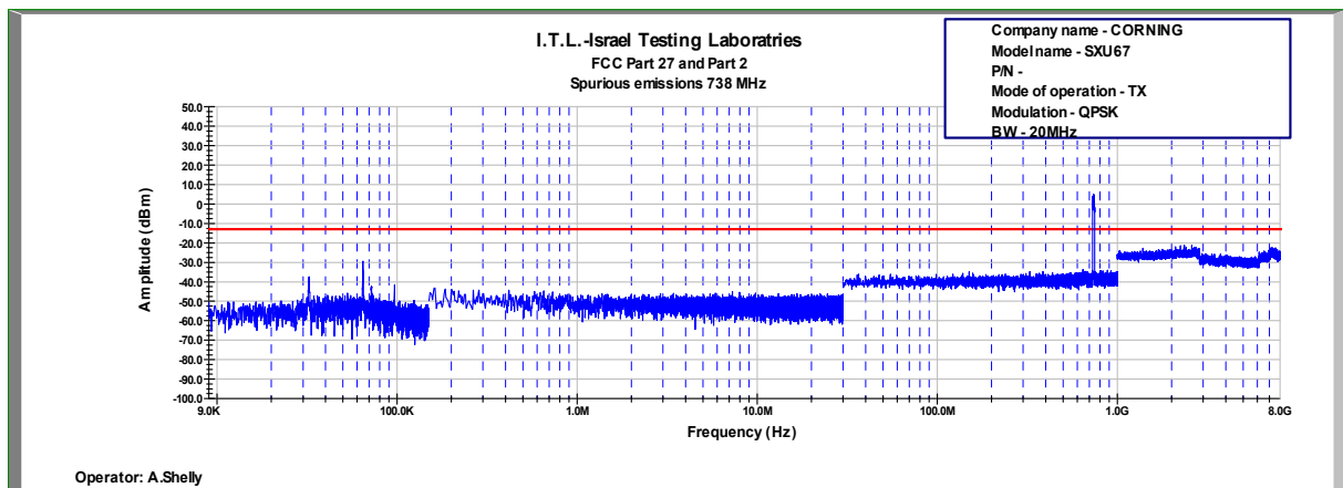
Figure 747: Spurious Emissions at Antenna Terminal QPSK, 738.0MHz, B.W. 20MHz, Sub Carrier 30kHz
