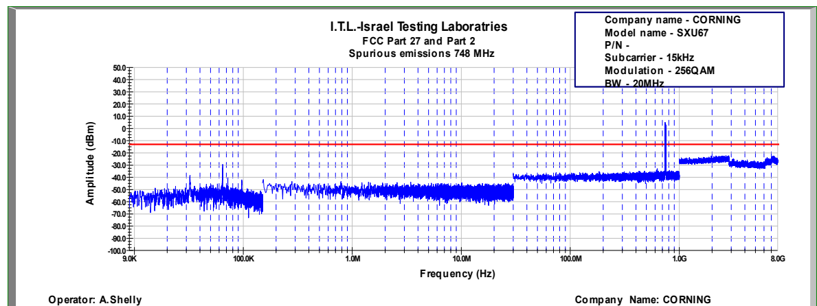
Figure 713: Spurious Emissions at Antenna Terminal 256QAM, 748.0MHz, B.W. 20MHz, Sub Carrier 15kHz
