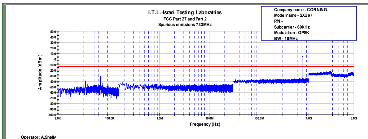
Figure 732: Spurious Emissions at Antenna Terminal QPSK, 733.0MHz, B.W. 10MHz, Sub Carrier 60kHz
