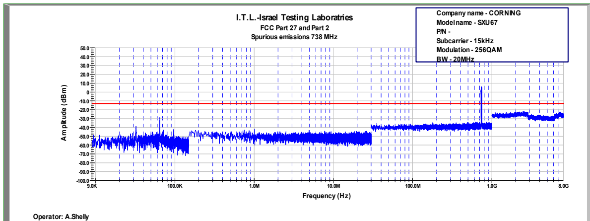
Figure 711: Spurious Emissions at Antenna Terminal 256QAM, 738.0MHz, B.W. 20MHz, Sub Carrier 15kHz
