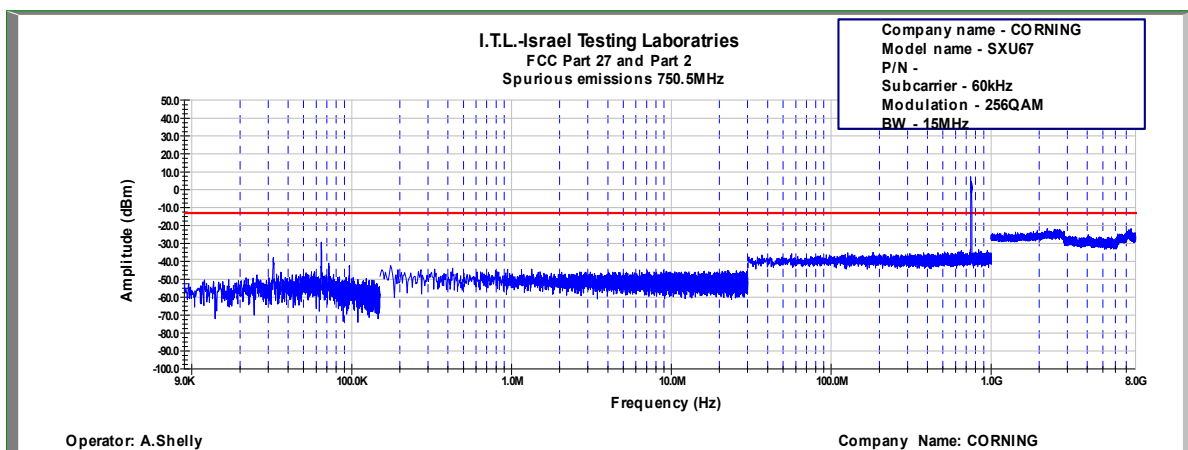
Figure 710: Spurious Emissions at Antenna Terminal 256QAM, 750.5MHz, B.W. 15MHz, Sub Carrier 60kHz
