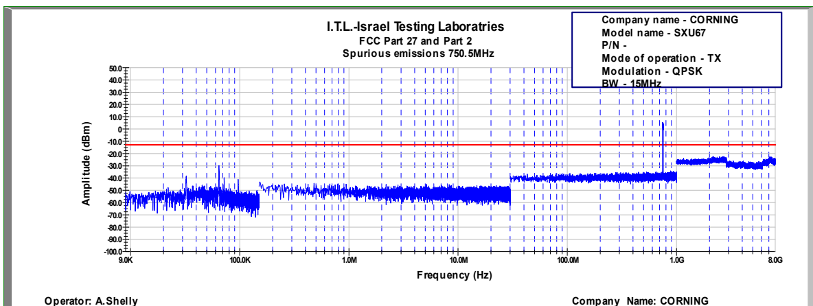
Figure 743: Spurious Emissions at Antenna Terminal QPSK, 750.5MHz, B.W. 15MHz, Sub Carrier 60kHz
