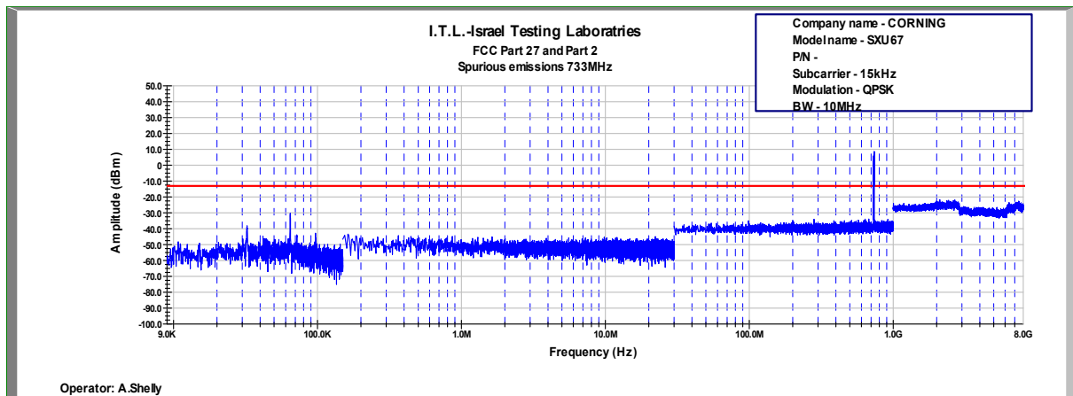
Figure 726: Spurious Emissions at Antenna Terminal QPSK, 733.0MHz, B.W. 10MHz, Sub Carrier 15kHz
