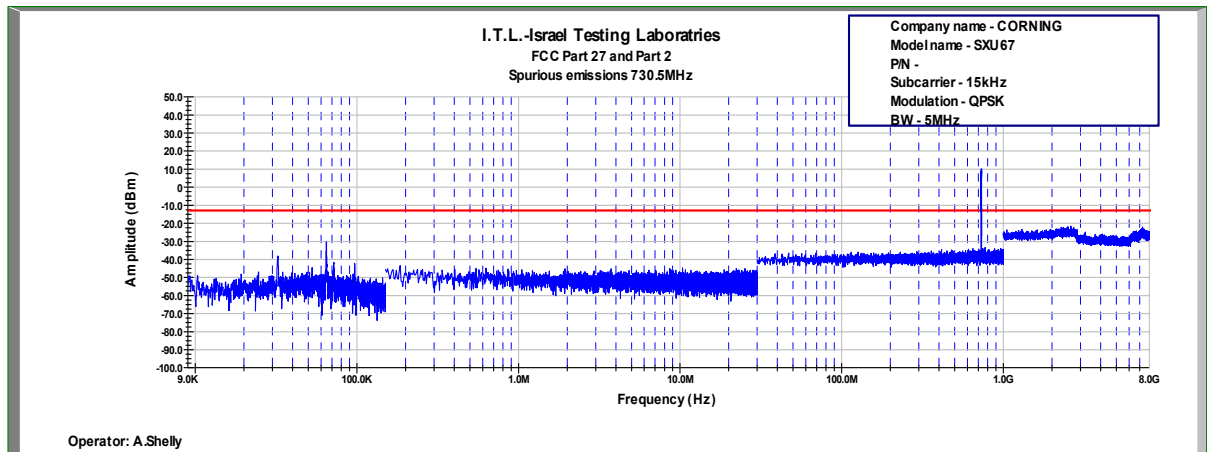
Figure 720: Spurious Emissions at Antenna Terminal QPSK, 730.5MHz, B.W. 5MHz, Sub Carrier 15kHz
