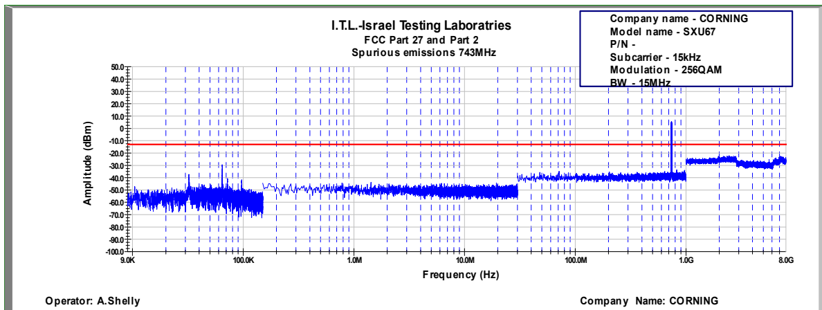
Figure 703: Spurious Emissions at Antenna Terminal 256QAM, 743.0MHz, B.W. 15MHz, Sub Carrier 15kHz
