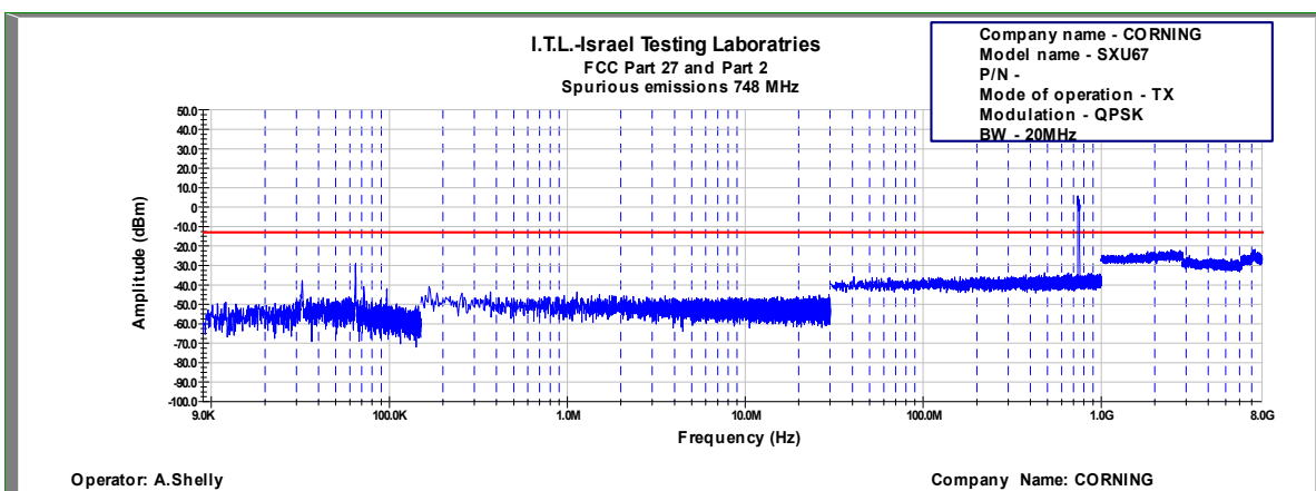
Figure 752: Spurious Emissions at Antenna Terminal QPSK, 748.0MHz, B.W. 20MHz, Sub Carrier 60kHz
