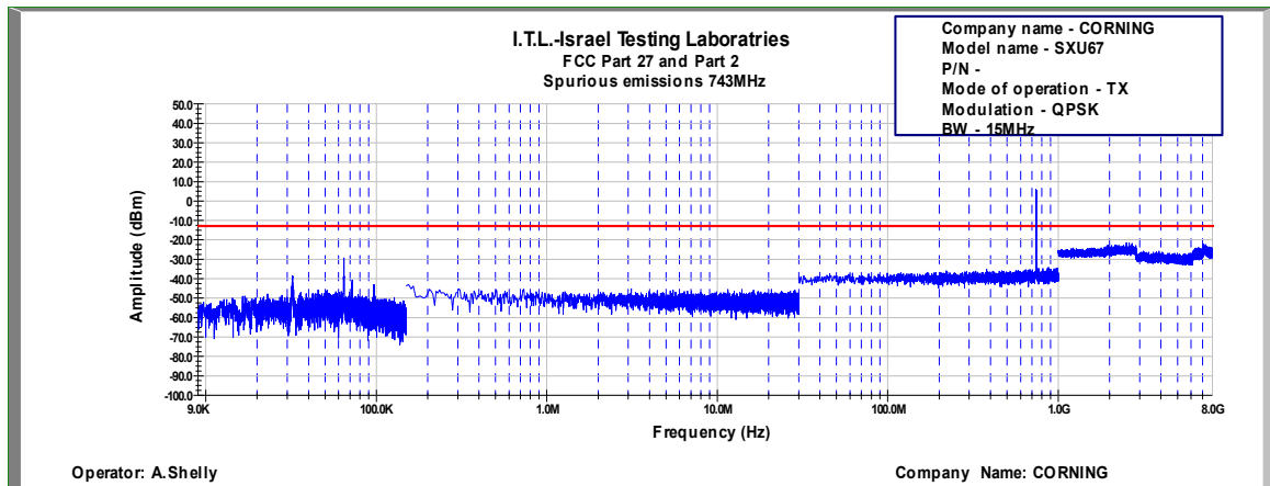
Figure 742: Spurious Emissions at Antenna Terminal QPSK, 743.0MHz, B.W. 15MHz, Sub Carrier 60kHz
