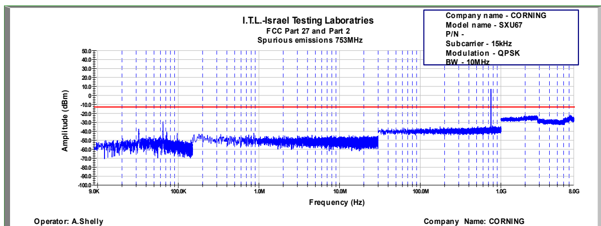
Figure 728: Spurious Emissions at Antenna Terminal QPSK, 753.0MHz, B.W. 10MHz, Sub Carrier 15kHz
