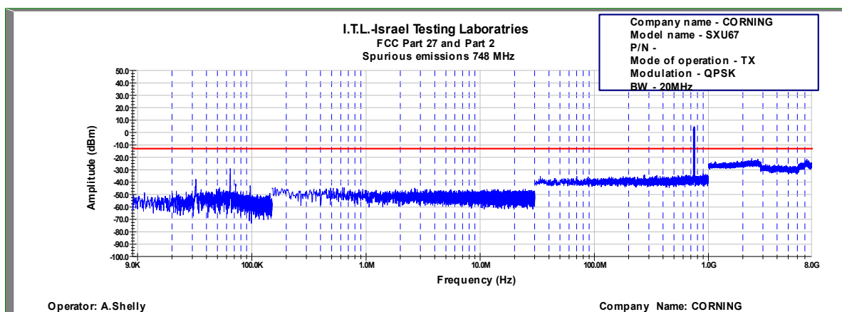
Figure 746: Spurious Emissions at Antenna Terminal QPSK, 748.0MHz, B.W. 20MHz, Sub Carrier 15kHz
