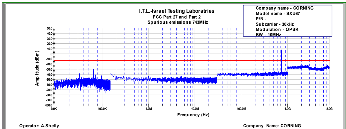
Figure 730: Spurious Emissions at Antenna Terminal QPSK, 743.0MHz, B.W. 10MHz, Sub Carrier 30kHz
