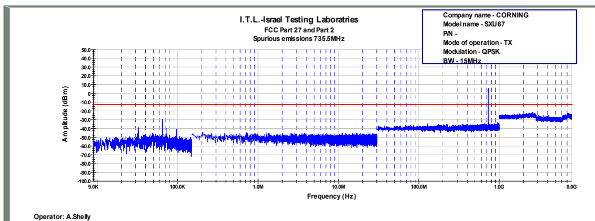
Figure 738: Spurious Emissions at Antenna Terminal QPSK, 735.5MHz, B.W. 15MHz, Sub Carrier 30kHz
