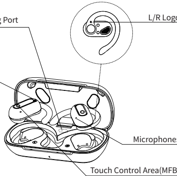
LED Indicator
