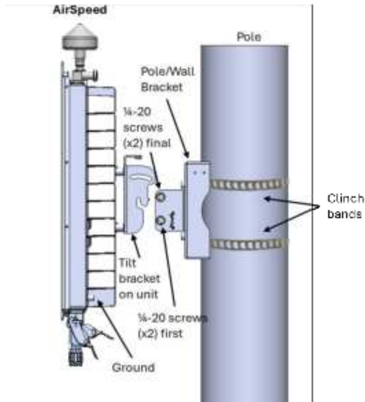
Figure 10: Pole Mounting - Maxi Clamps SS Bands
