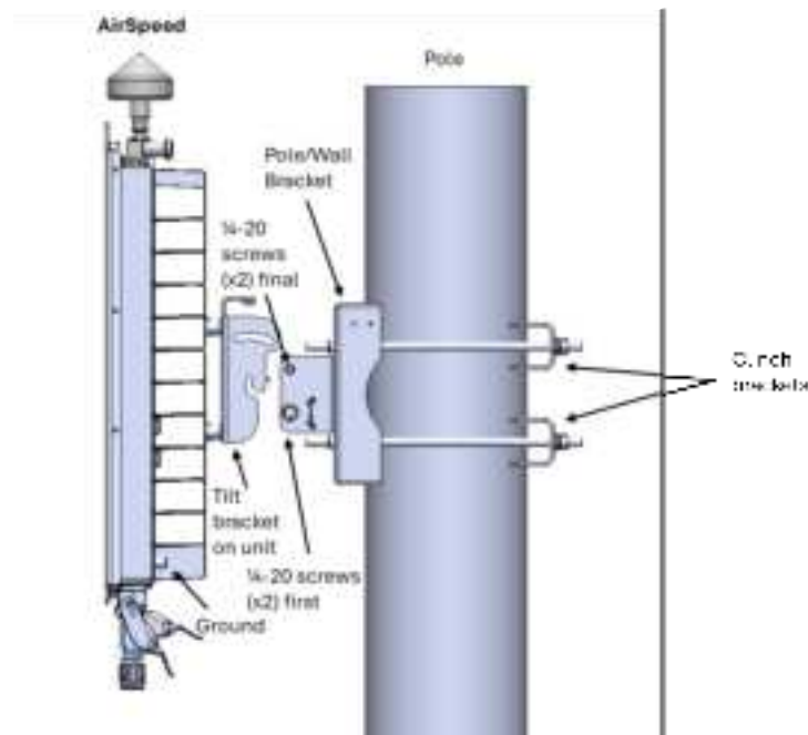
Figure 8: Pole Mounting Assembly
