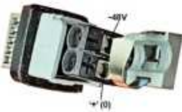
Figure 20: Power Wire Connection
