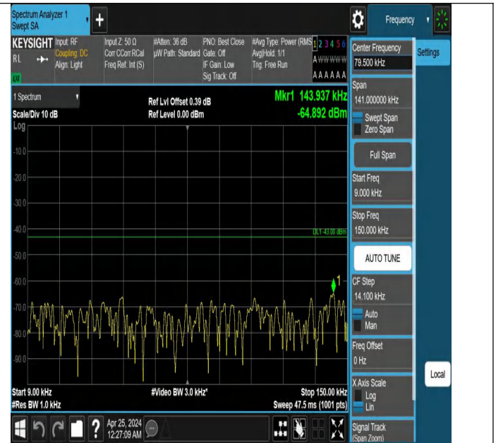
Band2_1.4MHz_QPSK_19193_1RB#5_0.009~0.15_0.009~0.15
