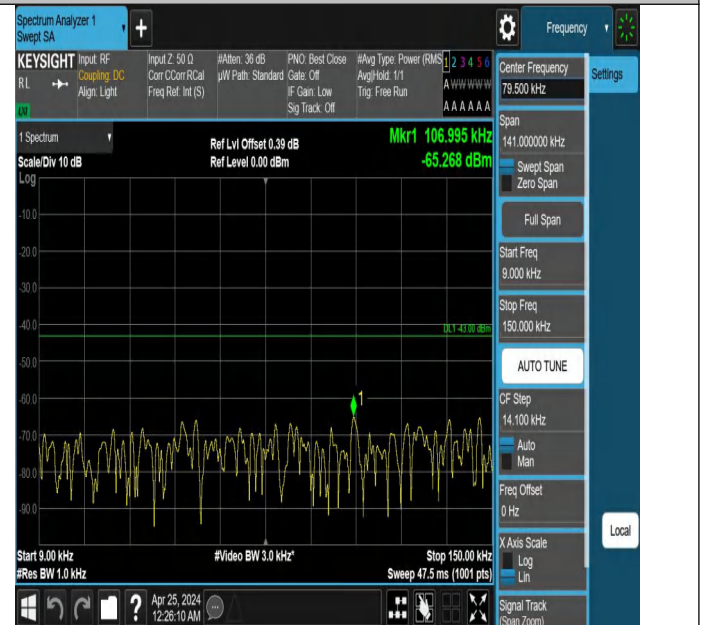
Band2_1.4MHz_QPSK_18900_1RB#5_0.009~0.15_0.009~0.15
