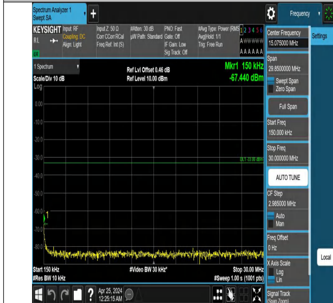
Band2_1.4MHz_QPSK_18607_1RB#5_0.15~30_0.15~30
