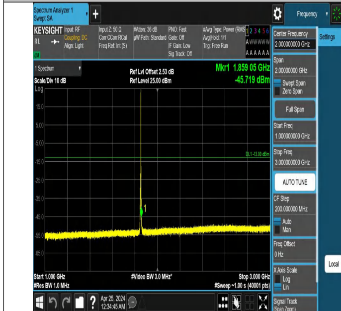
Band2_3MHz_QPSK_18615_1RB#14_1000~3000_1000~3000
