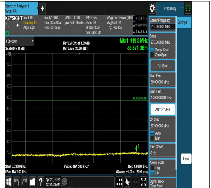
Band2_3MHz_QPSK_18615_1RB#14_30~1000_30~1000
