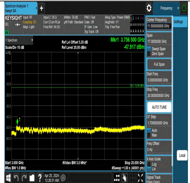
Band2_1.4MHz_QPSK_18900_1RB#5_3000~20000_3000~20000
