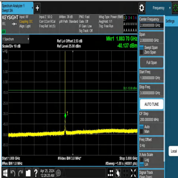
Band2_1.4MHz_QPSK_18900_1RB#5_1000~3000_1000~3000
