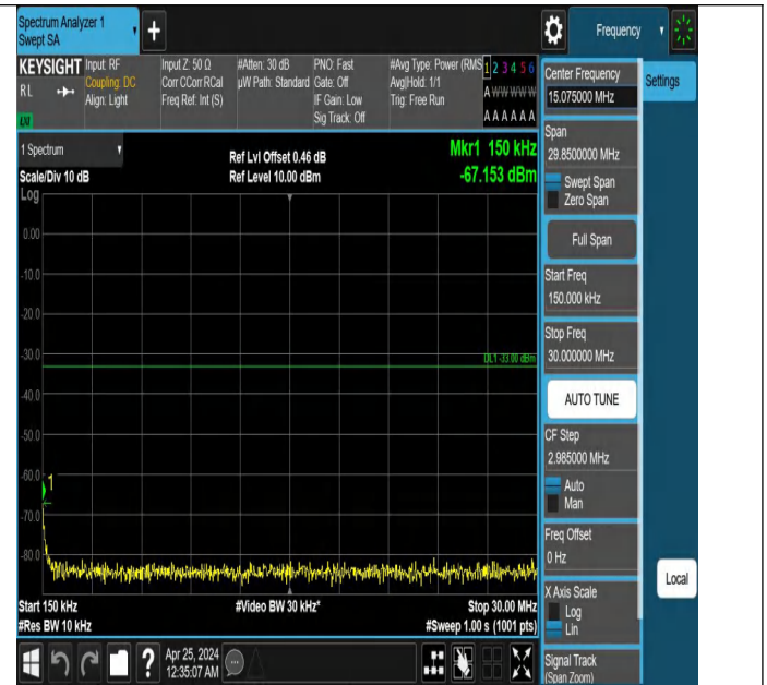
Band2_3MHz_QPSK_18900_1RB#0_0.15~30_0.15~30
