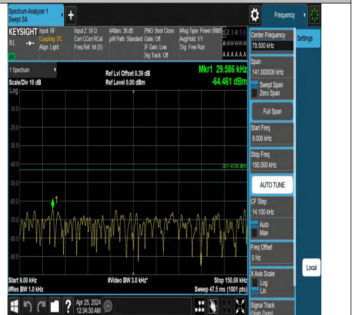
Band2_3MHz_QPSK_18615_1RB#14_0.009~0.15_0.009~0.15
