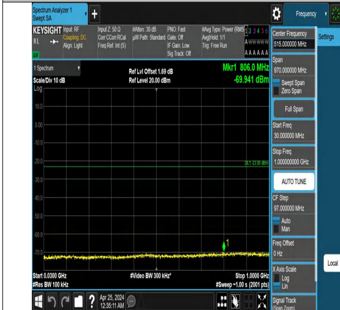
Band2_3MHz_QPSK_18900_1RB#0_30~1000_30~1000
