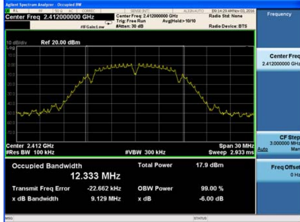
(802.11b) 6dB Bandwidth plot on channel 1
