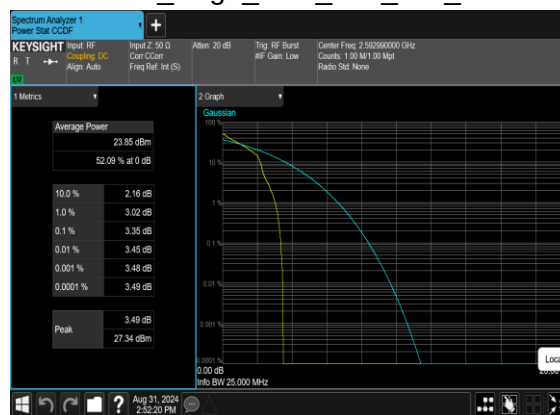
B66_N41(20M)_DFT-s-OFDM_PI_2-BPSK_Edge_1RB_Left_Mid_CH
