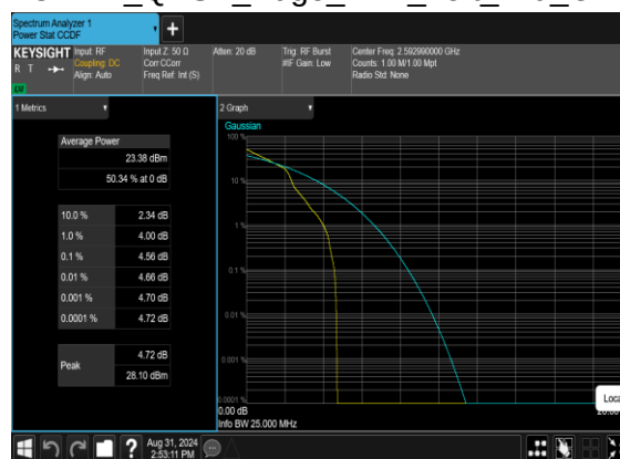
B66_N41(20M)_DFT-s-OFDM_QPSK_Edge_1RB_Left_Mid_CH
