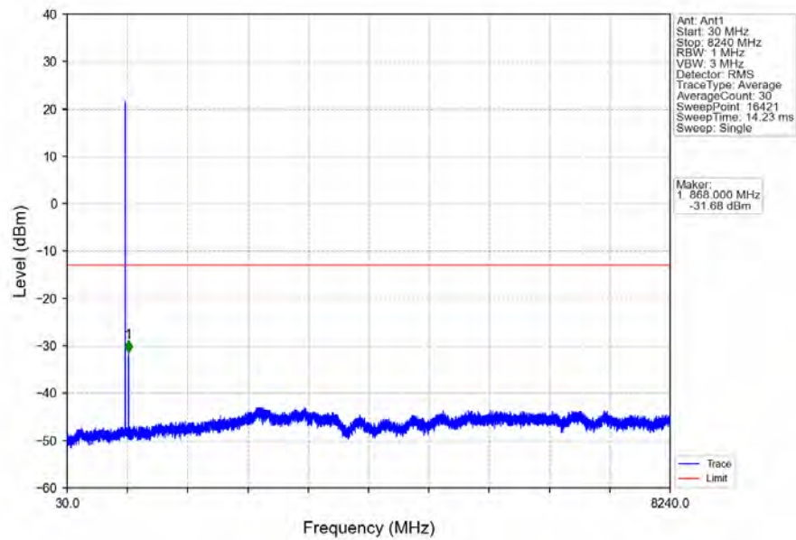
Band26a_3MHz_QPSK_HCH_822.5MHz_RB_1_14_NTNV
