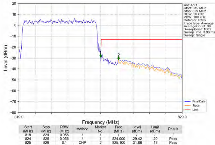
Band26a_5MHz_QPSK_HCH_821.5MHz_RB_25_0_NTNV
