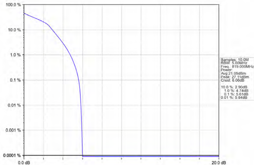
Band26a_3MHz_16QAM_MCH_819MHz_RB_15_0_NTNV
