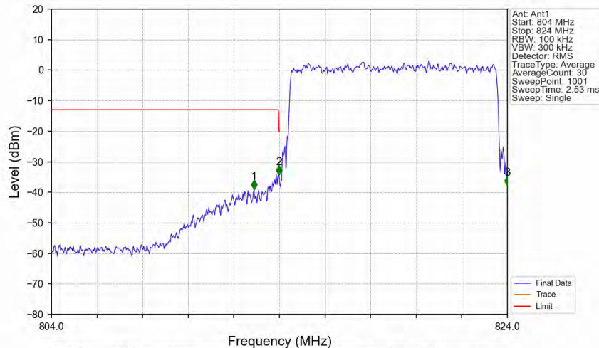
Band26a_10MHz_64QAM_LCH_819MHz_RB_50_0_NTNV
