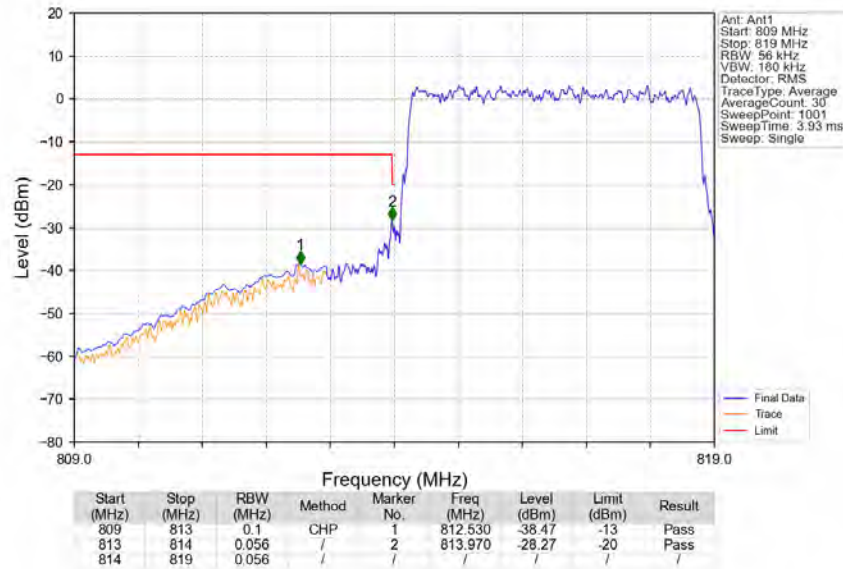
Band26a_5MHz_64QAM_LCH_816.5MHz_RB_25_0_NTNV
