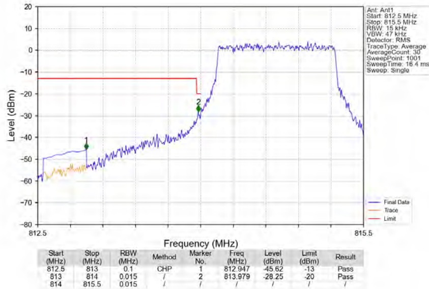
Band26a_1.4MHz_64QAM_LCH_814.7MHz_RB_6_0_NTNV
