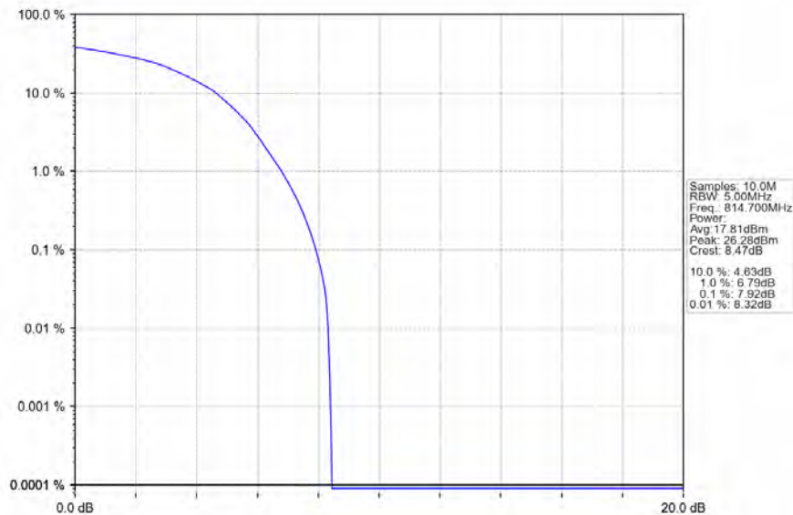
Band26a_1.4MHz_64QAM_LCH_814.7MHz_RB_6_0_NTNV
