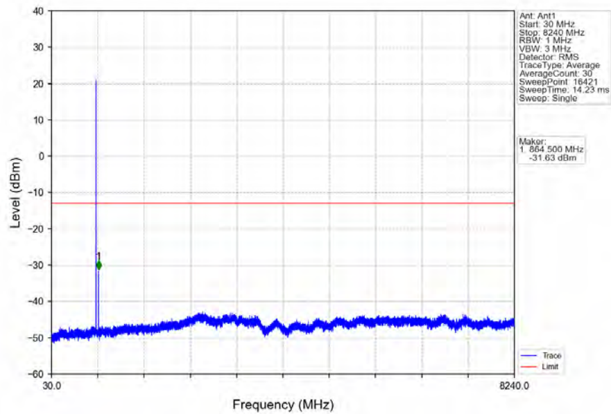
Band26a_3MHz_16QAM_HCH_822.5MHz_RB_1_0_NTNV
