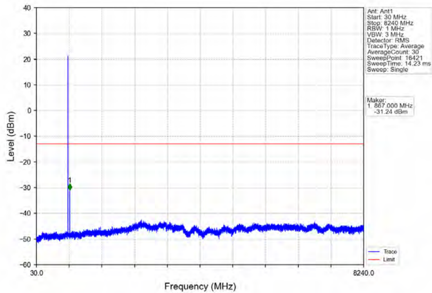
Band26a_5MHz_QPSK_HCH_821.5MHz_RB_1_24_NTNV
