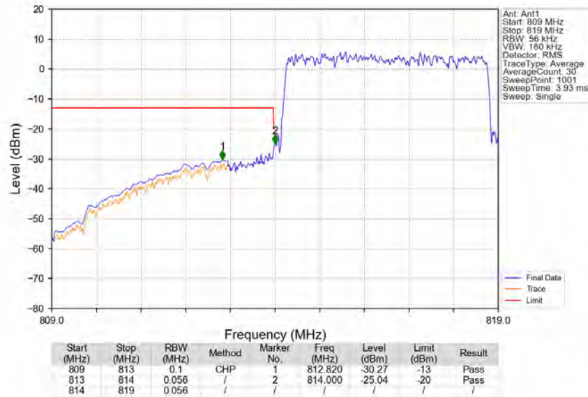
Band26a_5MHz_QPSK_LCH_816.5MHz_RB_25_0_NTNV
