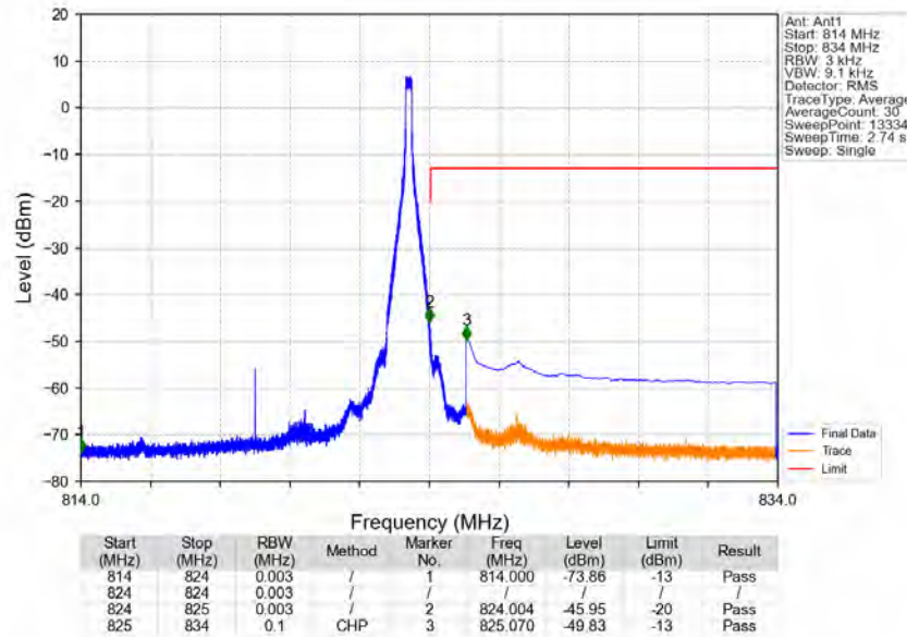
Band26a_10MHz_QPSK_HCH_819MHz_RB_50_0_NTNV
