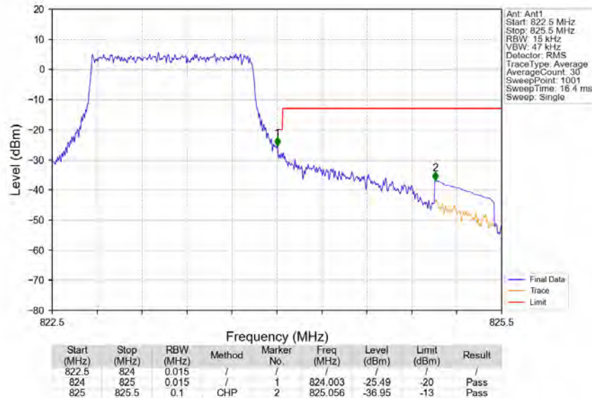
Band26a_1.4MHz_QPSK_HCH_823.3MHz_RB_6_0_NTNV
