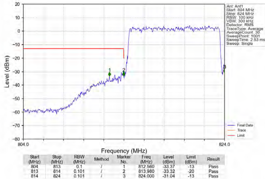
Band26a_10MHz_16QAM_LCH_819MHz_RB_50_0_NTNV
