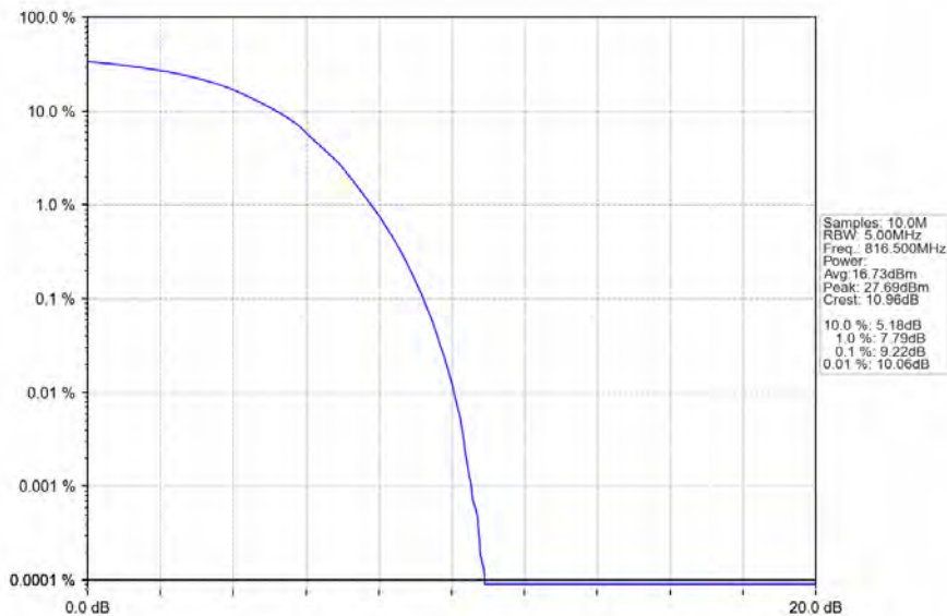
Band26a_5MHz_64QAM_LCH_816.5MHz_RB_25_0_NTNV
