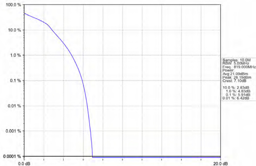
Band26a_5MHz_16QAM_MCH_819MHz_RB_25_0_NTNV
