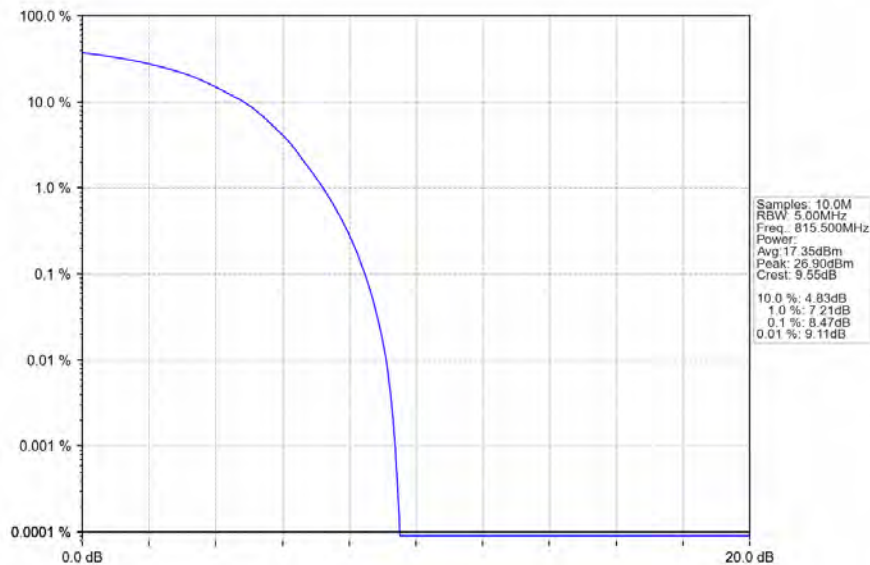
Band26a_3MHz_64QAM_LCH_815.5MHz_RB_15_0_NTNV
