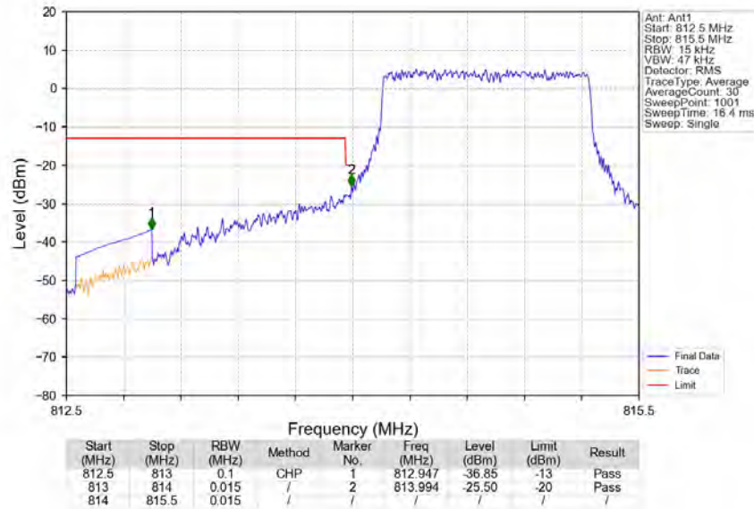
Band26a_1.4MHz_QPSK_LCH_814.7MHz_RB_6_0_NTNV
